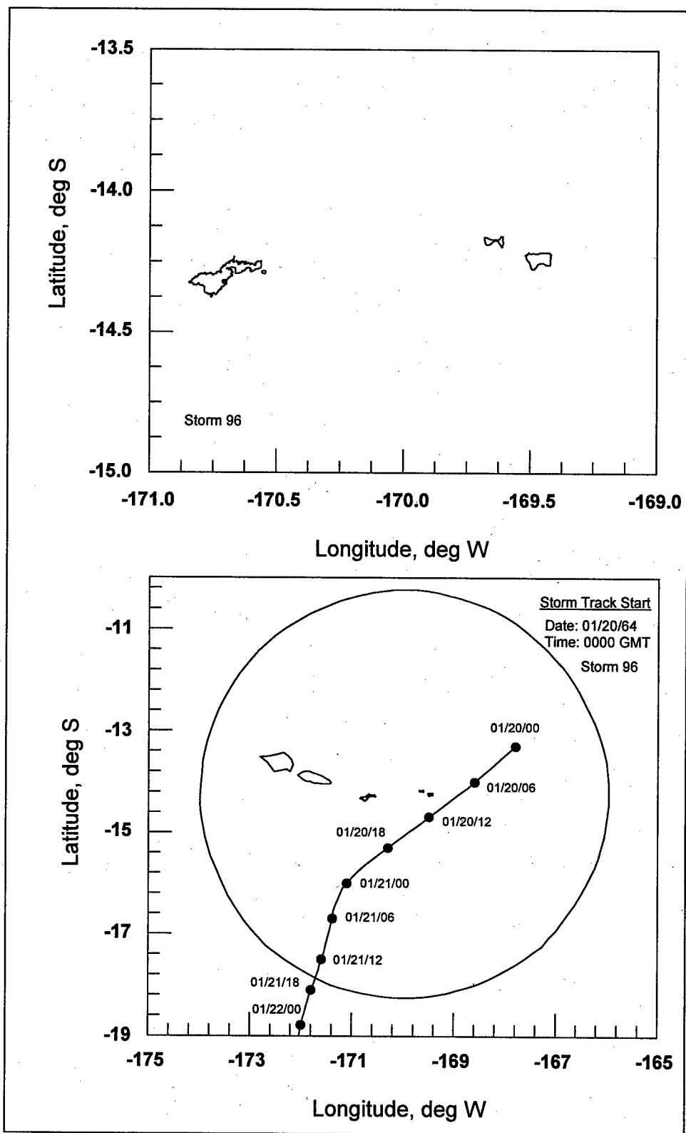
Figure E.10. Storm track for storm number 96
