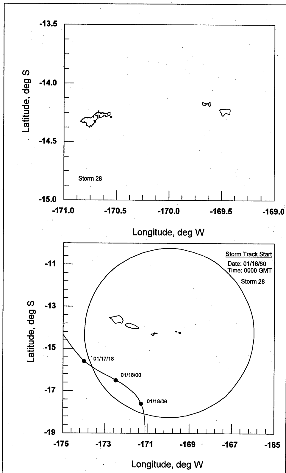
Figure E.4 Storm track for storm number 28
