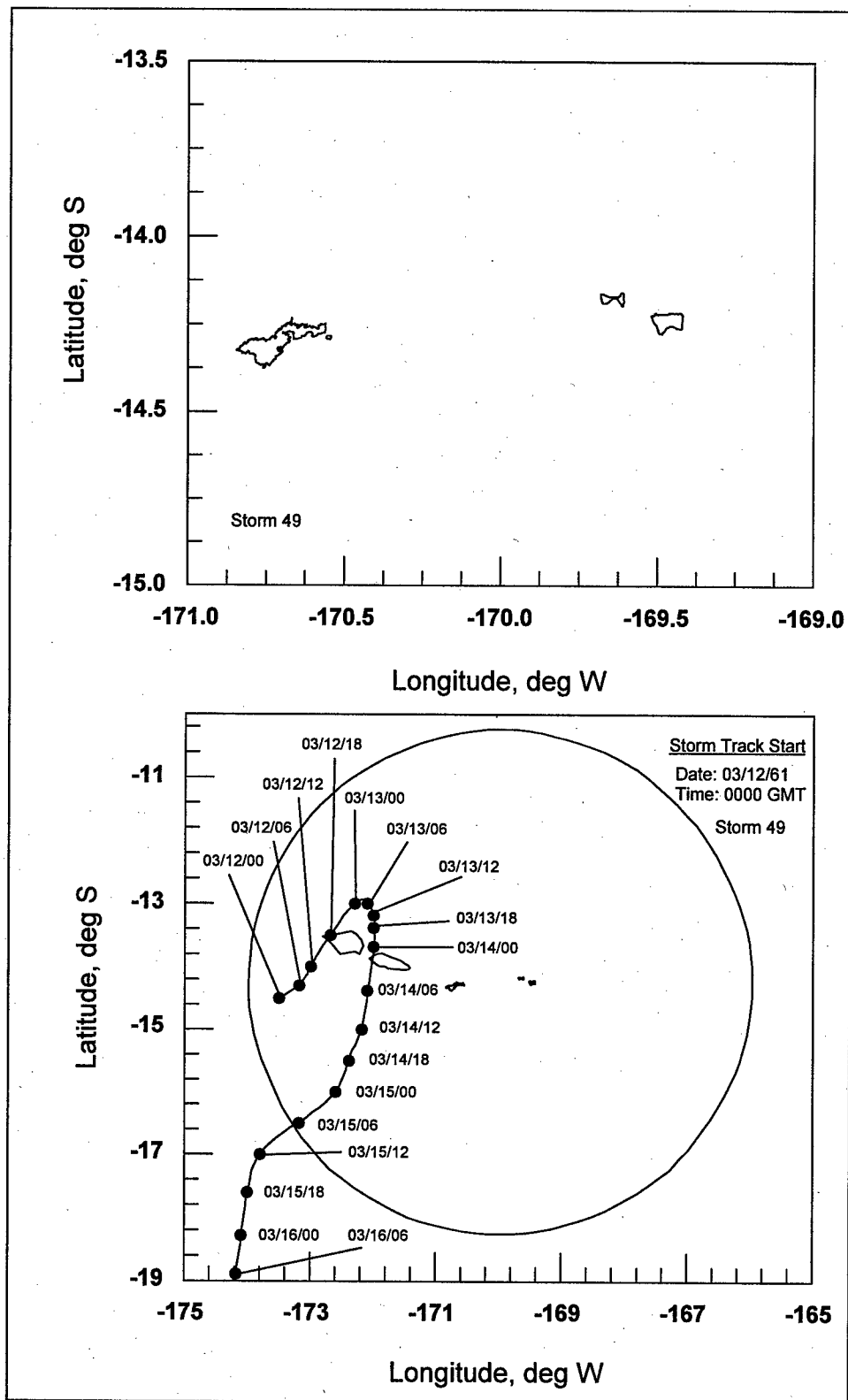
Figure E.6 Storm track for storm number 49
