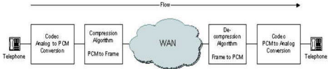
Figure 9. Voice Flow (From: Ref 11)
