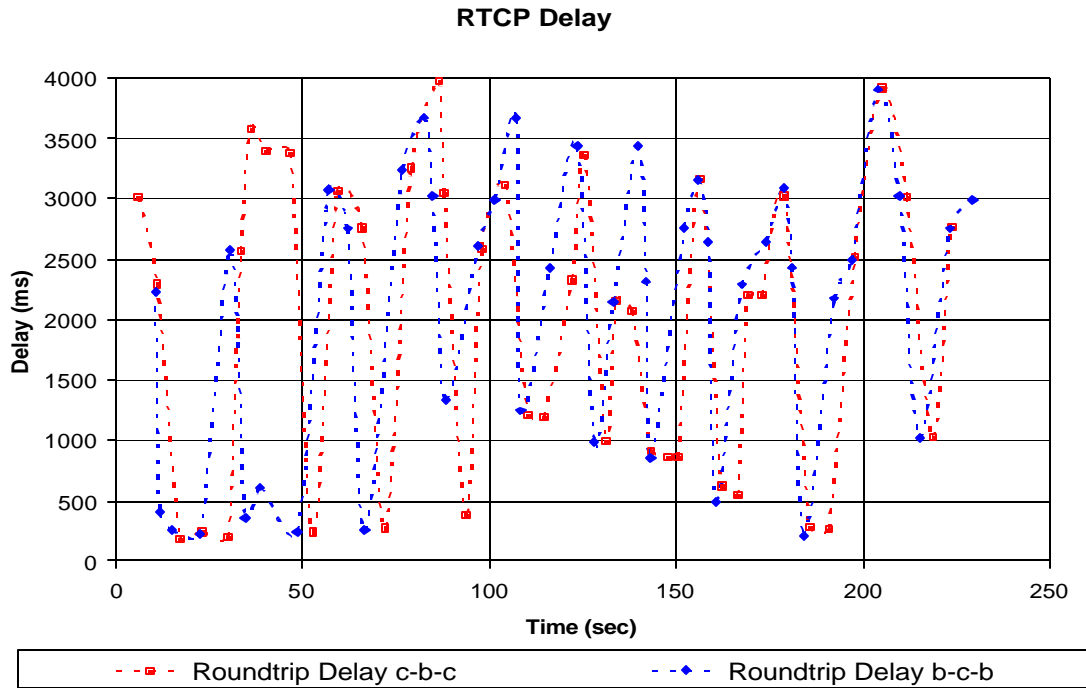
Figure 59. RTCP Consistency
