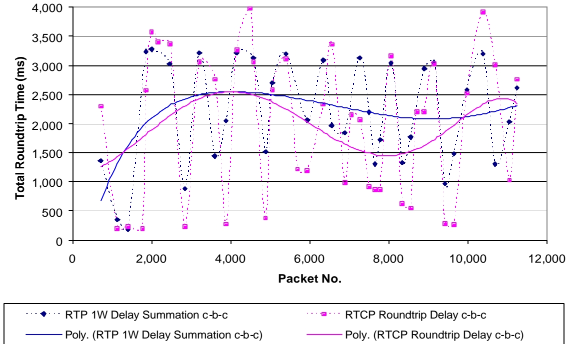
Figure 60. RTCP Accuracy
