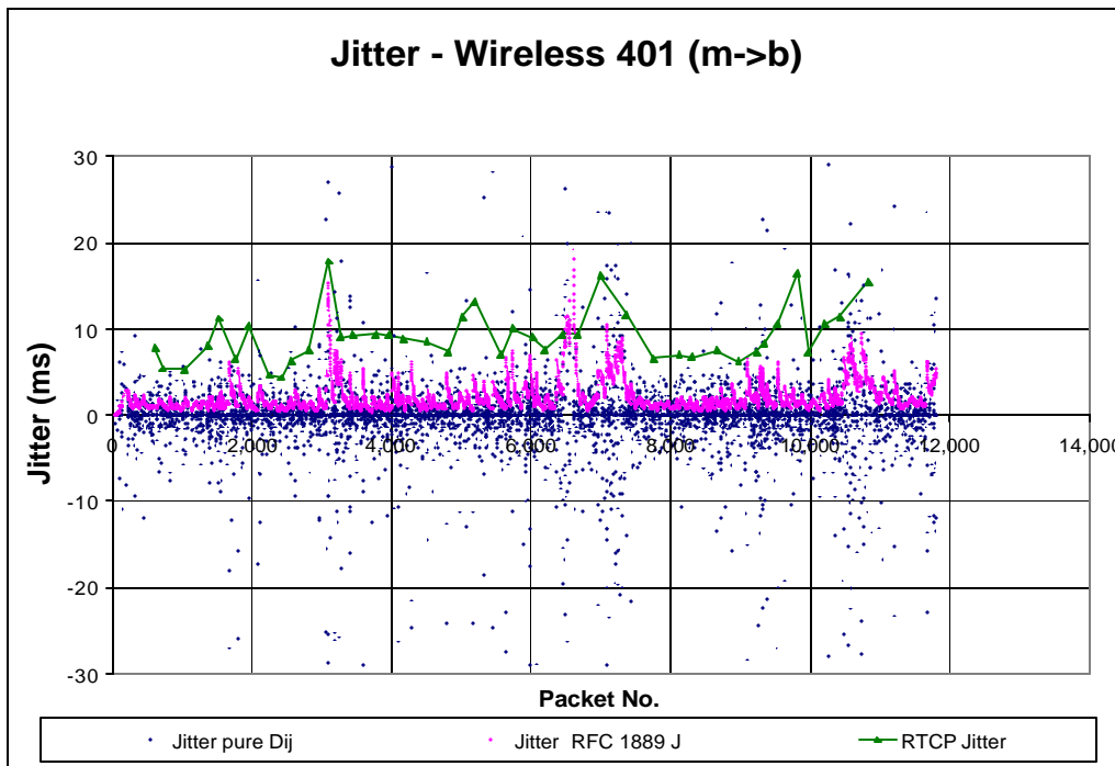
Figure 58. Wireless Test Result (2)
