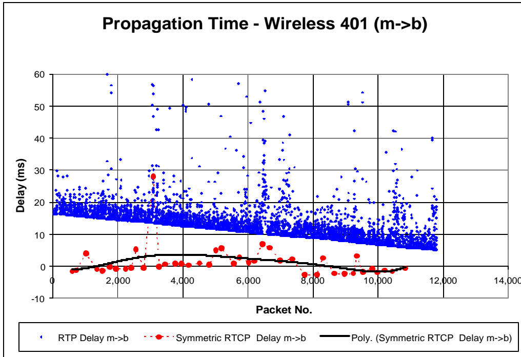
Figure 57. Wireless Test Result (1)
