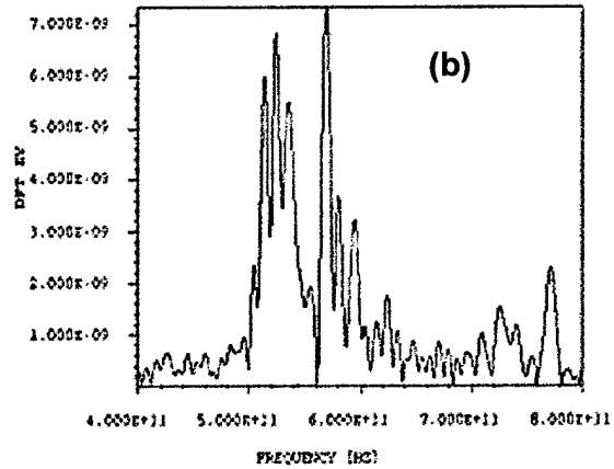
Figure 10 Simulated y-component of electric field at position p1 of Figure 9.
