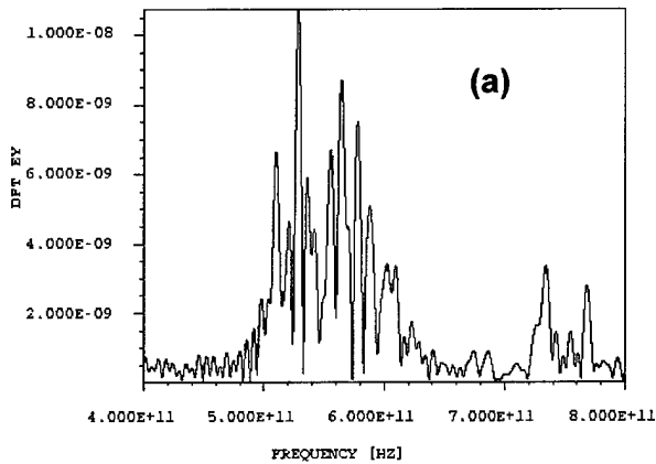
Figure 10 Simulated y-component of electric field at position p1 of Figure 9.
