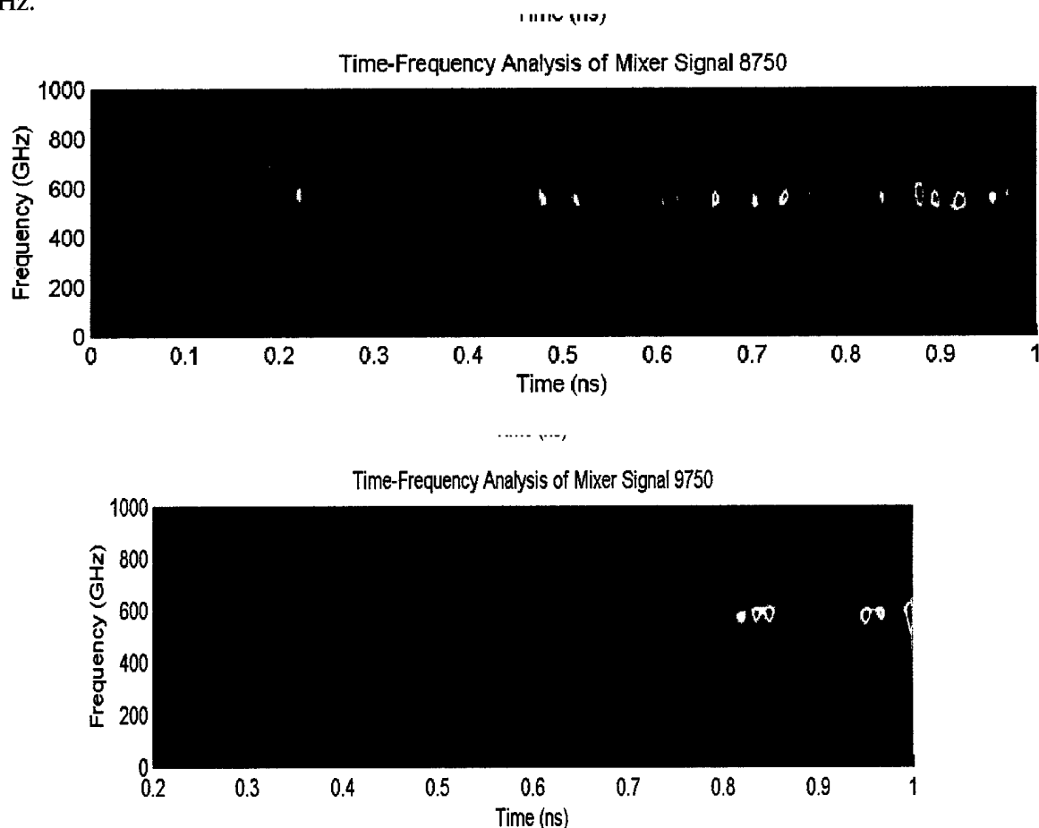
Figure 12 Time frequency analysis. (a) Intermediate feedback ( -8.75 dB return loss) (b) Critical feedback ( -9.75 dB return loss).
