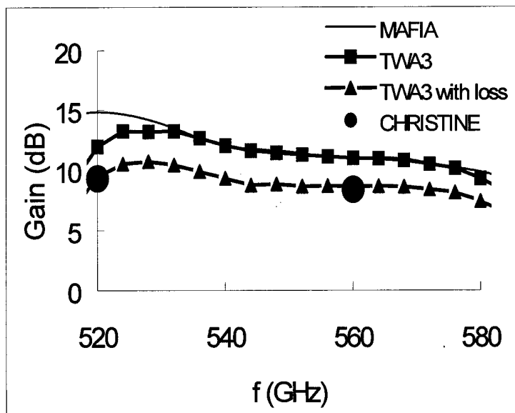
Figure 6 Small signal single pass gain for a 6.6 mm long FWG-TWT designed to operate at \sim 560 GHz. The simulation assumes a 10.9 kV, 0.5 mA electron beam.
