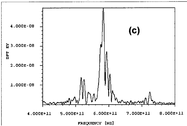
Figure 11 Simulations showing frequency selection for the 560 GHz oscillator. (a) 0 dB loss. Overdriven feedback having multi frequency oscillation states. (b) - 8.75 dB loss. Intermediate feedback, showing two preferred frequency states and (c) - 9.75 dB loss. Critical feedback showing approach to a single frequency state.
