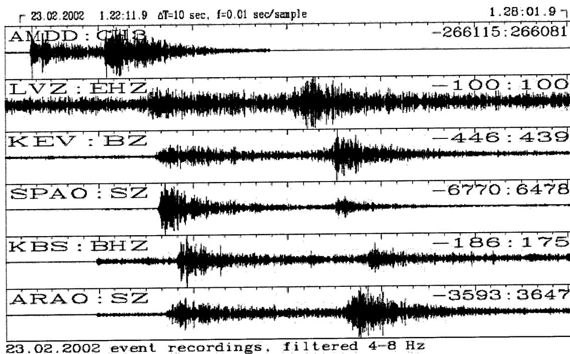
Fig. 6.2.3. Recorded SPZ waveforms for the 23.02.2002 seismic event. The data are filtered in the 4-8 Hz band. Note the high P-phase SNR in particular at the Spitsbergen array (sensor SPA0) and the Amderma station (AMDD). Note also the relatively weak S-phase for the two stations at Spitsbergen (SPA0 and KBS).
