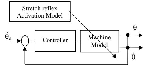
Fig.5. Stretch reflex and Multi-Iso control model
