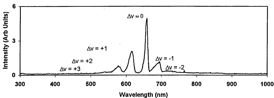
Figure 3. Spectrum of visible emission resulting from the photolysis of \text{NCl}_3 at 193 nm. Sequences of the \text{NCl } b \rightarrow X transition are labeled.
