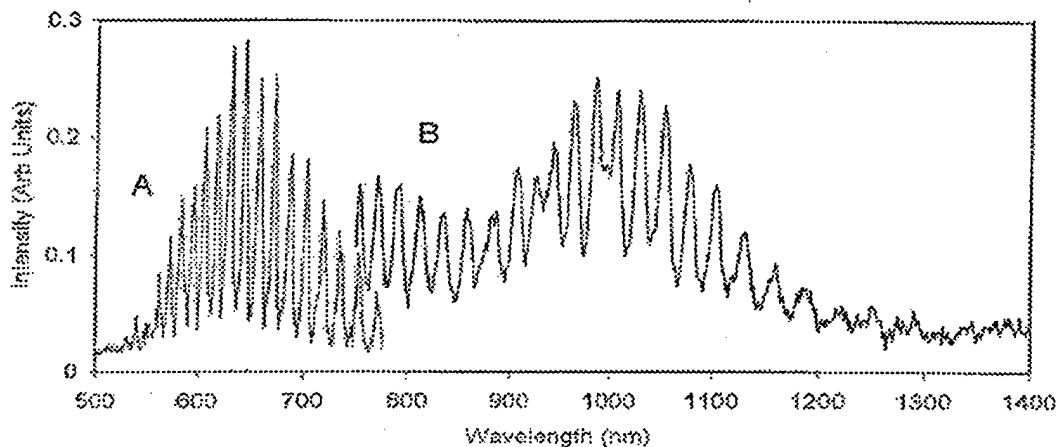
Figure 1. Spectrum of visible and near IR emission produced from the 249 nm photolysis of \text{NCl}_3 , gated from 0 to 50 \mu\text{s} . (A) data from Gilbert, et. al. (ref. 16); (B) present data.
