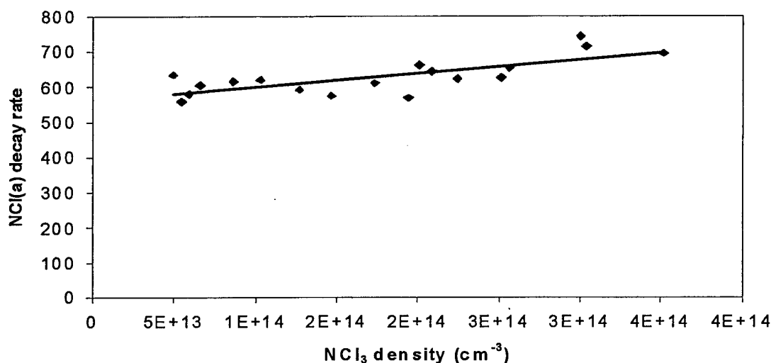
Figure 6. A plot of the exponential decay rate of emission from NCl(a) vs. the initial density of NCl 3 . The linear least-squares fit to the slope gives a rate constant k = (3.4 \pm 1.7) \times 10^{-13} \text{ cm}^3 \text{ s}^{-1} .
