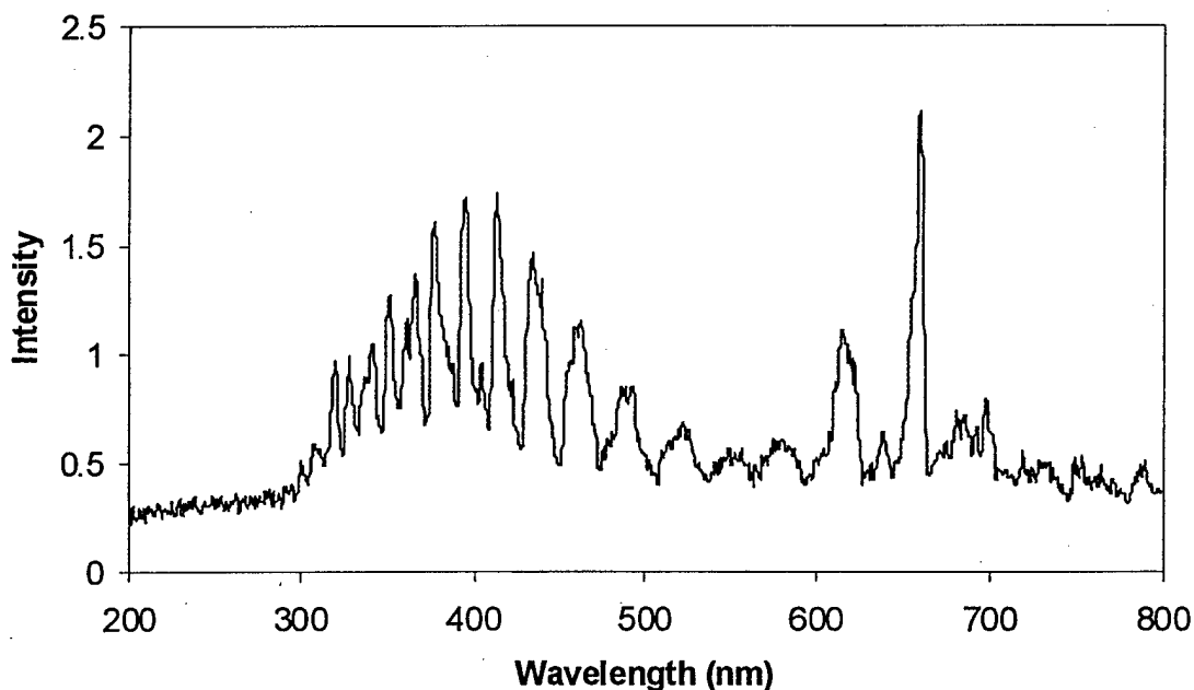
Figure 10. Spectrum of emission from excited \text{NS}^* produced by 193 nm photolysis of \text{NCl}_3/\text{H}_2\text{S}/\text{Ar} mixtures. The intense features between 600 and 700 nm correspond to emission from \text{NCl}(b^1\Sigma^+) , as in Figure 2 above.
