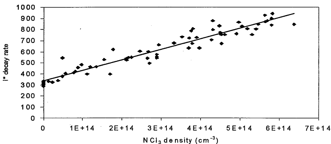
Figure 7. A plot of the exponential decay rate of emission from I*(5 2 P 1/2 ) vs. the density of NCl 3 . A linear least-squares fit to the slope gives a rate constant k = (9.5 \pm 2.0) \times 10^{-13} \text{ cm}^3 \text{ s}^{-1} .
