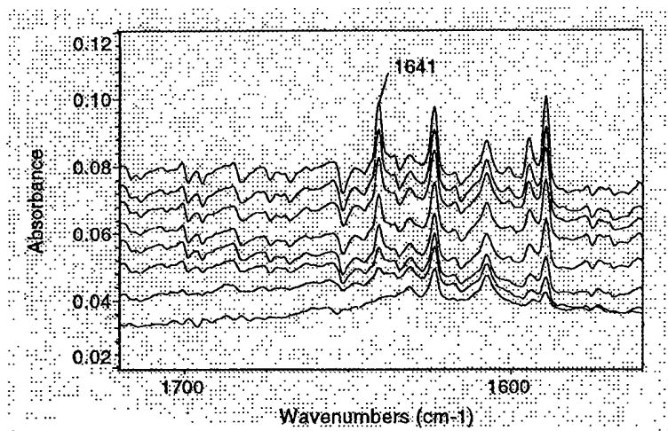
Figure 13. IR spectra of the 1600-1700 \text{cm}^{-1} region, from a sample of \text{B}(\text{N}_3)_3 dissociated in a discharge through Ar. The bottom spectrum was taken earliest, the top spectrum latest
