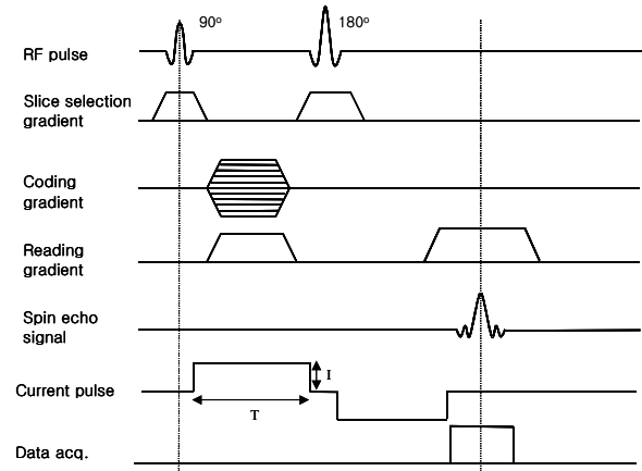
Fig. 2. The current injection MRI pulse sequence
