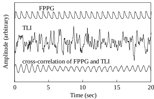
Fig.2 Typical example of transmitted light intensity (TLI), finger photoplethysmogram (FPPG) and their cross-correlation.
