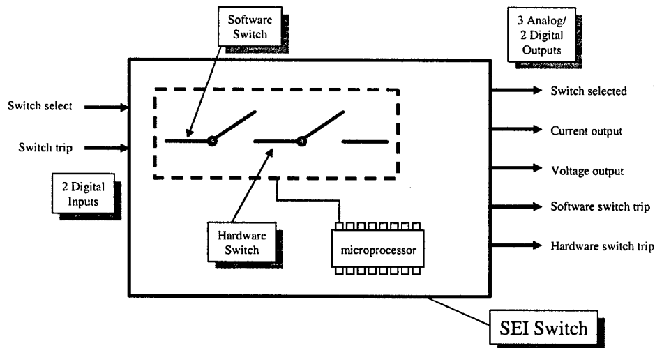
Figure 3: SEI Switch Abstraction
