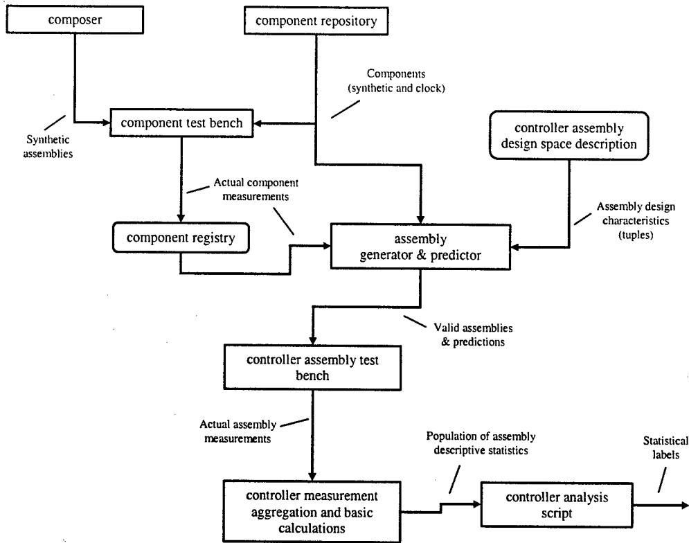
Figure 53: Measurement Infrastructure Tool Workflow
