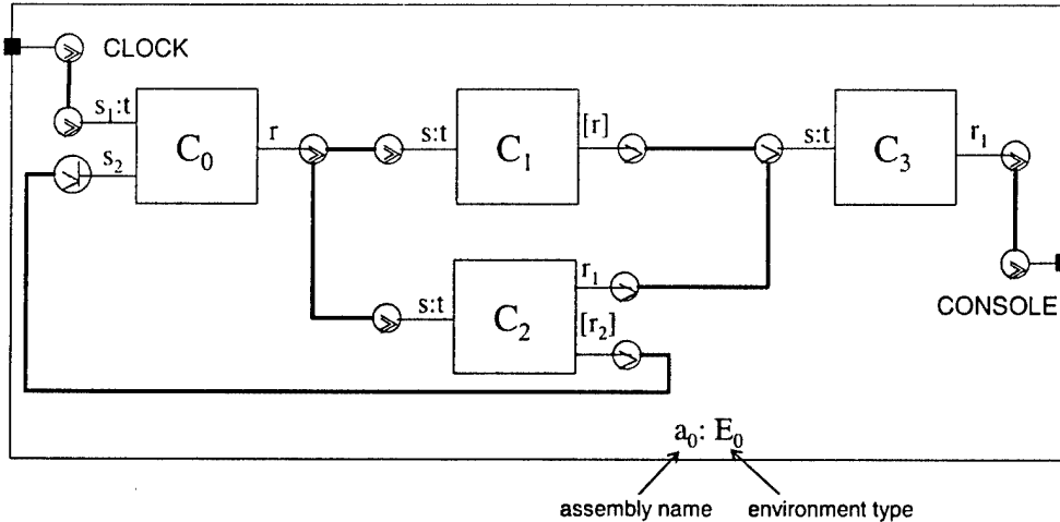
Figure 7: A Simple Assembly
