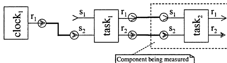
Figure 48: General Assembly Topology for Benchmarking Synthetic
