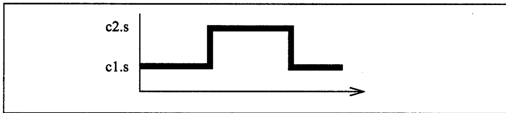
Figure 30: Timeline for a Sink Pin with Interactions in the Middle of Its Execution
