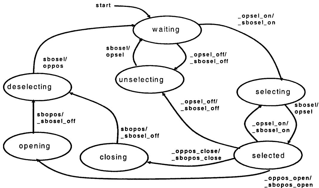
Figure 18: CSWI State Machine
