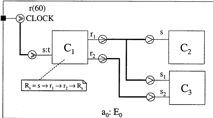
Figure 32: Constructive Assembly with Tree-Like Topology
