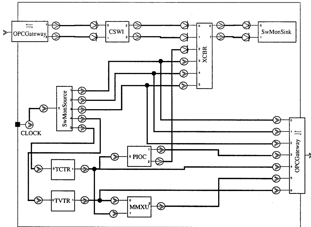
Figure 9: SAS Software Controller in Pin 16
