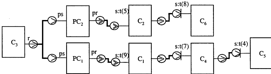
Figure 36: Multiple Asynchronous Connections Rewrite
