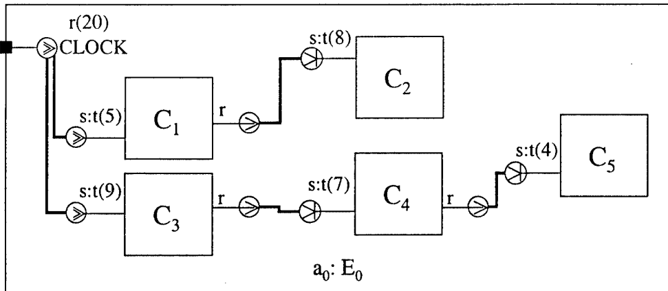
Figure 33: Constructive Assembly with Asynchronous Connections
