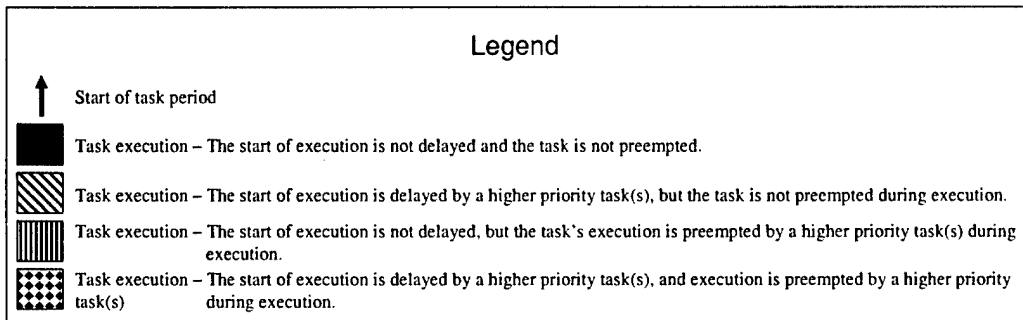
Figure 22: Task Phasing and Hyper-Period
