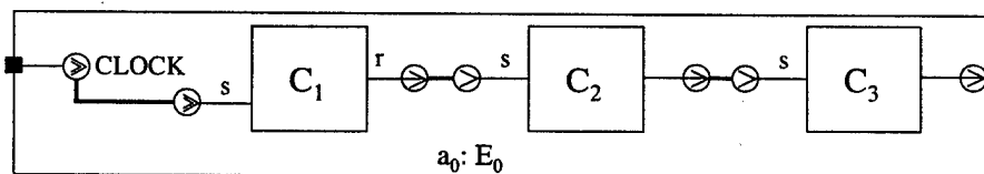
Figure 14: Clock Component Initiating a Sequence of Interactions
