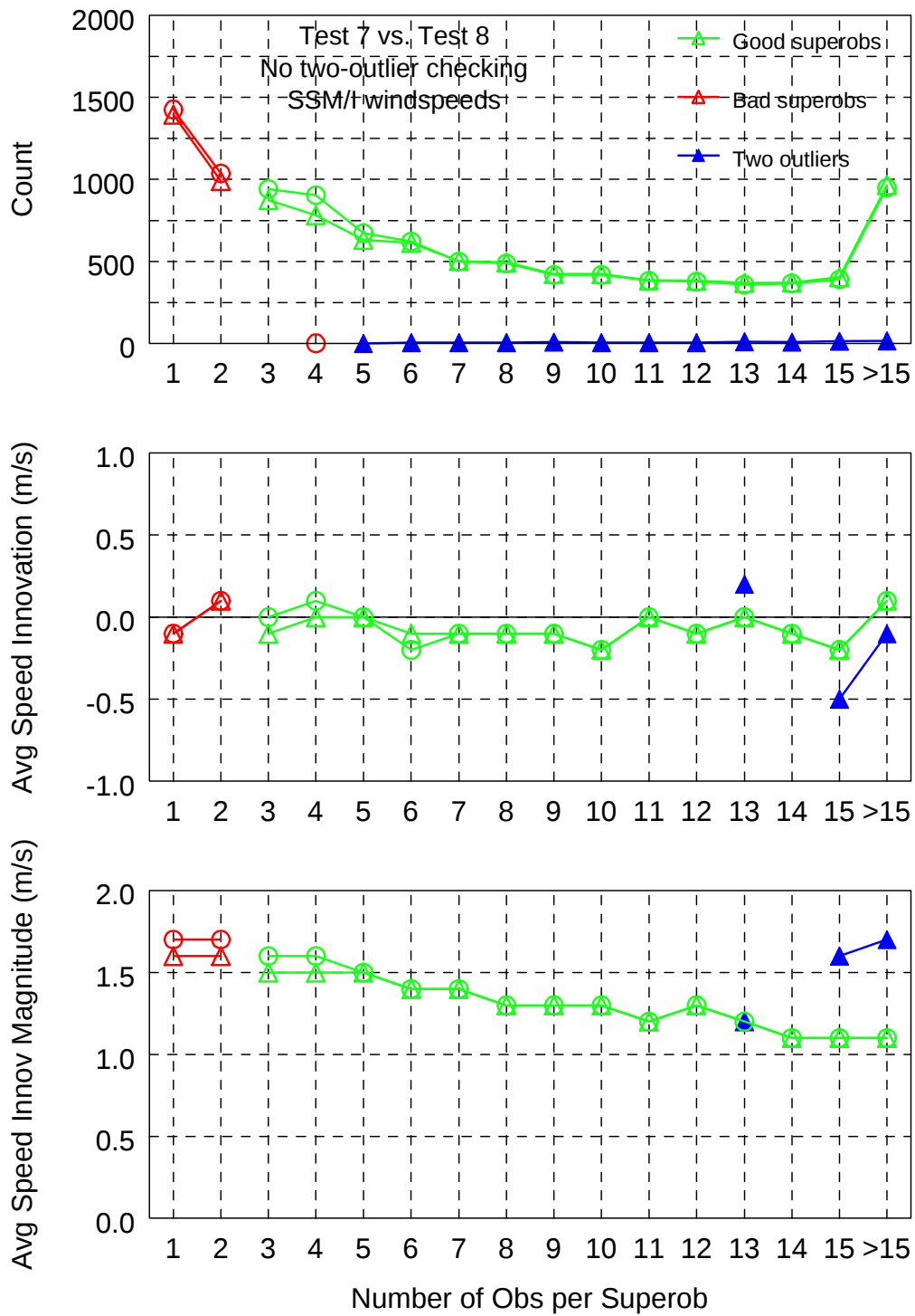
Figure 26: Same as Fig. 21 except for SSM/l windspeeds with (triangles) and without (circles) two-outlier checking.
