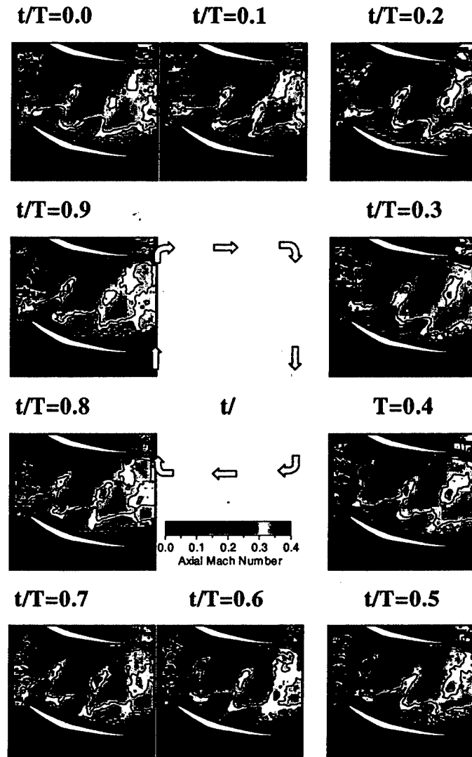
Figure 30. Time-variant stator axial mach number at transonic rotor speed
