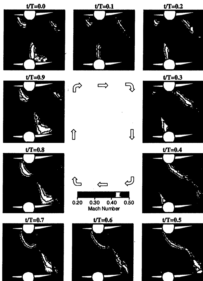
Figure 13. Time-variant IGV flow field for nominal loading at 20,000 rpm
