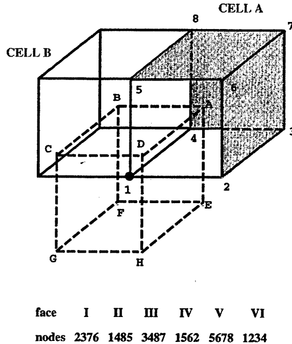
Figure 3.4: Contribution of cell A to the second order flux integration.
