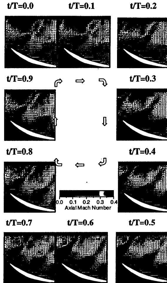
Figure 31. Unsteady stator pressure surface velocity vectors at transonic rotor speed
