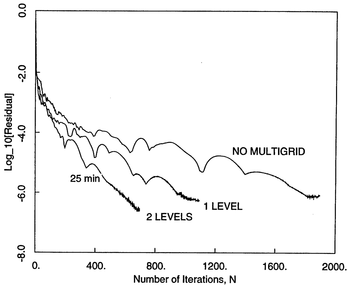
Figure 6.16: 3D Compressor. Steady code convergence history. Grid: IGV(81×17×17), R1(81×17×17), S1(81×17×17). Total number of nodes 70,227.
