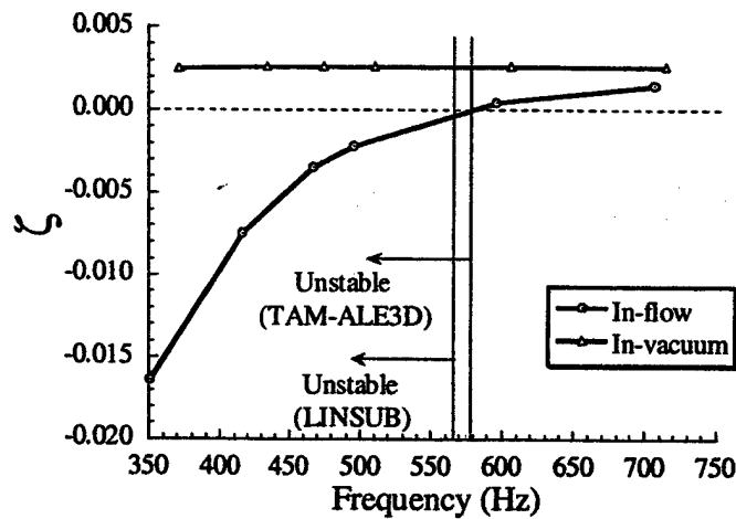
Figure 78. Decay rate for 1 st torsion mode, e^{-\zeta}
