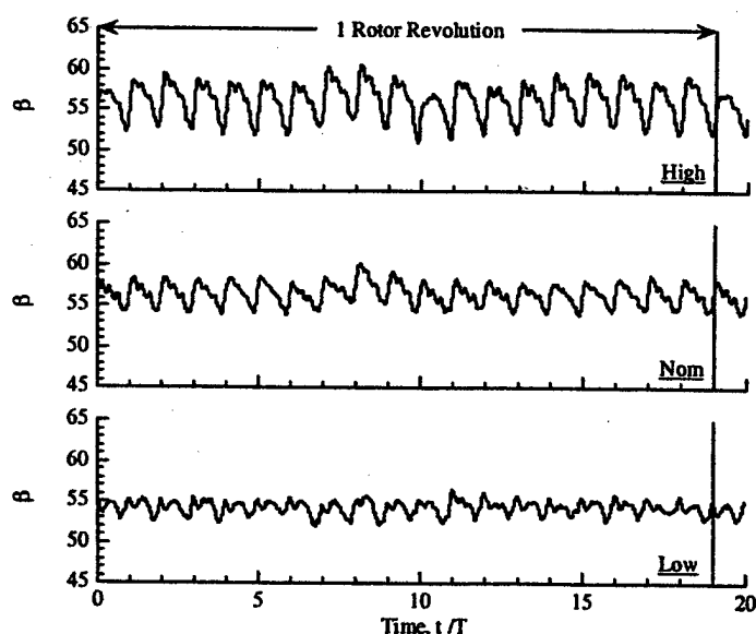
Figure 33. Steady loading effect on rotor wake relative flow angle
