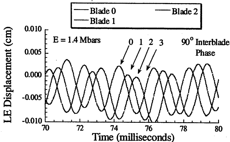
Figure 79. Tuned rotor blade leading edge displacement showing 90^\circ interblade phase angle
