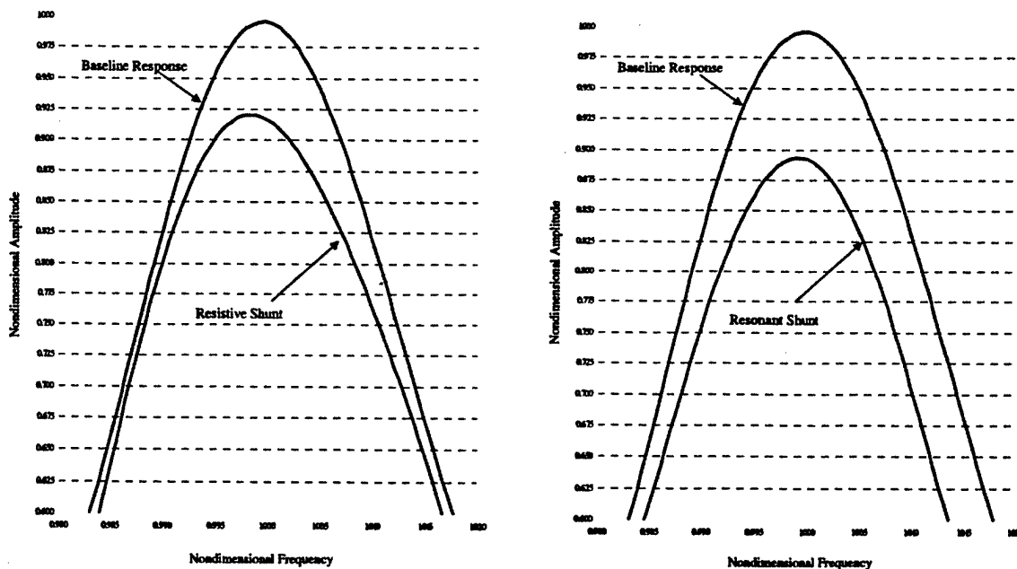
Figure 92. Piezoelectric controlled response of LPE vane
