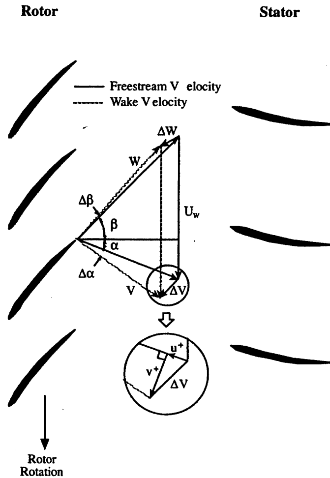
Figure 2. Stator excitation due to rotor wake
