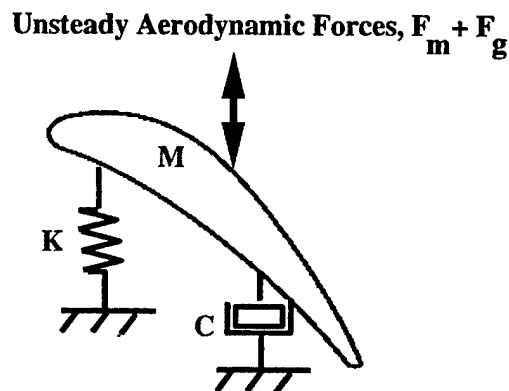
Figure 1.1: Turbomachinery blade model.
