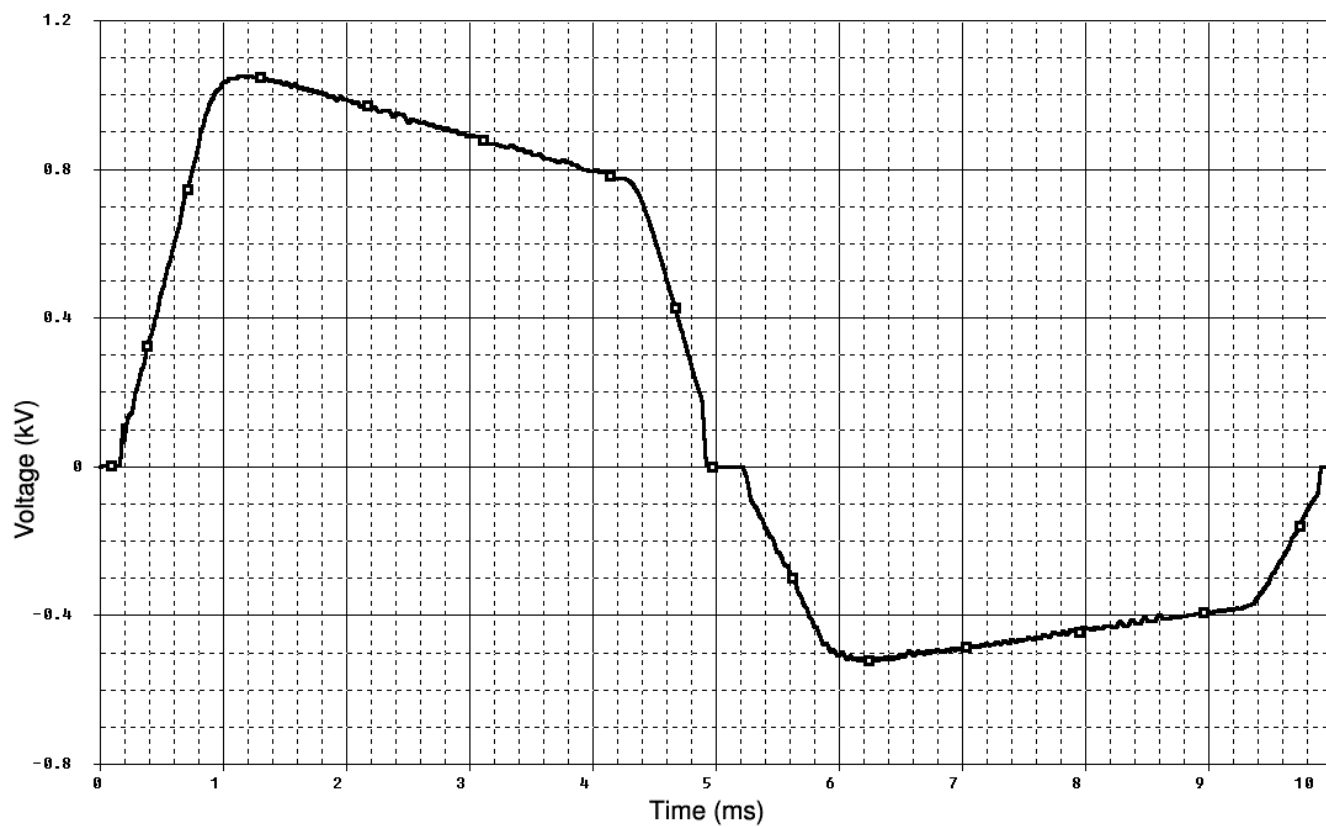
Fig.4. Voltage-time curve for 200 J delivered energy and 25 Ω load resistance.
