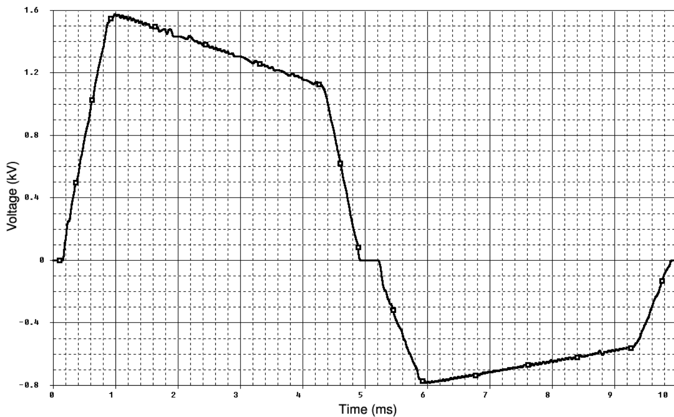
Fig.3. Voltage-time curve for 200 J delivered energy and 50 Ω load resistance.
