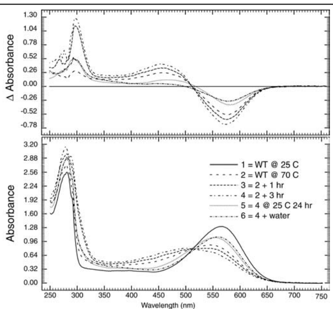
Figure 3.15: UV-visible spectra of bR in 85% glycerol heated to 70°C, then cooled back to 25°C and rehydrated. The spectrum of the rehydrated sample was normalized to the 280 nm peak of spectrum 5. Significant differences can be seen at 300 nm after heating, and at 370 nm, 450 nm, and 560 nm following rehydration.
