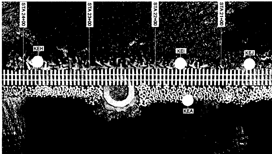
Figure 13. Locations of targeted armor units on Kahului east breakwater
