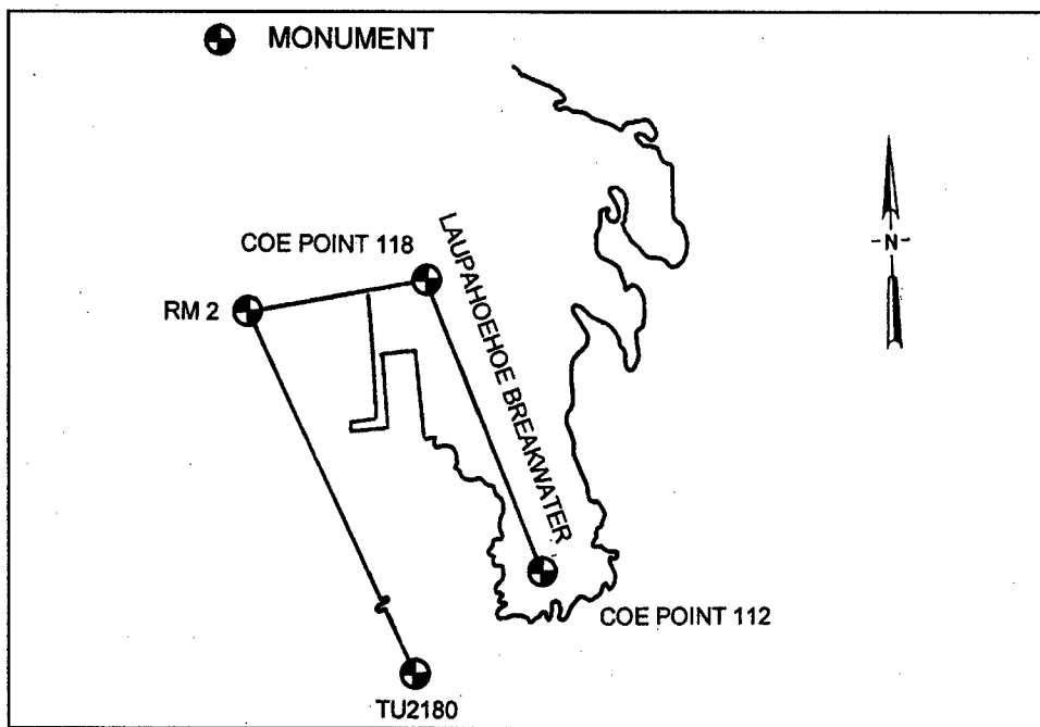
Figure 12. Monuments used to establish survey control at Laupahoe boat-launching facility
