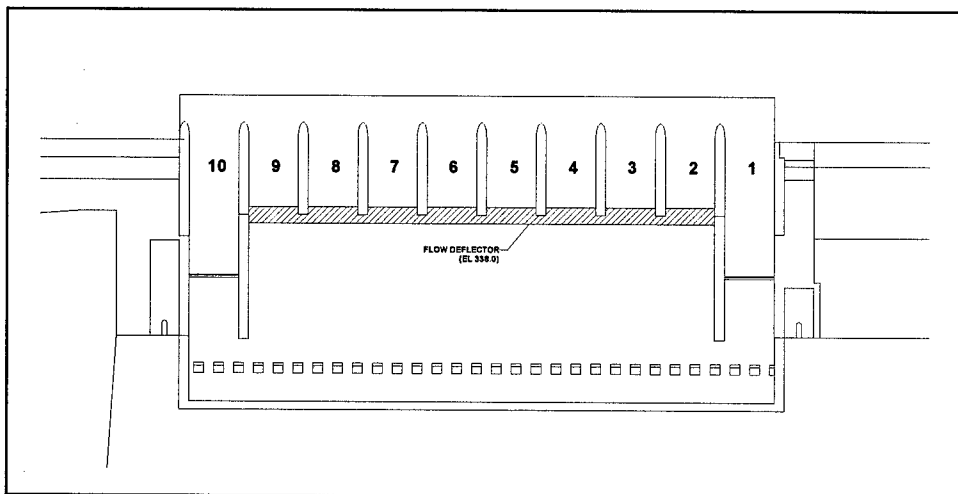
Figure 5. Flow deflectors installed on gate bays 2 - 9
