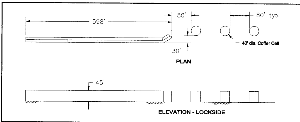
Figure 16. Type 4 design guide wall
