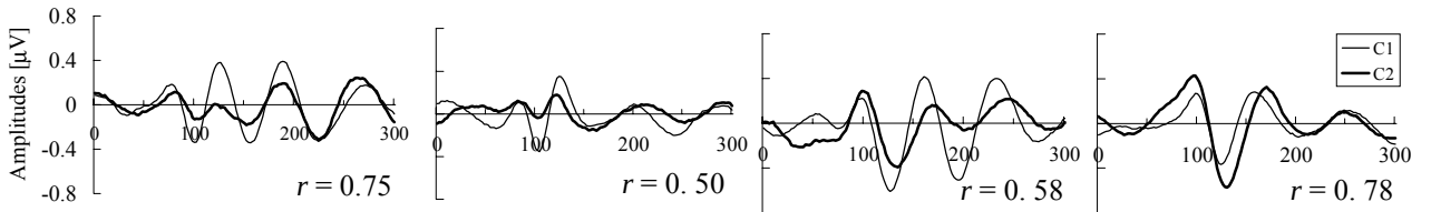
First-order Kernels b_1(\tau)
