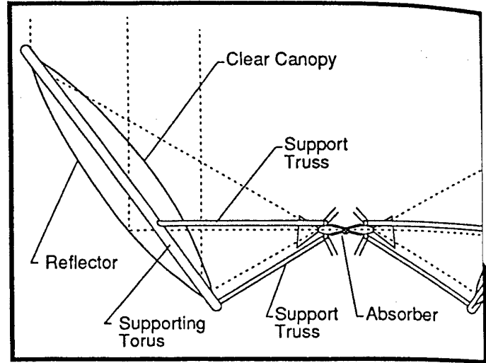
Figure 2 Torus Supported Inflatable Concentrator Concept
