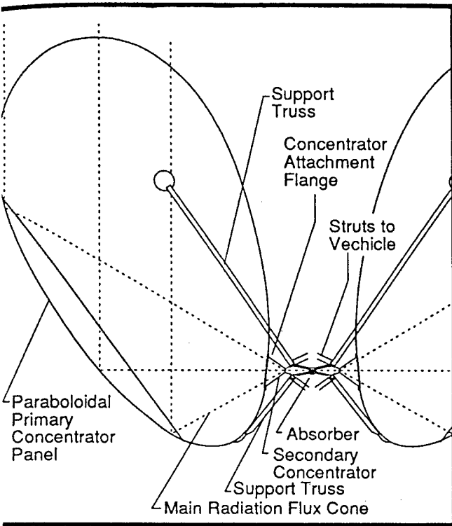
Figure 3 The Single Chamber Inflatable Concentrator Concept
