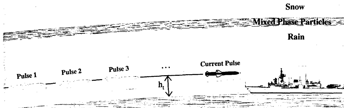
Figure 1. The general scenario modelled by the target simulation. Blue shading depicts the spherical sea surface. Grey shading depicts the three phases of precipitation in the atmosphere. The thin black line depicts the missile trajectory at a constant altitude along a constant azimuth with respect to the radar.
