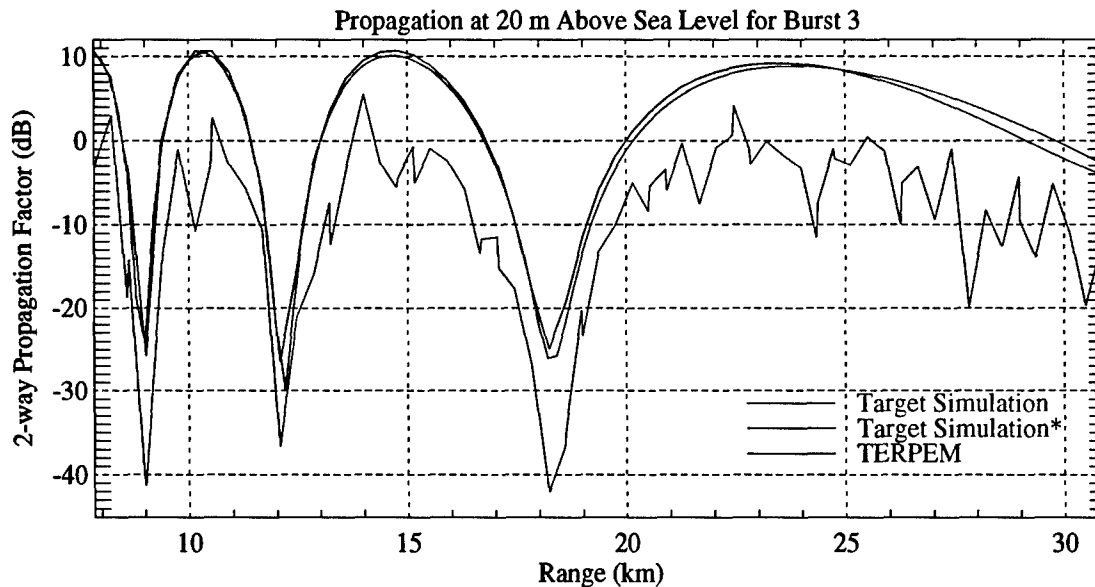
Figure 15. Comparison of the propagation factors calculated by the target simulation and TERPEM. The target simulation data corresponds to the burst 3 waveform parameters. The blue curve shows F_T^4 vs. range. The red curve shows F'^4 vs. range. The green curve shows F^4/P_c vs. range.
