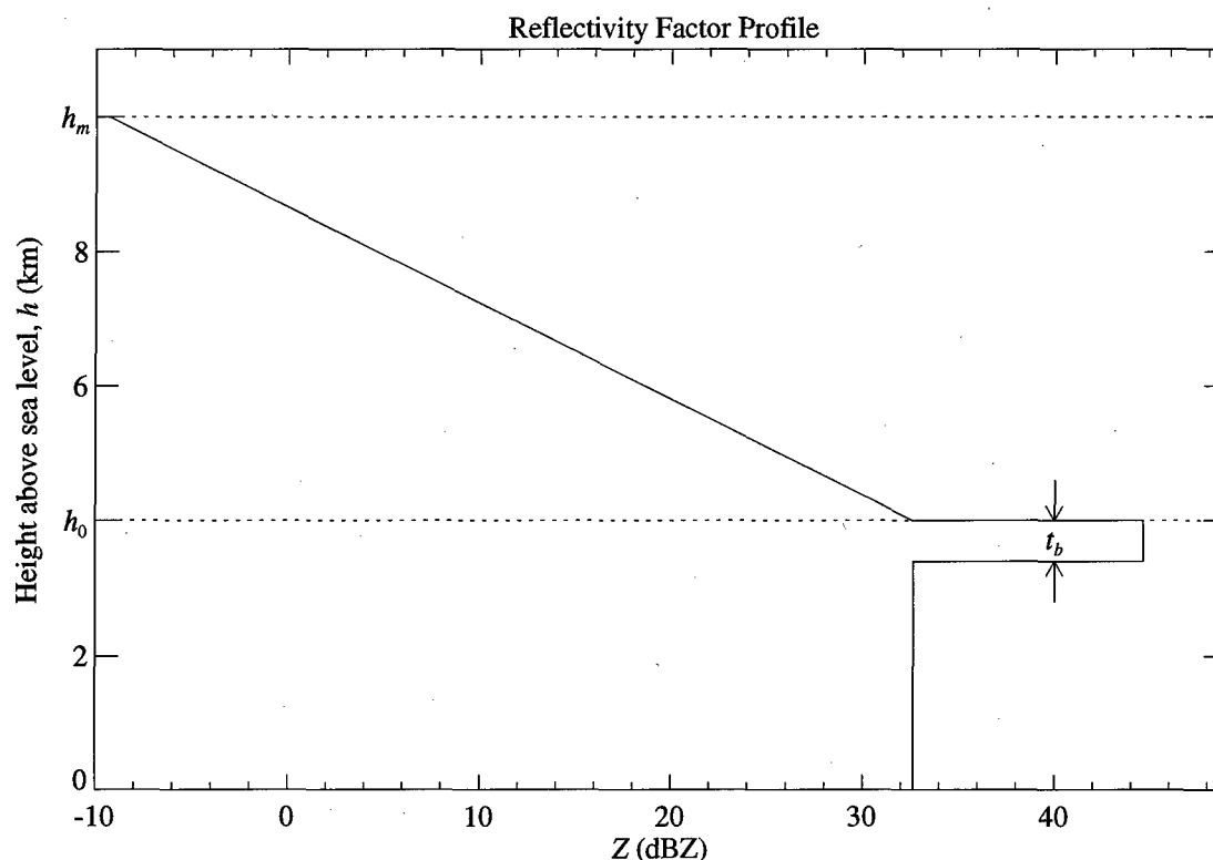
Figure 3. Example height profile of reflectivity factor, Z , where \text{dBZ} = 10.0 \log(Z \text{ in } \text{mm}^6 \text{ m}^{-3}) 4.0 km is where the snow melts into rain. The rain only region is below 3.4 km altitude.
