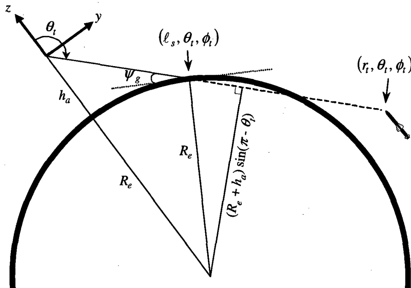
Figure 9. Geometry describing target positions below the radar horizon. The thick blue curve represents the sea surface.
