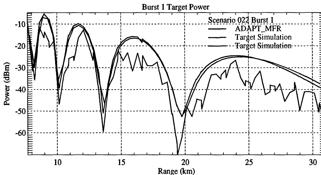
Figure 18. Comparison of the burst 1 target powers generated by the target simulation and ADAPT_MFR for the scenario defined in Tables 1, 2, 3, and 4. The green curve shows the standard output of the target simulation. The red curve shows the data generated by the target simulation without range weighting or statistical fluctuations. The blue curve shows the equivalent target powers generated by ADAPT_MFR.
