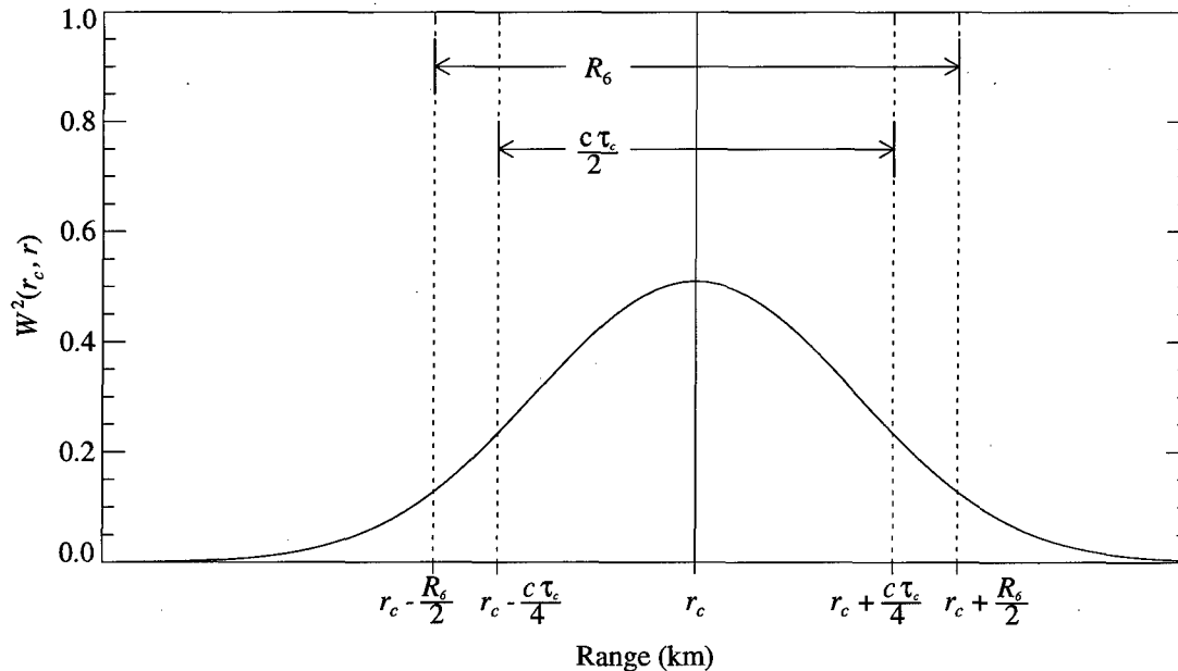
Figure 4. The range weighting function.
