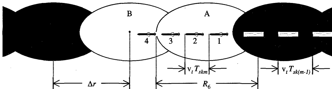
Figure 8. Example of burst missile positions relative to the radar resolution volumes.
