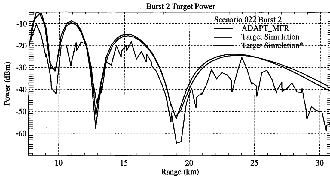
Figure 19. Comparison of the burst 2 target powers generated by the target simulation and ADAPT_MFR for the scenario defined in Tables 1, 2, 3, and 4. The green curve shows the standard output of the target simulation. The red curve shows the data generated by the target simulation without range weighting or statistical fluctuations. The blue curve shows the equivalent target powers generated by ADPT_MFR.
