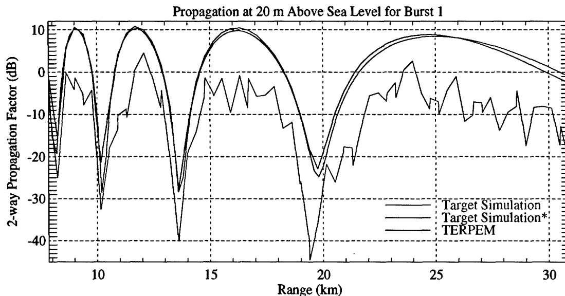
Figure 13. Comparison of the propagation factors calculated by the target simulation and TERPEM. The target simulation data corresponds to the burst 1 waveform parameters. The blue curve shows F_T^4 vs. range. The red curve shows F'^4 vs. range. The green curve shows F^4/P_c vs. range.
