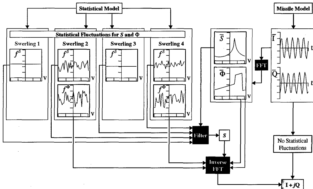
Figure 2. Overview of the computational approach used to generate the target signals. Here the dimension of the abscissa in the power and phase spectra plots is Doppler velocity, v , as opposed to Doppler shift frequency.
