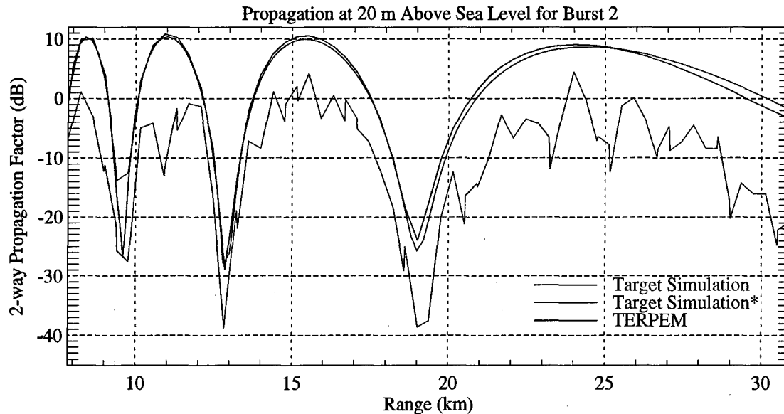
Figure 14. Comparison of the propagation factors calculated by the target simulation and TERPEM. The target simulation data corresponds to the burst 2 waveform parameters. The blue curve shows F_T^4 vs. range. The red curve shows F'^4 vs. range. The green curve shows F^4/P_c vs. range.
