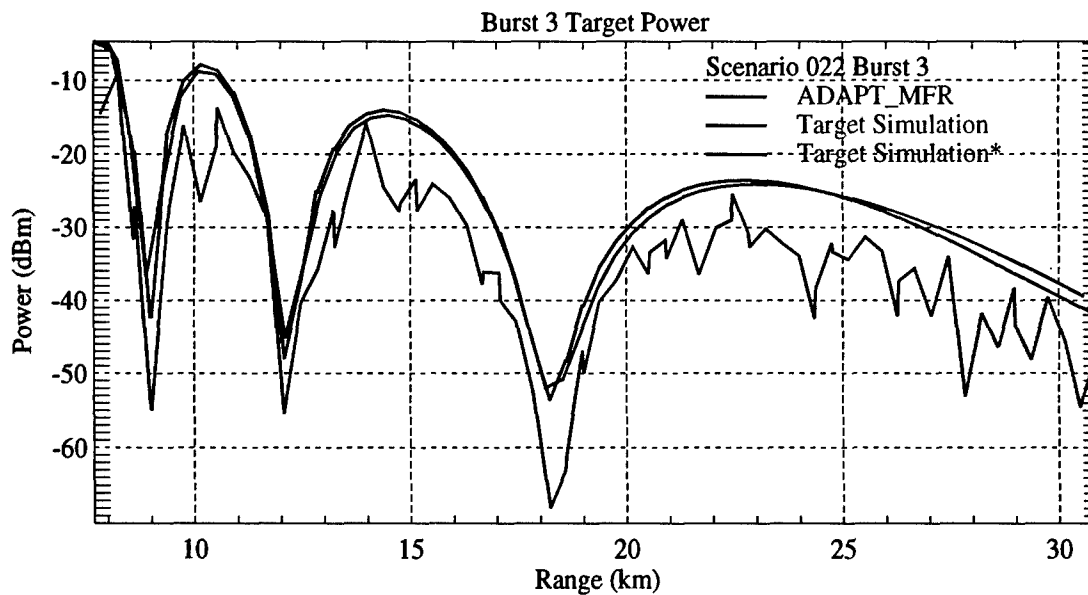
Figure 20. Comparison of the burst 3 target powers generated by the target simulation and ADAPT_MFR for the scenario defined in Tables 1, 2, 3, and 4. The green curve shows the standard output of the target simulation. The red curve shows the data generated by the target simulation without range weighting or statistical fluctuations. The blue curve shows the equivalent target powers generated by ADAPT_MFR.
