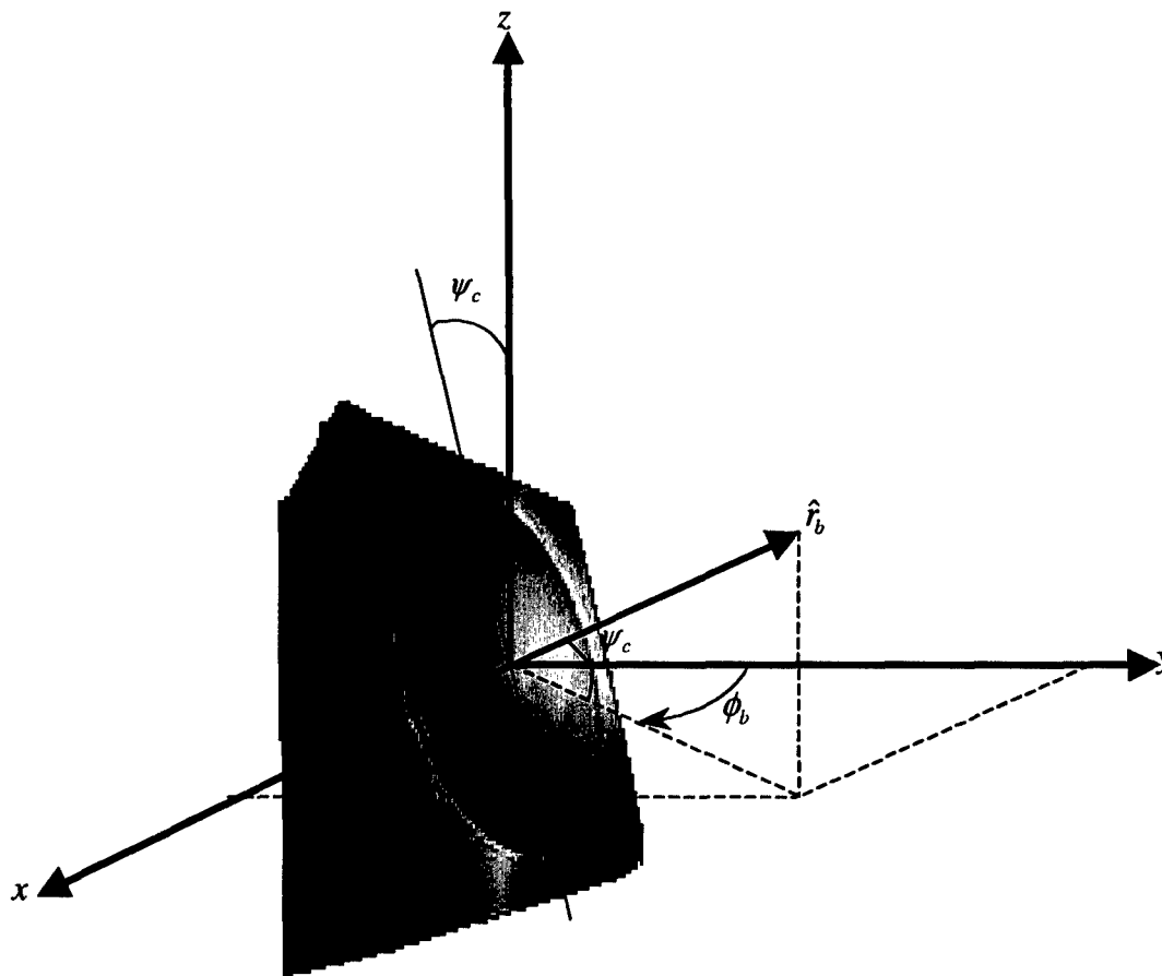
Figure 5. Antenna geometry.
