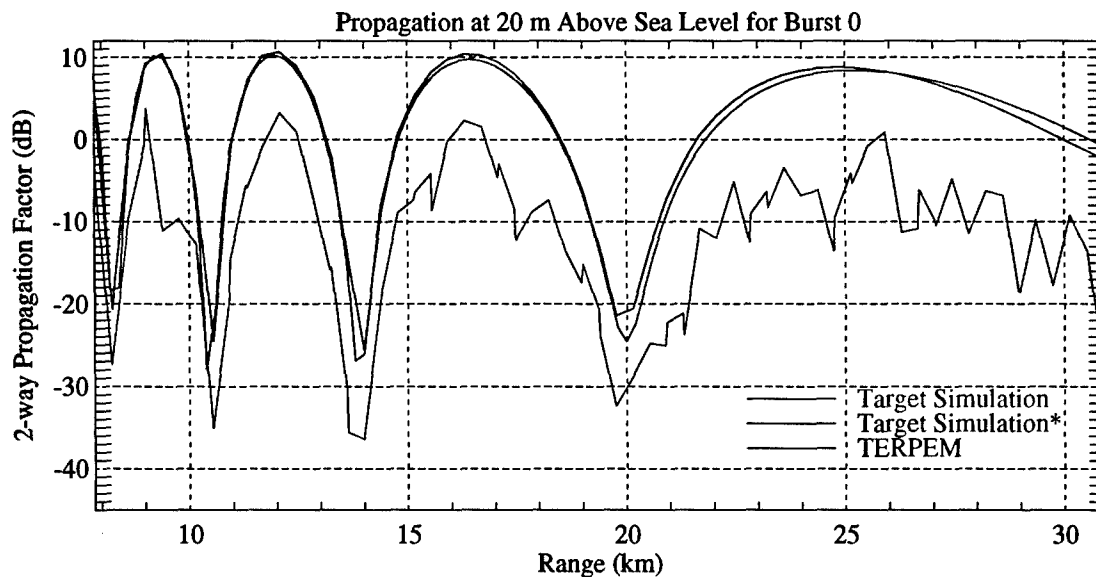
Figure 12. Comparison of the propagation factors calculated by the target simulation and TERPEM. The modelled scenario is represented by the parameters listed in Tables 1, 2, and 3. The T_s , f_r , and N_c parameters for this case represent burst 0 of a four burst dwell that is repeated continuously throughout the flight time of the missile. The blue curve shows F_T^4 vs. range. The red curve shows F'^4 vs. range. The green curve shows F^4/P_c vs. range.
