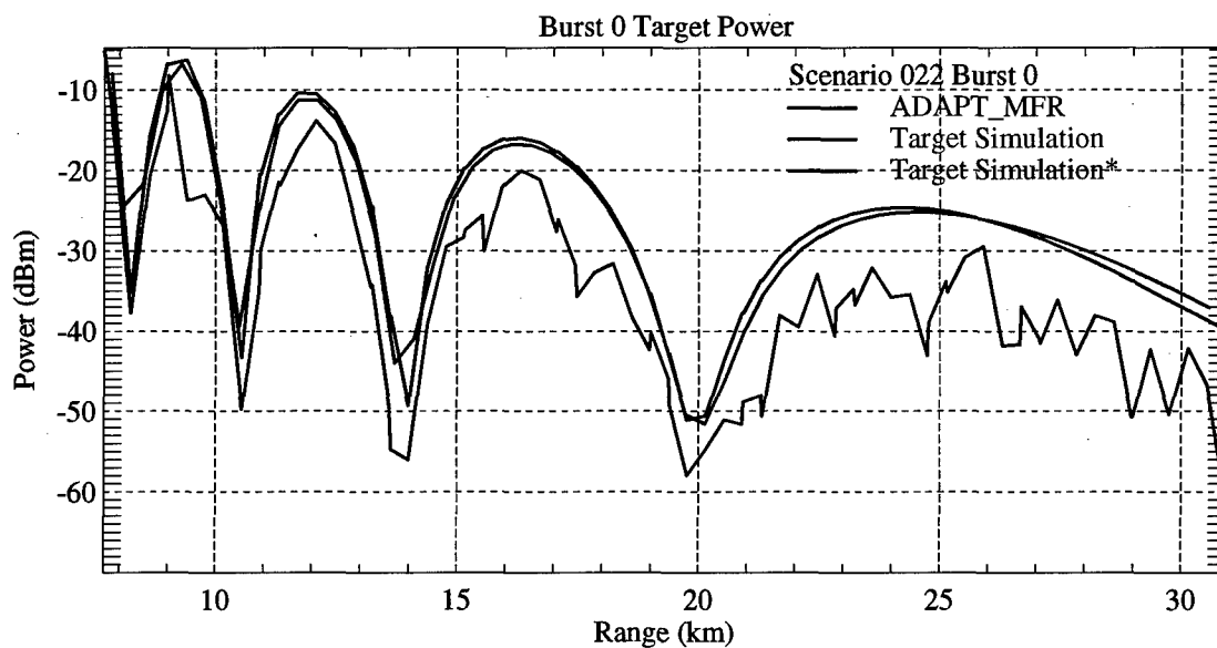
Figure 17. Comparison of the burst 0 target powers generated by the target simulation and ADAPT_MFR for the scenario defined in Tables 1, 2, and 3. The green curve shows the standard output of the target simulation. The red curve shows the data generated by the target simulation without range weighting or statistical fluctuations. The blue curve shows the equivalent target powers generated by ADAPT_MFR.
