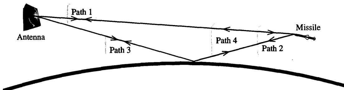
Figure 10. The signal paths that cause interference. The thick blue curve represents the sea surface.
