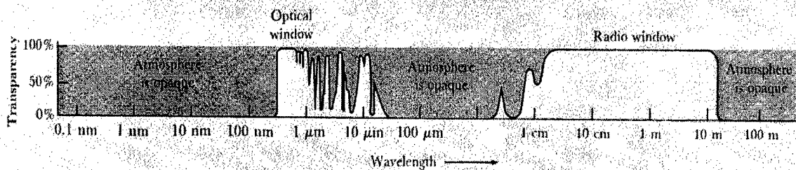
Figure 1: Transmission spectrum of atmosphere
