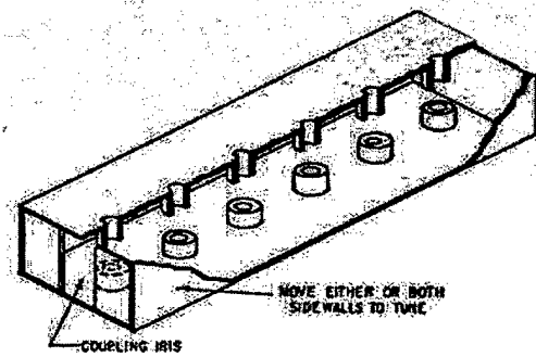
Figure 10: Distributed beam resonator [6].
