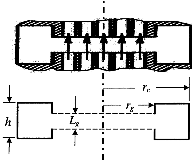
Figure 2: Schematic of a toroidal klystron cavity.
