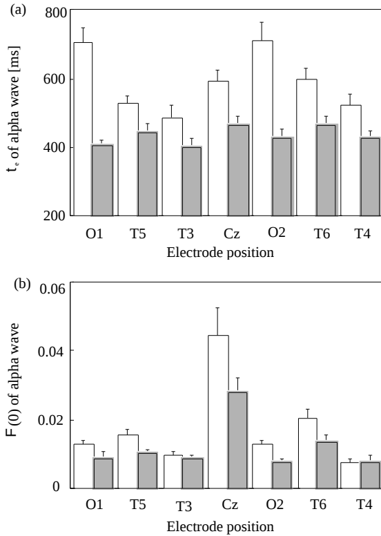
Fig. 4 Calculated (a) t_e and (b) F(0) . Error bars represent 95% confidence, white bars show higher preference, and gray bars show lower preference.
