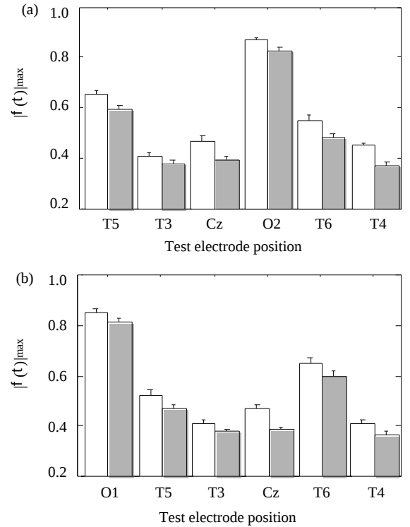
Fig. 6 Calculated |f(t)|_{\max} when (a) reference electrode is O1 and (b) reference electrode is O2. Error bars represent 95% confidence, white bars show higher preference, and gray bars show lower preference.
