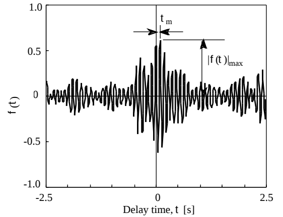
Fig. 3 Definition of |f(t)|_{\max} and t_m of normalized CCF between the alpha waves obtained from the O1 and those from the rest electrode.
