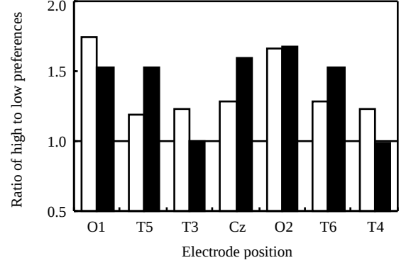
Fig. 5 Ratio of high to low preference in terms of t_e and F(0) . White bars show t_e and black bars show F(0) .
