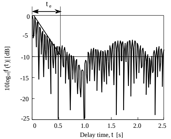
Fig. 2 Example of determining the effective duration of ACF ( t_e ).
