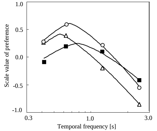
Fig. 1 Scale values of subjective preferences as a function of the temporal frequency. Different symbols indicate different mean luminance. (■): 7.5 \text{cd/m}^2 , (○): 30 \text{cd/m}^2 , (△): 120 \text{cd/m}^2 .
