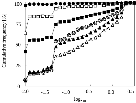
Fig. 7 Cumulative frequency curves of t_m (logarithmic scale) at the most preferred temporal frequency. Each symbol indicates different test electrode: (□) T5, (△) T3, (●) O2, (■) T6, (▲) T4, and (○) Cz (Reference electrode is O1).
