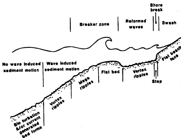
Figure 1. Schematic showing different regions of the surf zone (Nielsen, 1992).
