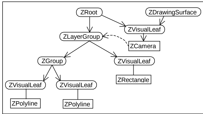
Figure 4: Run-time object structure in a typical application. This scene contains a single camera looking onto a layer that contains a rectangle and a group consisting of two polylines.
