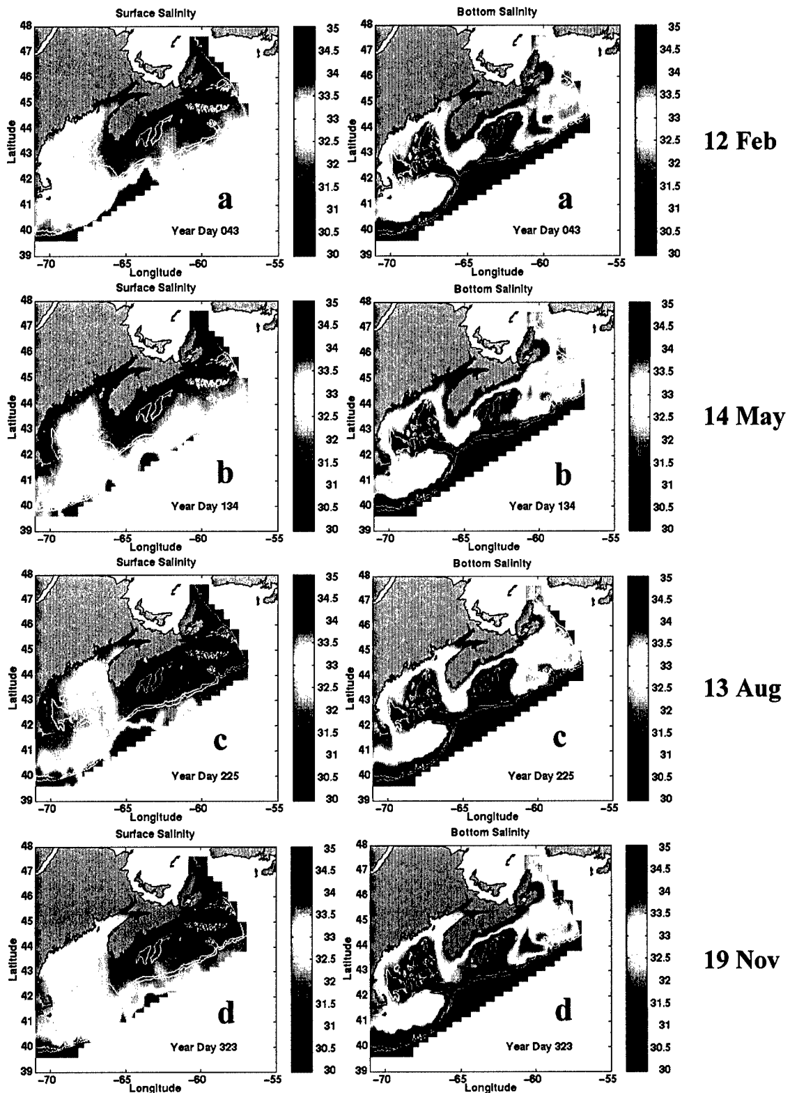
Fig. 11 — Regional surface and bottom salinities for representative days during: (a) winter (b) spring, (c) summer, and (d) fall (from www.mar.dfo-mpo.gc.ca/science/ocean/scotia/ssmap.html )
