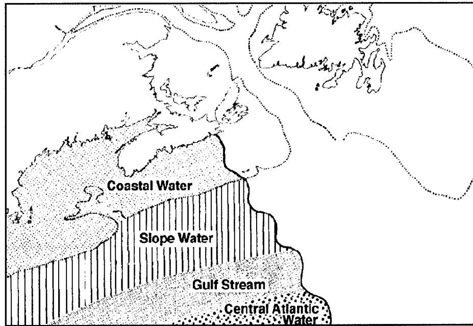
Fig. 3 — Approximate location of water masses moving offshore of Nova Scotia (from http://museum.gov.ns.ca/mnh/nature/nhns/index.htm , T6.2)
