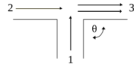
Fig. 2. Converging flow diagram
