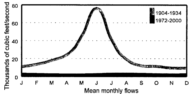
Fig. 40. Comparison of average monthly flows of the Colorado River at Yuma, Arizona prior to 1904–1934 construction of Boulder Dam and current river flows (1972–2000).
