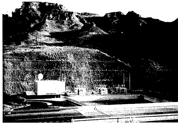
Fig. 38. Colorado River water is lifted nearly 800 feet by the Lake Havasu Pumping Plant located on Lake Havasu near the confluence of the Bill Williams River.
