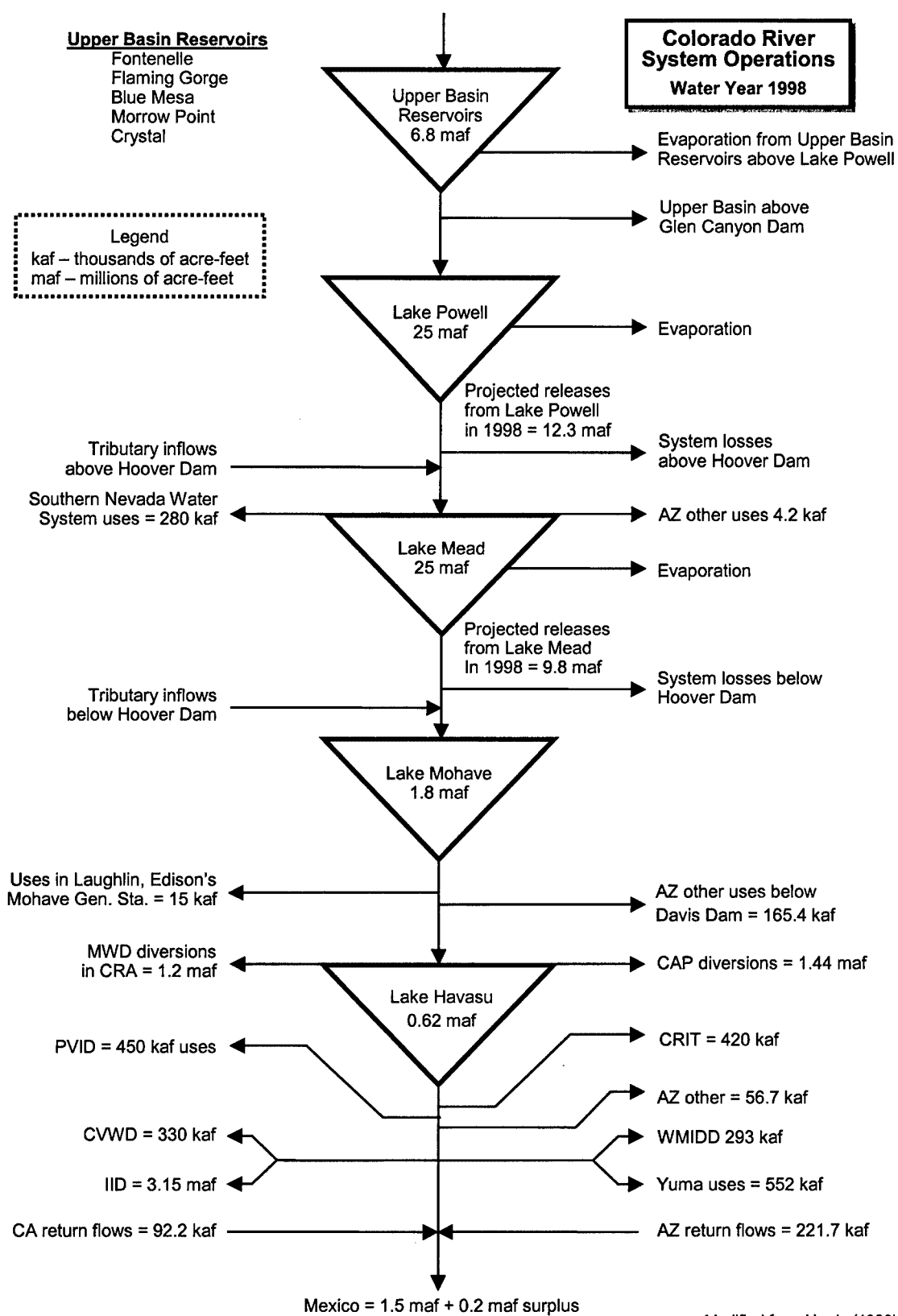
Fig. 24. A diagram of the source and fate of the Colorado River (Harris, 1998).
