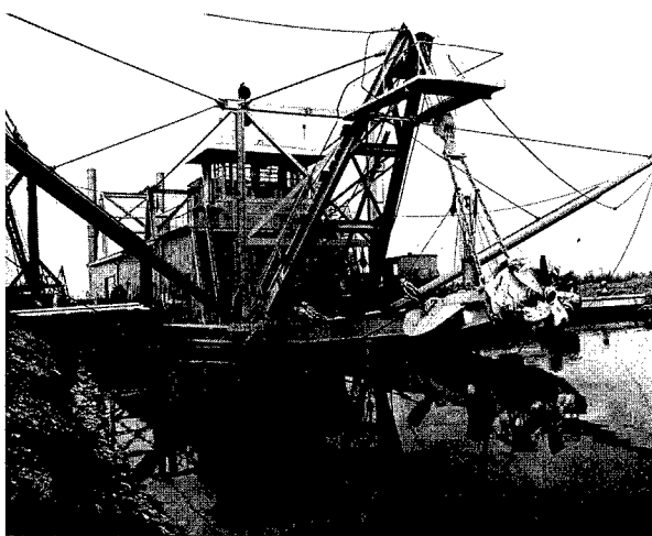
Fig. 23. The dredge Colorado straightened 30 miles of the Colorado River near Needles, California. Here the dredge is tied at Needles in 1949, P423-3000-1808A. Courtesy of the Bureau of Reclamation, Boulder City, Nevada.
