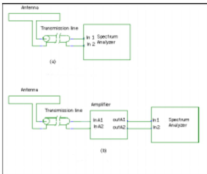
Fig. 1: Application of the amplifier in the test system. The upper figure shows the system without the amplifier, while the lower figure shows the enhanced system with the amplifier inserted between the antenna feeder and the spectrum analyzer.
