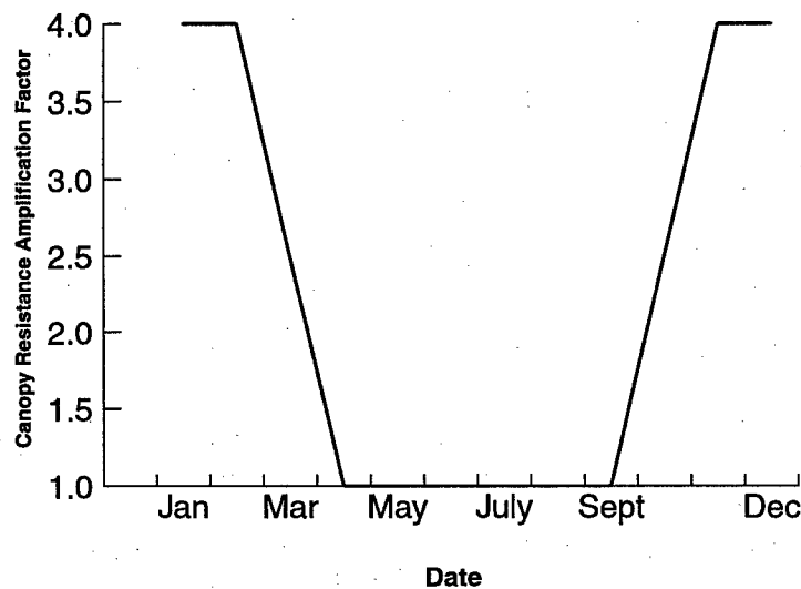
Figure 20. Annual variation in canopy resistance when seasonal resistance is selected
