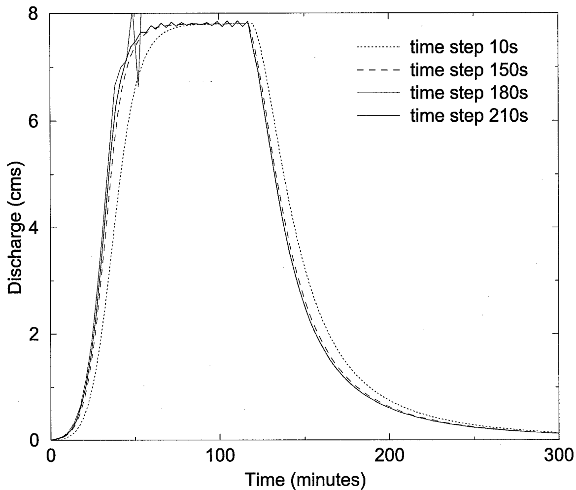
Figure 5. Example of a temporal convergence study. The hydrograph produced by the 10-sec time-step can be considered the most correct because it has the shortest time-step. The 210-sec time-step hydrograph crashed partway through the run. The 180-sec time-step, shows the oscillations that will be produced by a time-step too close to the limiting or crashing time-step. The 150-sec time-step appears normal, but when judged against the 10-sec time-step, the significant difference in peak time is observed, making the 150-sec time-step also inappropriate
