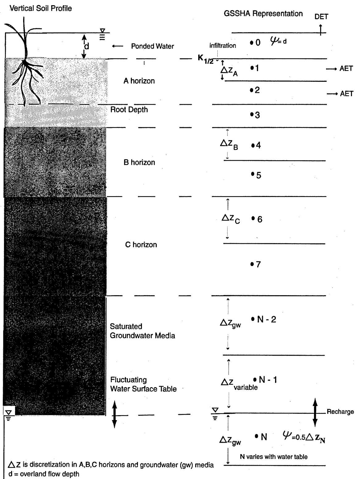
Figure 21. GSSHA representation of the unsaturated zone
