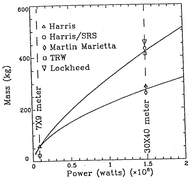
Figure 6: TRADE-STUDY MASSES OF SOLAR-THERMAL THRUSTER CONCENTRATOR SYSTEMS.
