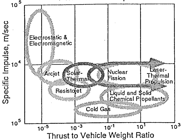
Laser-Thermal Propulsion Performance Comparison
