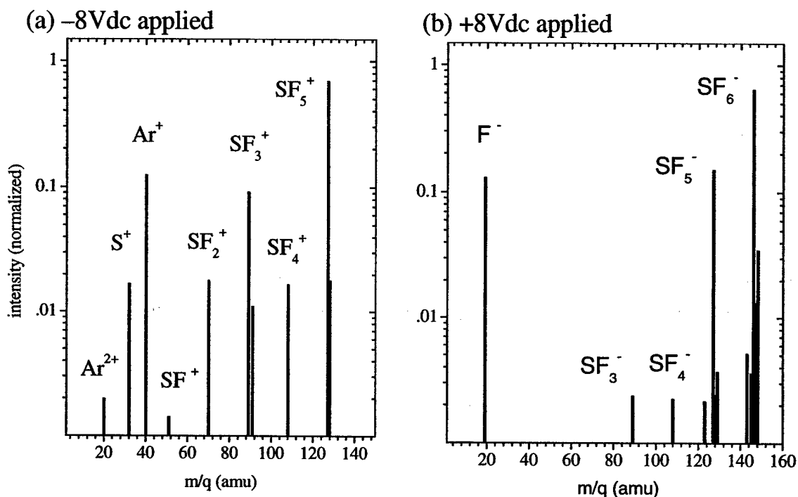
Figure 4 Mass spectrum of (a) cations and (b) anions drawn to biased electrode for a 50 mtorr Ar/50 mtorr SF_6 mixture.
