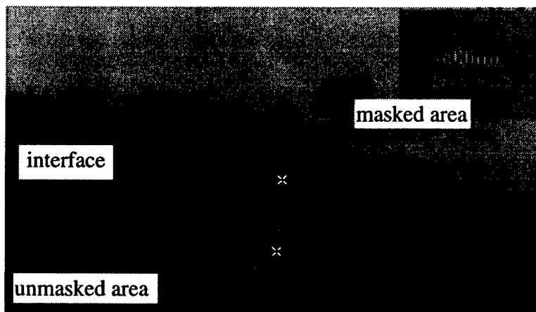
Figure 1 SEM of silver mask edge where a sloped interface superimposed on alumina micro-masked features formed, showing the different sidewall evolution. Etch conditions were 65 mtorr Ar/5 mtorr SF 6 and -100 V bias .
