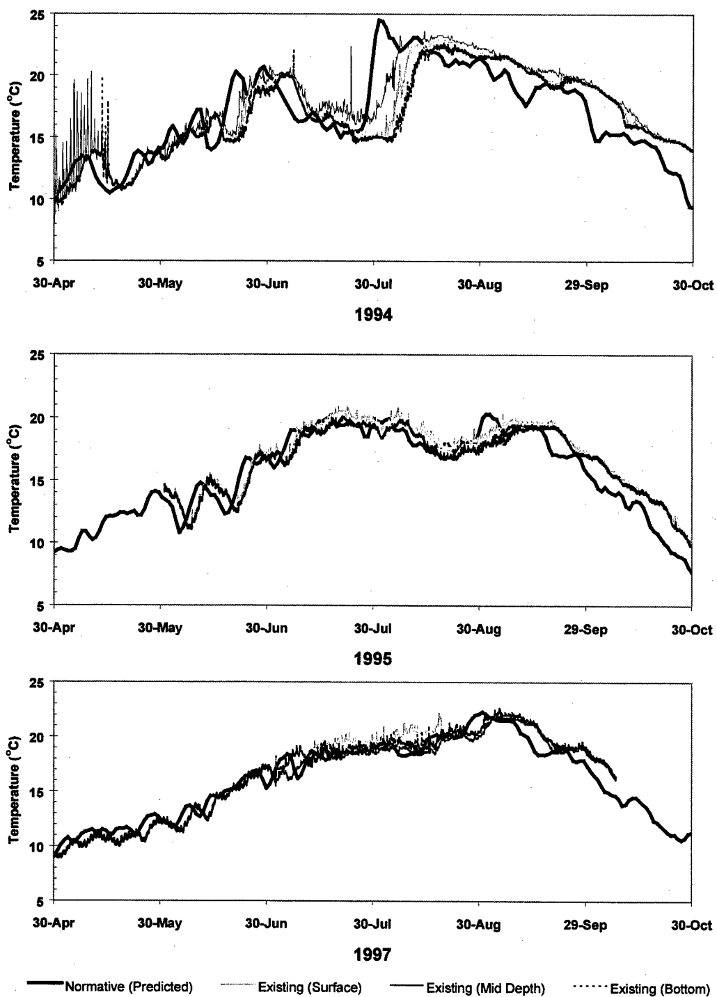
Figure 4-1. 1994, 1995, 1997 Near-natural River Temperatures Predicted by WQRRS Compared with Existing Water Temperatures (Normandeau, 1999a) RM 110.5
