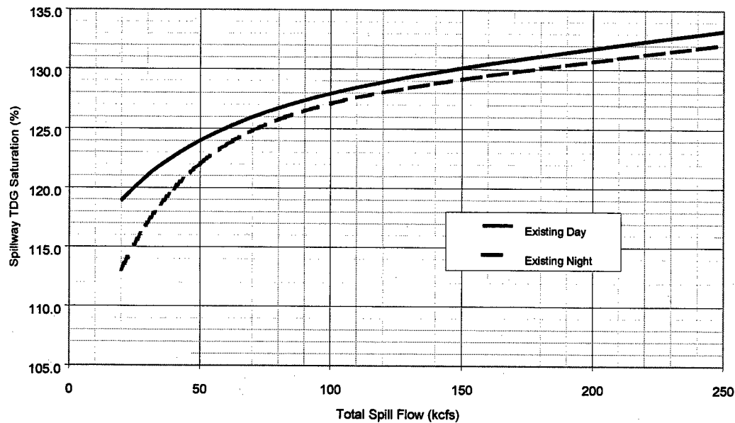
Figure 4-15. Lower Monumental Lock and Dam 1998 TDG and Total Spill Flow (day versus night) Source: Developed by the Corps
