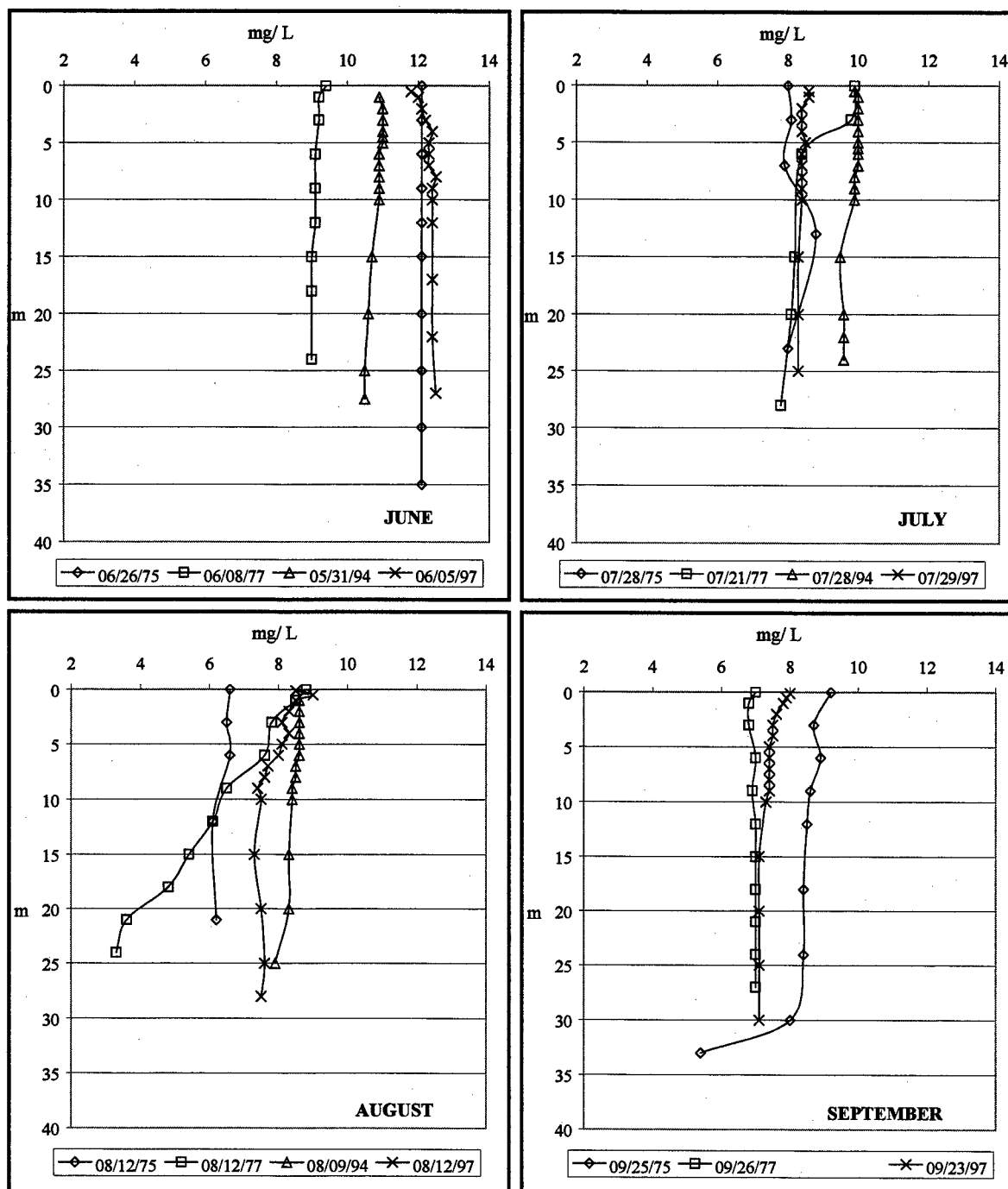
Figure 3-34. Dissolved Oxygen Profiles for the Sampling Station at SNR-83
