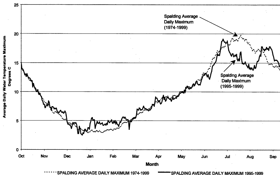
Figure 3-10. Average Daily Maximum Water Temperature (°C) Source: Developed by the Corps
