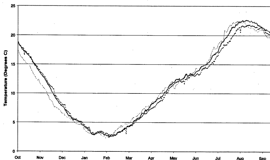
Figure 3-14. Average Maximum Temperatures in Degrees Celsius, 1974 through 1981 Source: Developed by the Corps
