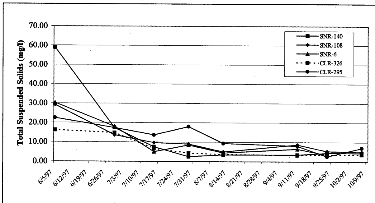
Figure 3-41. The TSS for Selected Sampling Stations in 1997
