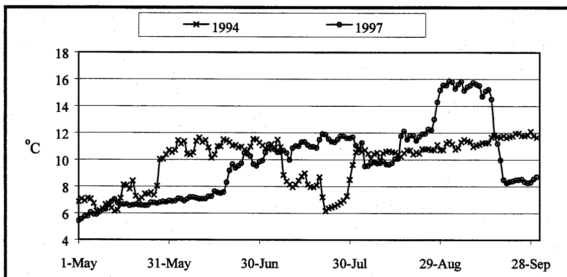
Figure 3-24. Daily Temperatures in the Dworshak Reservoir Outlet, 1994 and 1997
