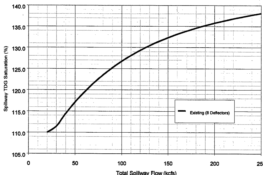
Figure 4-13. Lower Granite Lock and Dam 1998 TDG and Total Spillway Flow Source: Developed by the Corps
