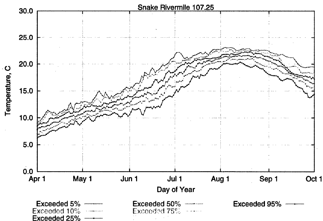
Figure 4-9. The MASS □ Simulated Temperatures for Lower Snake River with Reservoirs in Place at RM 107
