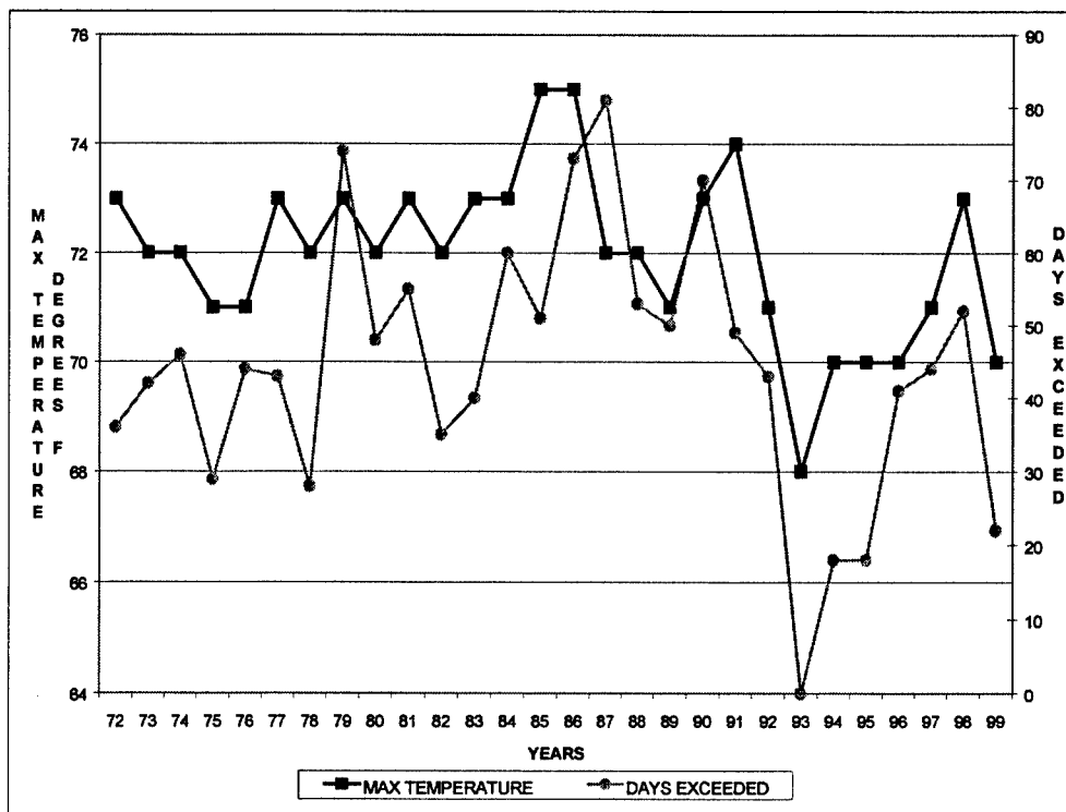
Figure 3-19. Days Exceeding 68°F (20°C)–Ice Harbor Dam Scroll Case Temperature Source: Developed by the Corps
