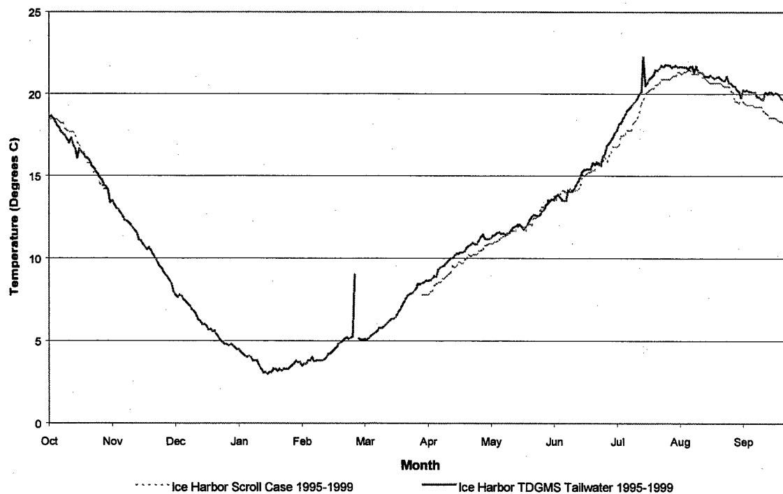
Figure 3-12. Average Maximum Temperatures in Degrees Celsius, 1995 through 1999
