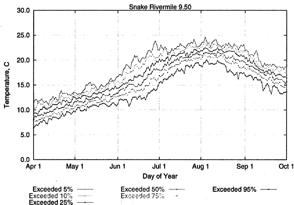
Figure 4-8. The MASS □ Simulated Temperatures for Lower Snake River with Near-Natural River Conditions at RM 10
