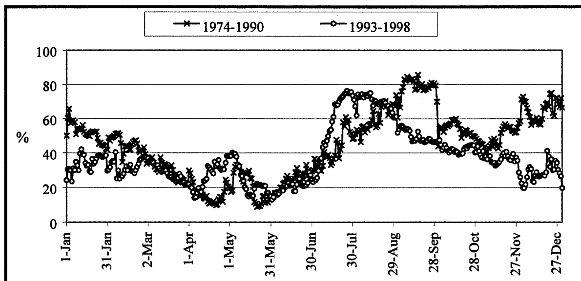
Figure 3-25. Flow in the Clearwater River at Spalding, Idaho—Percentage Due to Discharge from the Dworshak Reservoir, Idaho
