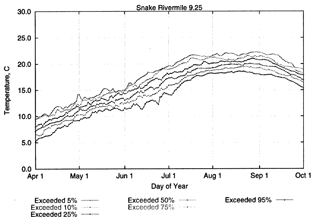
Figure 4-11. The MASS □ Simulated Temperatures for Lower Snake River with Reservoirs in Place at RM 10
