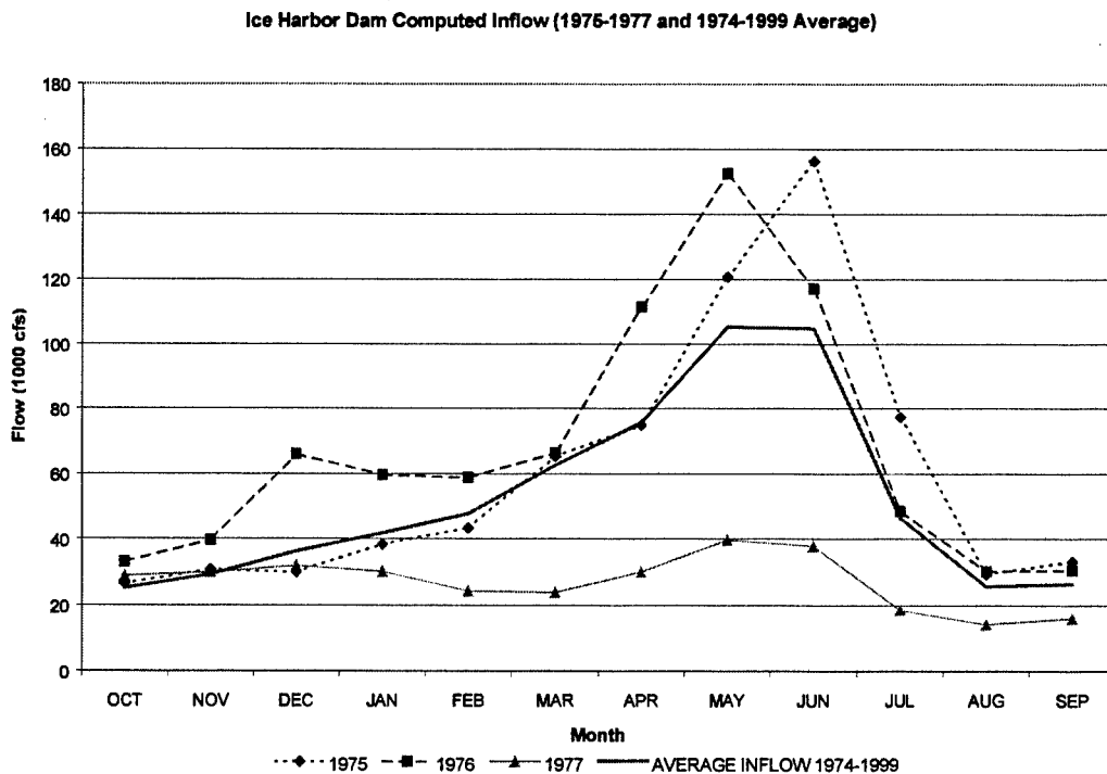
Figure 3-3. Monthly Mean Flow Data at Ice Harbor Dam for the Years 1975 through 1977
