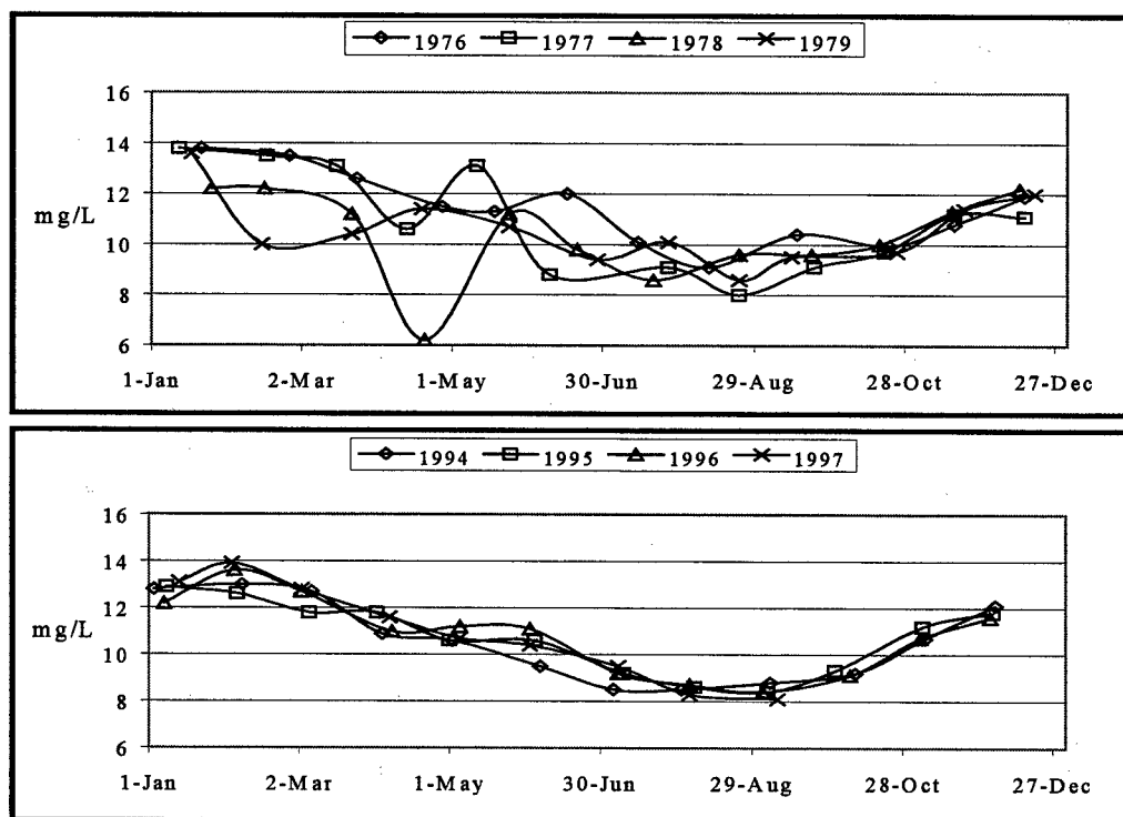
Figure 3-36. Dissolved Oxygen Data Collected at the USGS Gaging Station at SNR-167.2 during 1976-1979 at the Anatone Gaging Station and at the Ecology Monitoring Site at SNR-132.9 during 1994-1997
