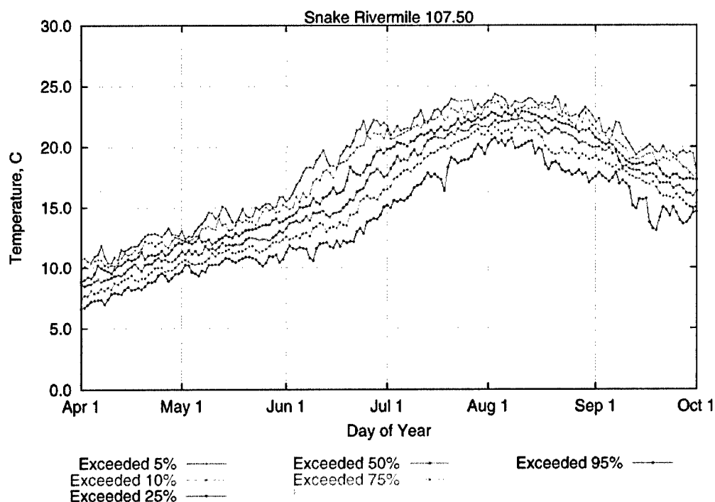
Figure 4-10. The MASS □ Simulated Temperatures for Lower Snake River with Near-Natural River Conditions at RM 107
