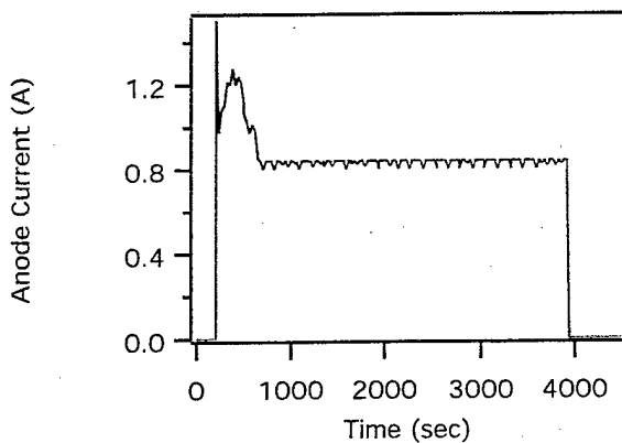
Fig. 4. Anode current trace characteristic of a start following exposure of the thruster to atmospheric conditions for several days. Duration of the anode current transient is 420 seconds. Note: initial current spike to 1.5 A is caused by start-up sequence.
