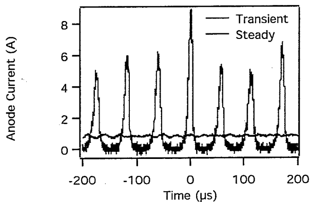
Fig. 8. Current oscillations of the transient and steady state cases seen in the time domain. Conditions are analogous to those in Fig. 4.
