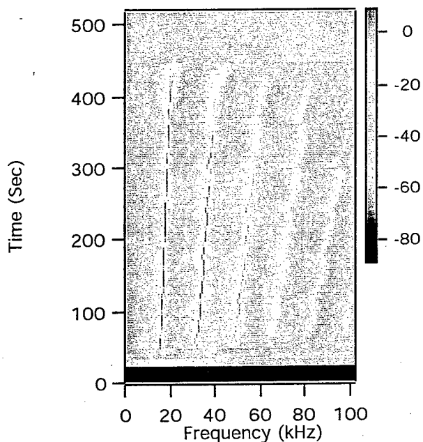
Fig. 7. Contour plot showing the time evolution of the anode Log Magnitude Peak Current (dBA) during a start where the anode current transient is present.
