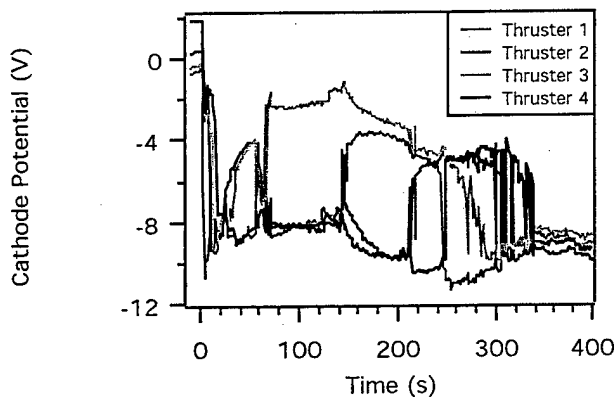
Fig. 3. Cathode potential during the transient of four clustered Hall thrusters.
