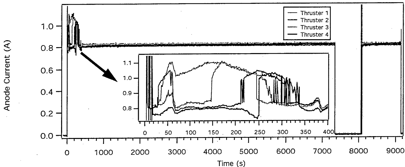
Fig. 2. Anode current transient of four nearly simultaneously started thrusters. Note the transient persists for ~400 seconds and does not reappear in a later restart of the cluster.
