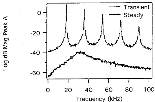
Fig. 6. Two spectra of current oscillations. The first during the transient with an average current of 1.14 A, and the second during steady state operation with an average current of 0.84 A.
