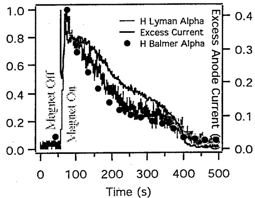
Fig. 12. Normalized hydrogen emission (Balmer alpha, and Lyman alpha) compared to the excess anode current (defined as actual current minus nominal current).
