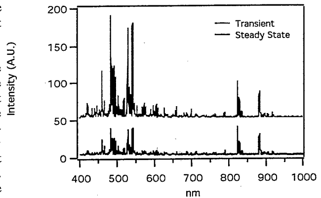
Fig. 10. Visible Spectrum of main discharge. Red—shortly after start with maximum discharge current during start transient. Blue—steady state operation.
