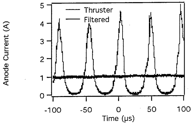
Fig. 9. Current oscillations during the anode current start transient as seen at the thruster and behind the filter at the power supply.
