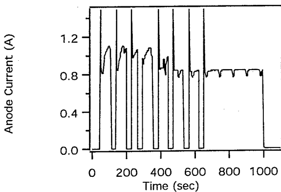
Fig. 5. Anode current trace of the transient with a number of nominally 60 second firings spaced 30 seconds apart. The anomaly persisted for approximately 4.25 min. Note that the thruster has been exposed to regenerated cryo-panel products for a period of 12 days and not exposed to atmosphere.
