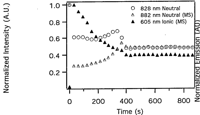
Fig. 11. Normalized representative line intensities for neutral xenon (828 and 882 nm) and ionic xenon (605 nm). Note that the neutral 882 nm and ionic 605 nm transitions have metastable lower states.
