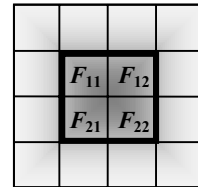
Fig. 1. Selected FFT coefficients for a block of 4 \times 4 pixels.
