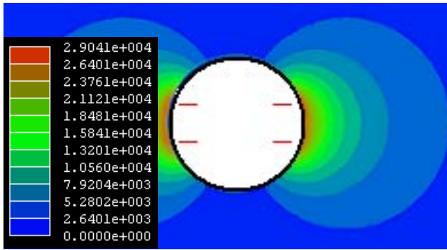
Fig. 4. The distribution of the simulated magnetic losses per unit of coil length in W/m for I = 1 A.
