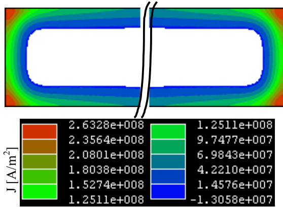
Fig. 2. The distribution of the current density in the cross section of an isolated rectangular infinite long wire for a current I = 1 A.
