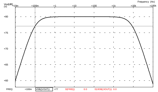
Fig. 4: Frequency characteristic of differential mode gain
