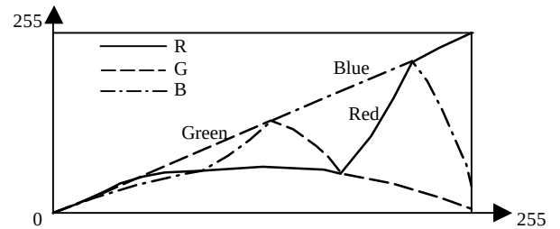
Fig. 1. Pseudo-color transformation using HSV color model
