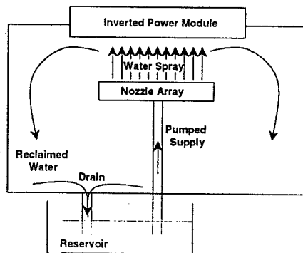
Fig. 17. Schematic of the water-spray facility.
