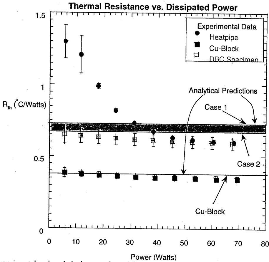
Fig. 12 Experimental and analytical comparison of thermal resistance R_{th} measurement vs. dissipated power.
