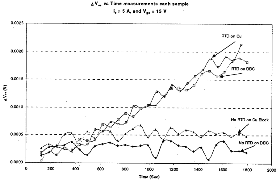
Fig. A.3 Plot of the change in V_{ce} as a function of time for specimens with and without RTD's on both copper block and DBC substrates. Note the relative independence of \Delta V_{ce} with time for the IGBTs without the RTDs, irrespective of DBC or copper block substrate conditions, whereas the \Delta V_{ce} consistently rises with time for the IGBTs with RTDs on both DBC and copper block substrates.
