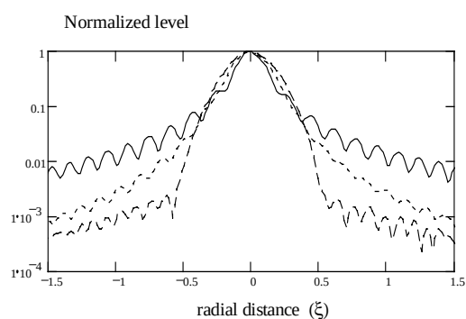
Fig. 1. Numerical results for beam patterns for the fundamental components in water(—uniform, .... cosine, ---exponential)
