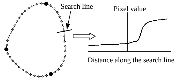
Fig. 3 Left: an initial shape S represented by 45 points, showing edge searching for a particular model point. Right: possible 1D pixel profile along the search line.
