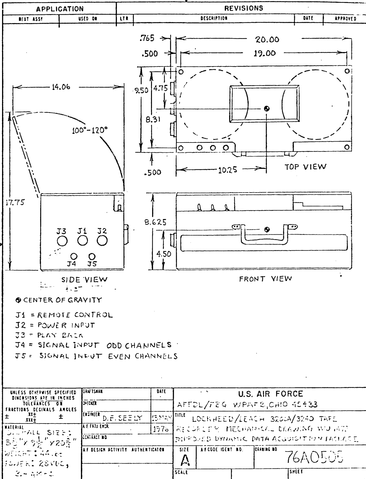
AF 1652 Figure 11 Lockheed/Leach Tape Recorder AWING LAYOUT A VERTICAL
