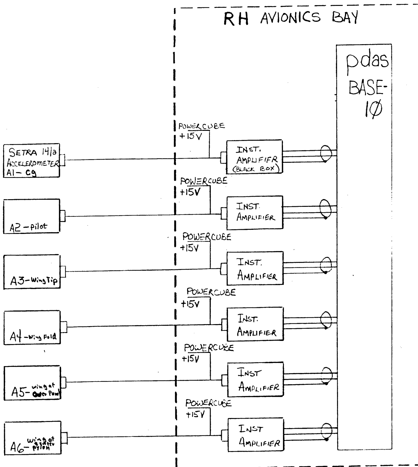
Figure 4 Wiring from Accelerometers to Signal Conditioning
