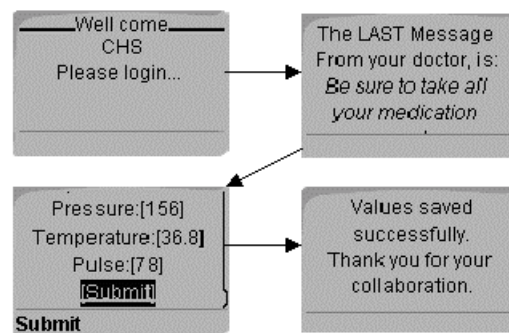
Fig. 3. Screen sequences for a patient session using WAP, with the following units: (a) login and authentication, (b) read possible messages from physician, (c) enter measured values and answer questions, (d) save values.
