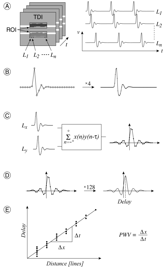
Fig. 2. Summarized description of the signal processing. A) The vessel wall velocities were extracted from the tissue motion given by the TDI information. Two region-of-interests, ROIs, defined the desired wall segments. The velocity was interpolated (B) before crosscorrelation (C). The delay was determined from the interpolated correlation function (D). The pulse wave velocity (PWV) was estimated from the delays between the velocity traces (E).
