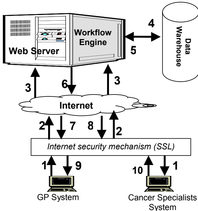
Fig. 1. Proposed web-based WFMS.
