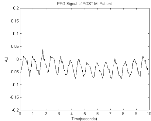
Fig 4b PPG signal of Post MI patient
