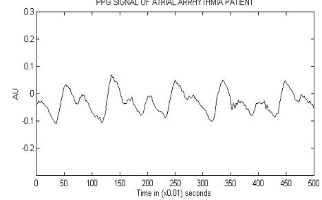
Fig 4a PPG signal of atrial flutter patient
