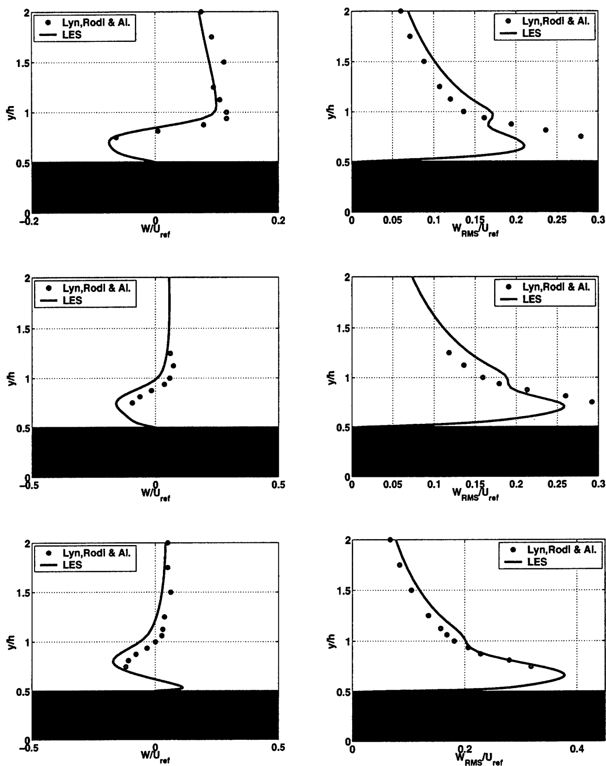
Fig. C.11: Additional simulations, Case II: velocity profiles for vertical velocity, left and vertical RMS, right, at three stations, from top to bottom: x = \frac{1}{4}H , x = \frac{3}{8}H and x = \frac{1}{2}H .
