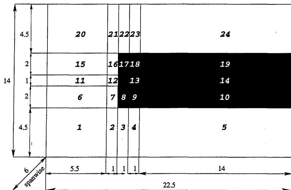
Fig. A.1: Revised multi-domain set-up for computational field. No coloring: 3 d order, upwind treatment of advective term; coloring: 4 th order central treatment of advective term.
