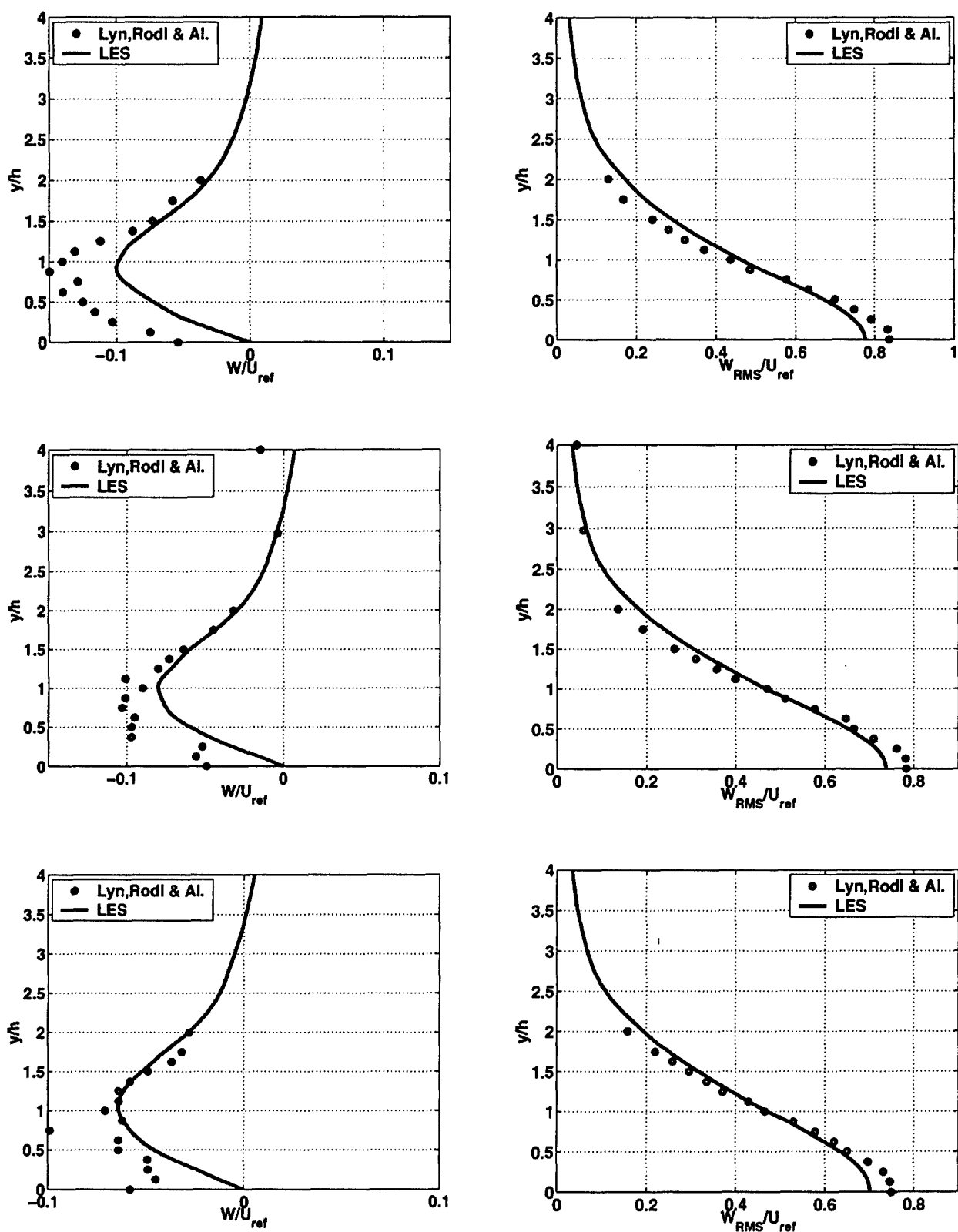
Fig. B.30: Additional simulations, Case I: velocity profiles for vertical velocity, left and vertical RMS, right, at three stations, from top to bottom: x = \frac{18}{8H} , x = \frac{20}{8H} and x = \frac{22}{8H} .
