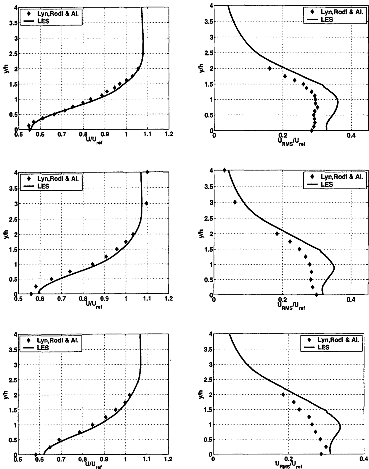
Fig. 2.35: Velocity profiles for stream-wise velocity, left and stream-wise RMS, right, at three stations, from top to bottom: x = \frac{24}{8H} , x = \frac{28}{8H} and x = \frac{32}{8H} .
