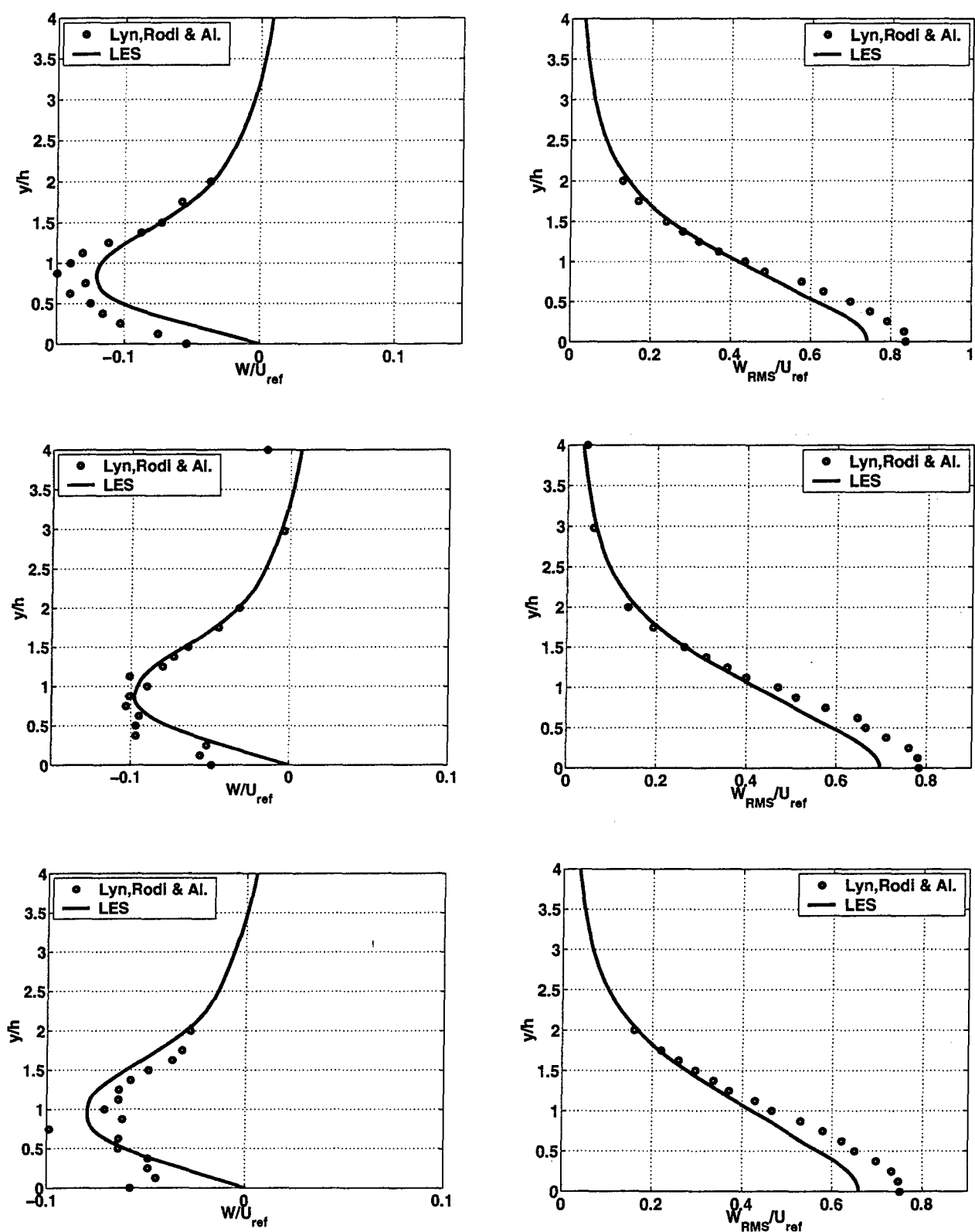
Fig. C.30: Additional simulations, Case II: velocity profiles for vertical velocity, left and vertical RMS, right, at three stations, from top to bottom: x = \frac{18}{8H} , x = \frac{20}{8H} and x = \frac{22}{8H} .
