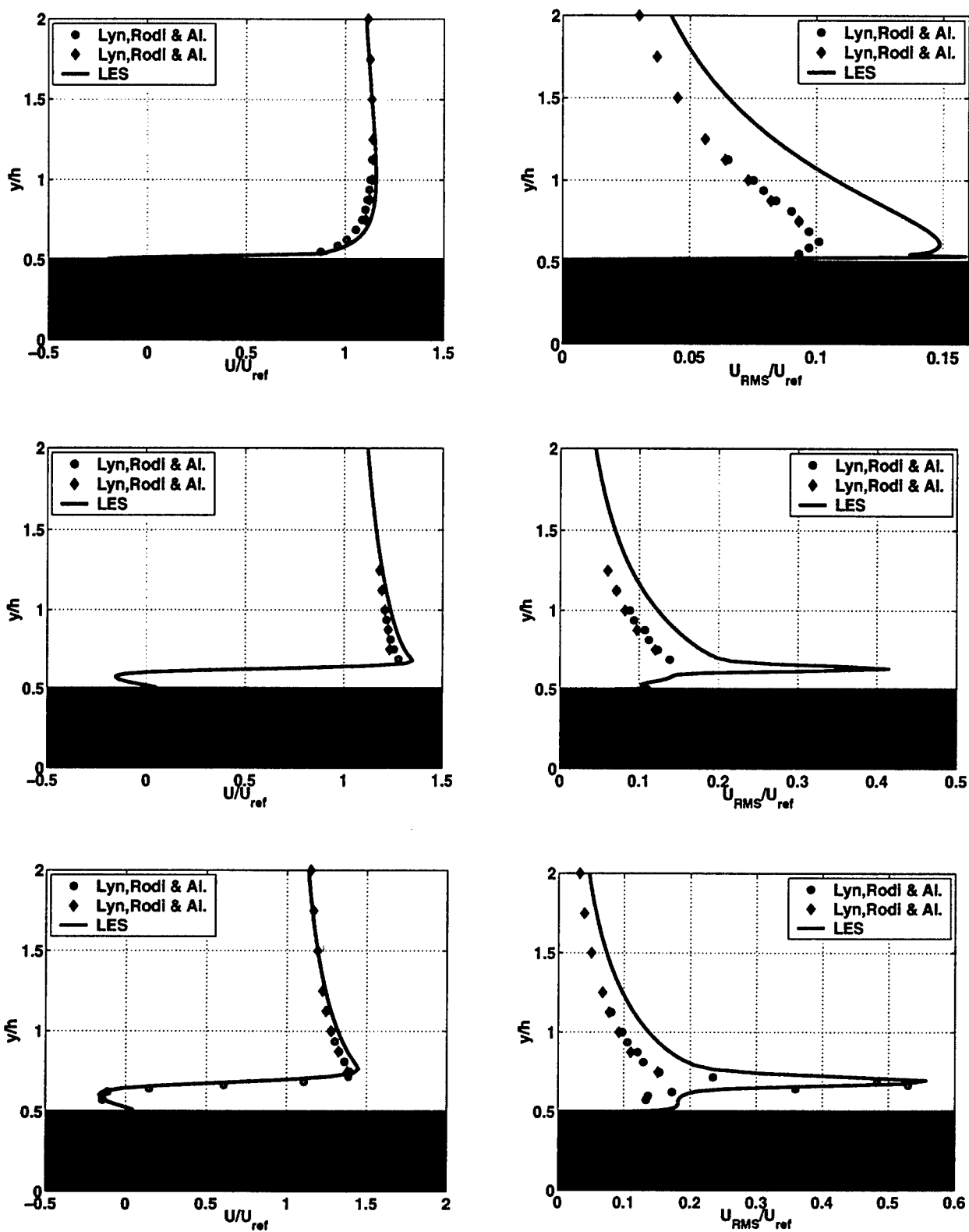
Fig. B.6: Additional simulations, Case I: velocity profiles for stream-wise velocity, left and stream-wise RMS, right, at three stations, from top to bottom: x = -\frac{1}{2H} , x = -\frac{3}{8H} and x = -\frac{1}{4H} .
