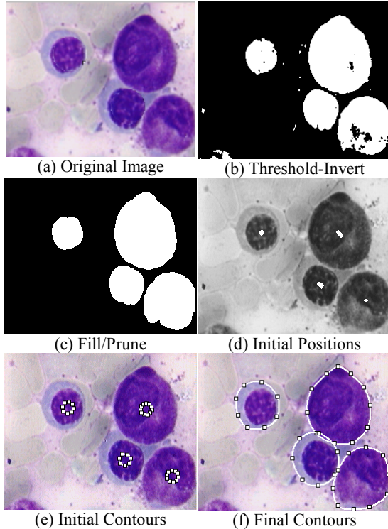
Fig. 2. Segmentation steps.
