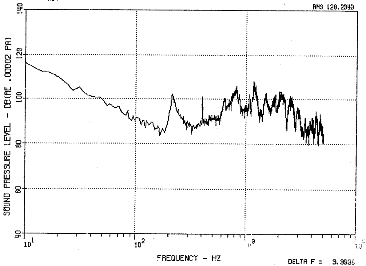
Figure 26. C-130 Fwd Microphone MF, 1000 Ft, 250 Kt, 30 Deg, and 5000 Ft, 250 Kt, 30 Deg.
