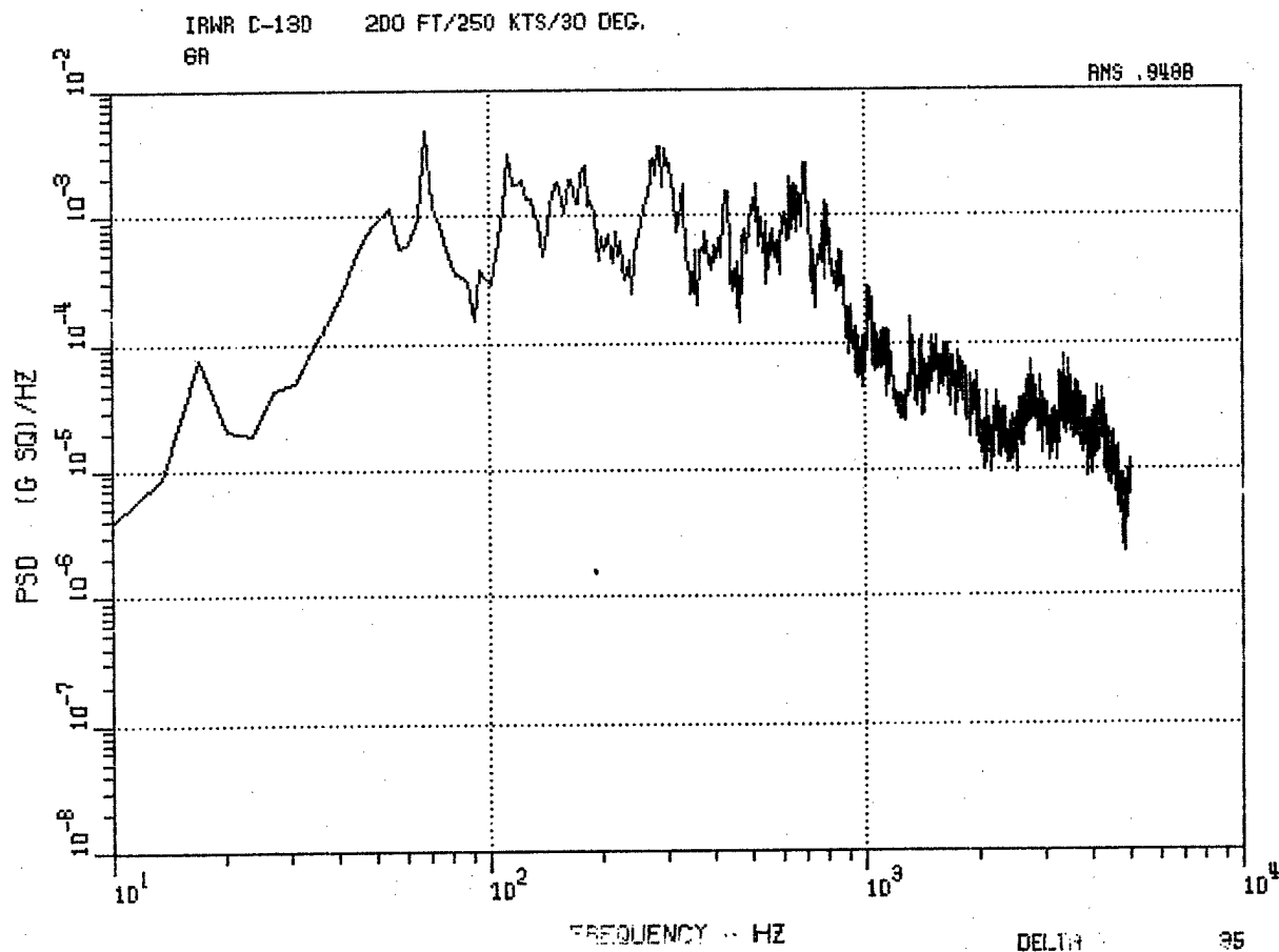
Figure 53. C-130 Aft Longitudinal Accelerometer 6A, 5000 Ft, 130 Kt, 0 Deg, and 200 Ft, 250 Kt, 30 Deg.
