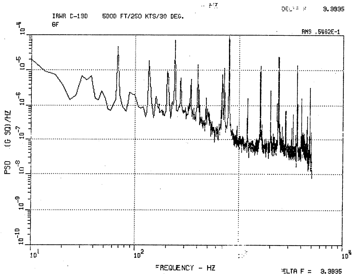
Figure 22. C-130 Fwd Longitudinal Accelerometer 6F, 1000 Ft, 250 Kt, 30 Deg, and 5000 Ft, 250 Kt, 30 Deg.
