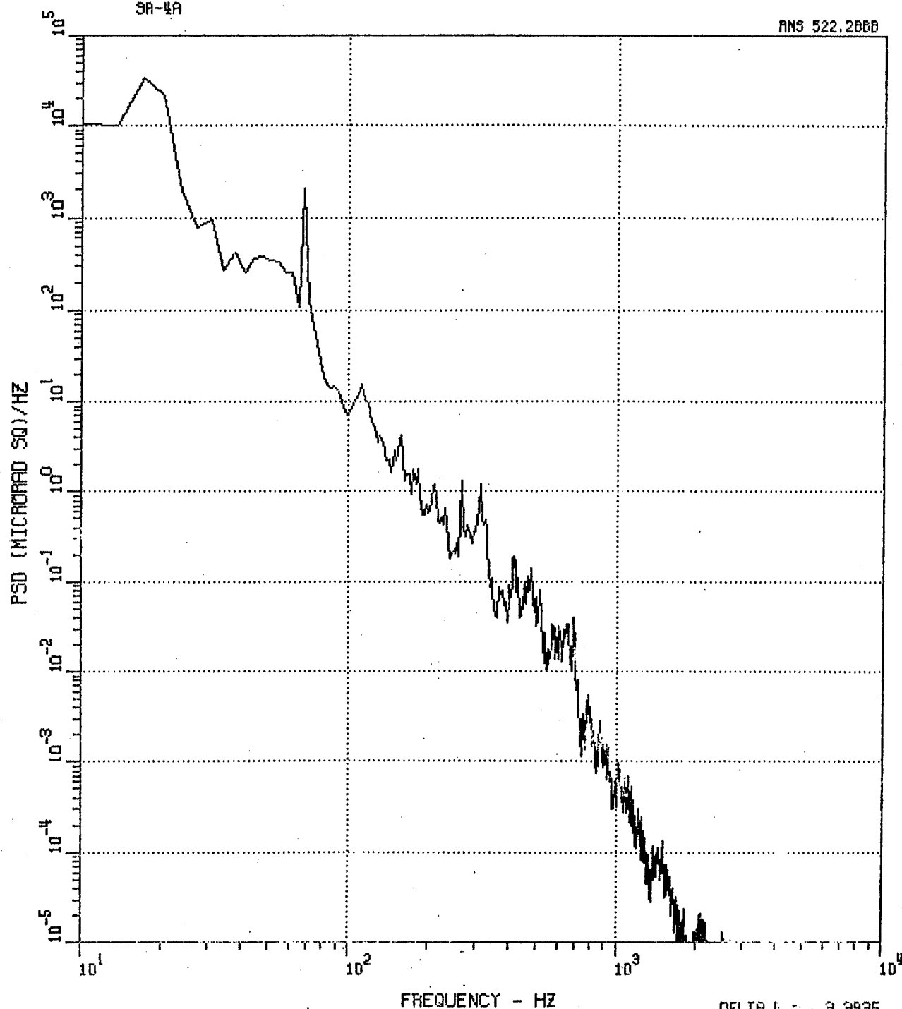
Figure 100. C-130 Aft Pieth PSD, 3A-4A, 1000 Ft, 250 Kt, 30 Deg. DELTA F = 3.9935
