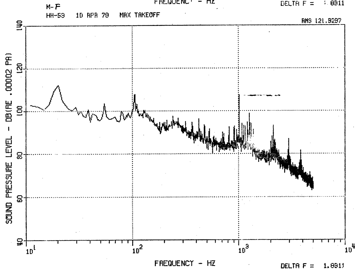
Figure 69. HH-53 Fwd Microphone MF, Hover IGE and Max Takeoff.
