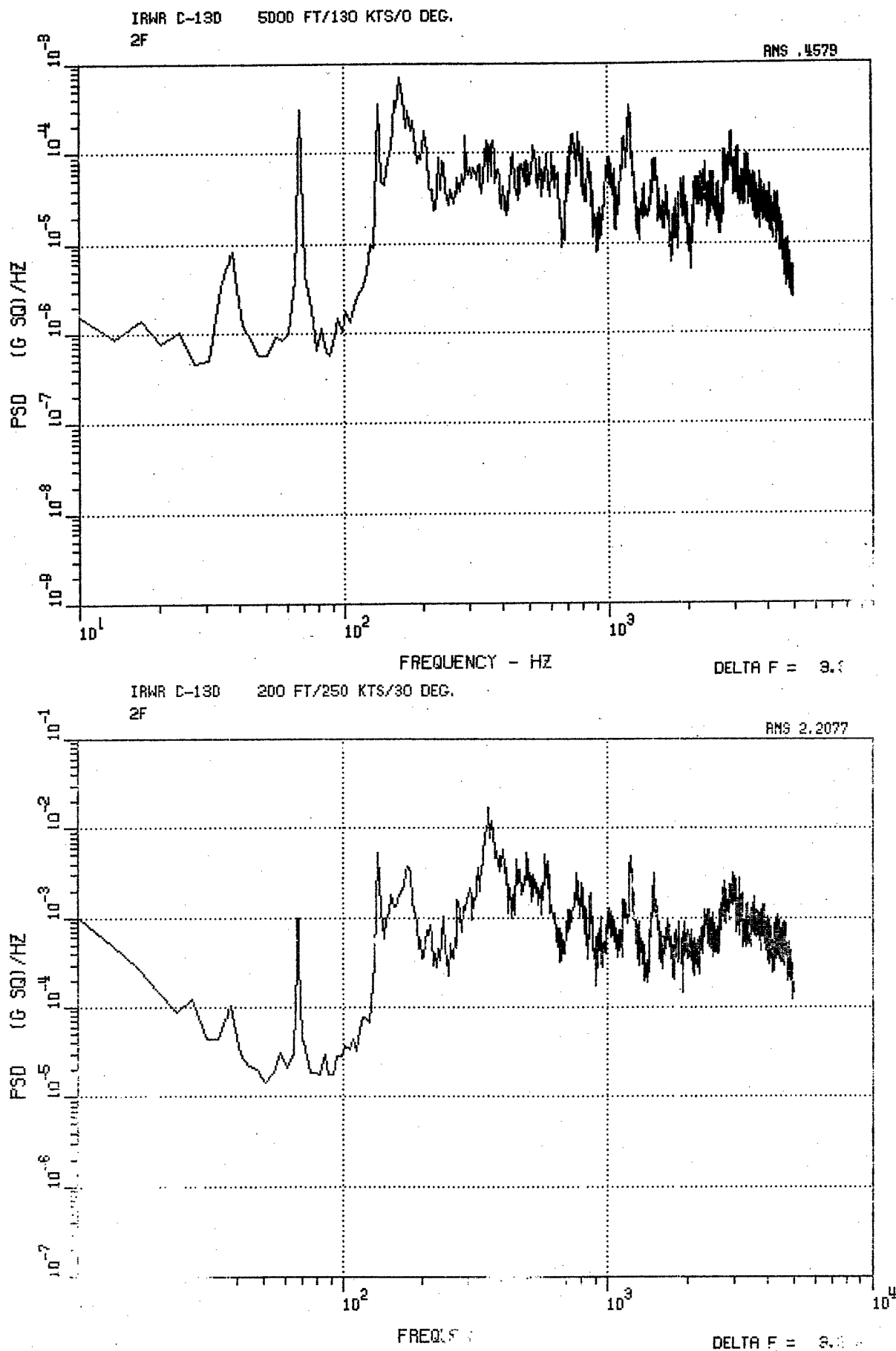
Figure 13. C-130 Fwd Lateral Accelerometer 2F, 5000 Ft, 130 Kt, 0 Deg, and 200 Ft, 250 Kt, 30 Deg.
