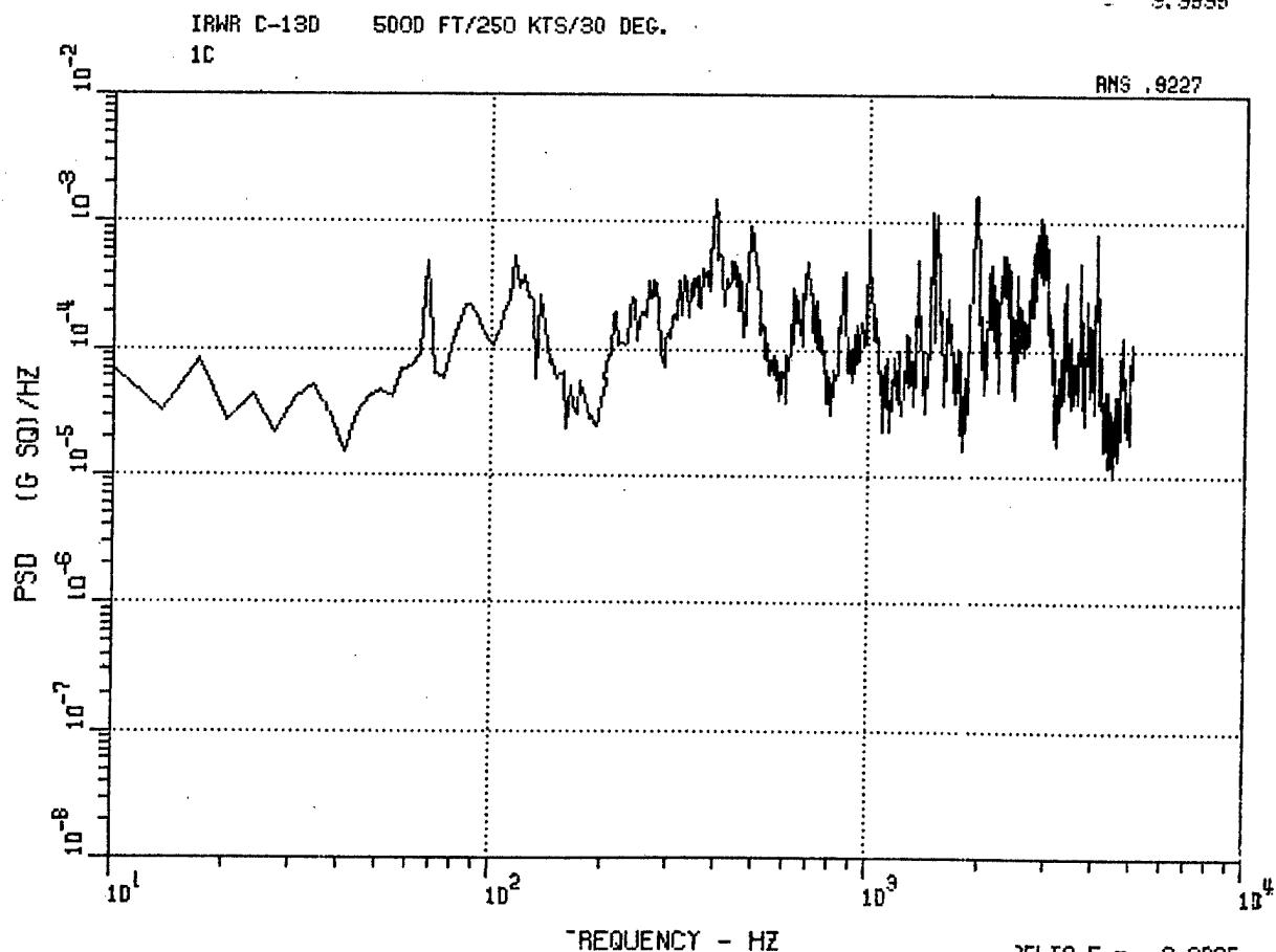
Figure 30. C-130 Center Vertical Accelerometer 1C, 1000 Ft, 250 Kt, 30 Deg, and 5000 Ft, 250 Kt, 30 Deg.
