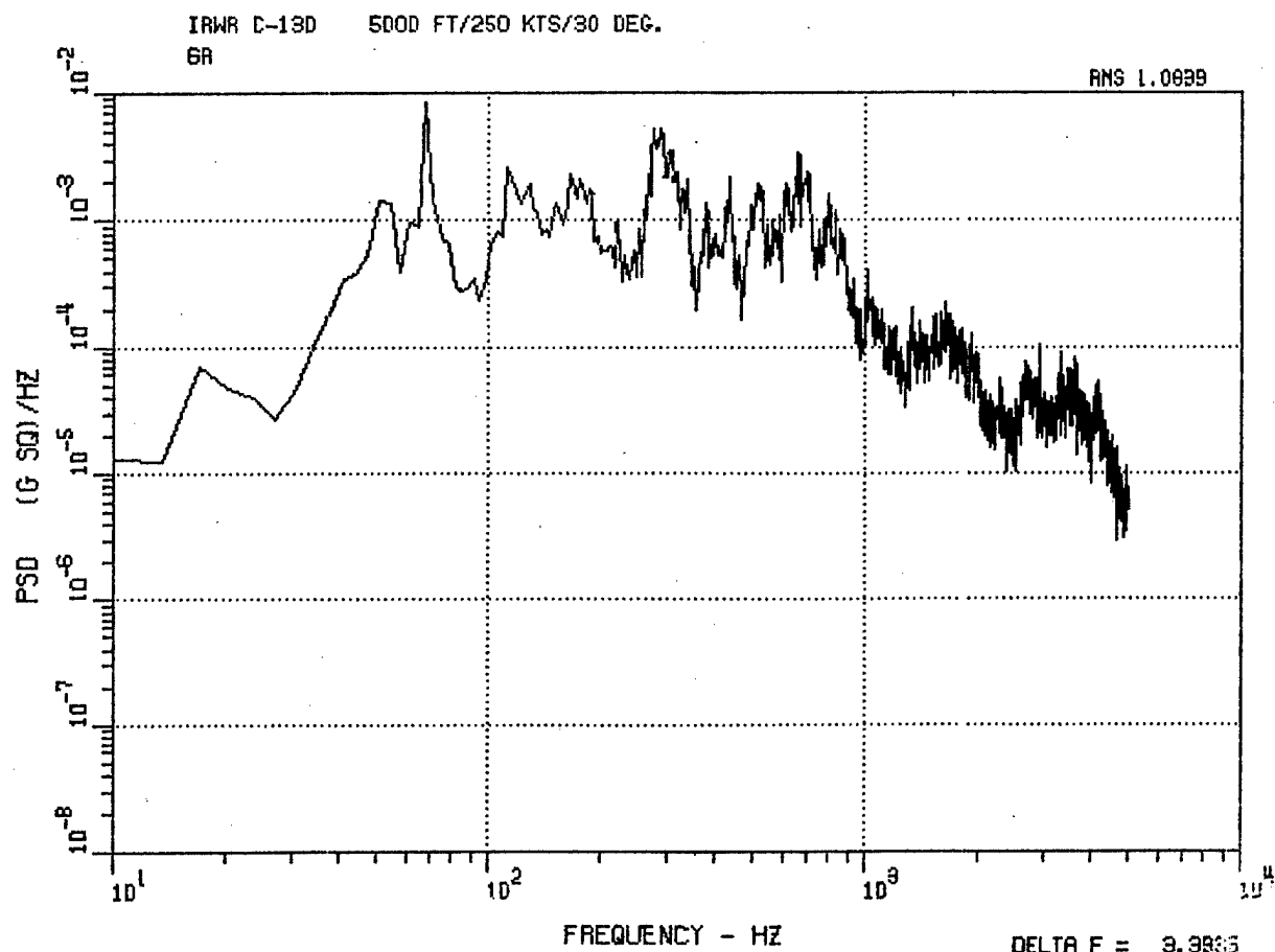
Figure 54. C-130 Aft Longitudinal Accelerometer 6A, 1000 Ft, 250 Kt, 30 Deg, and 5000 Ft, 250 Kt, 30 Deg.
