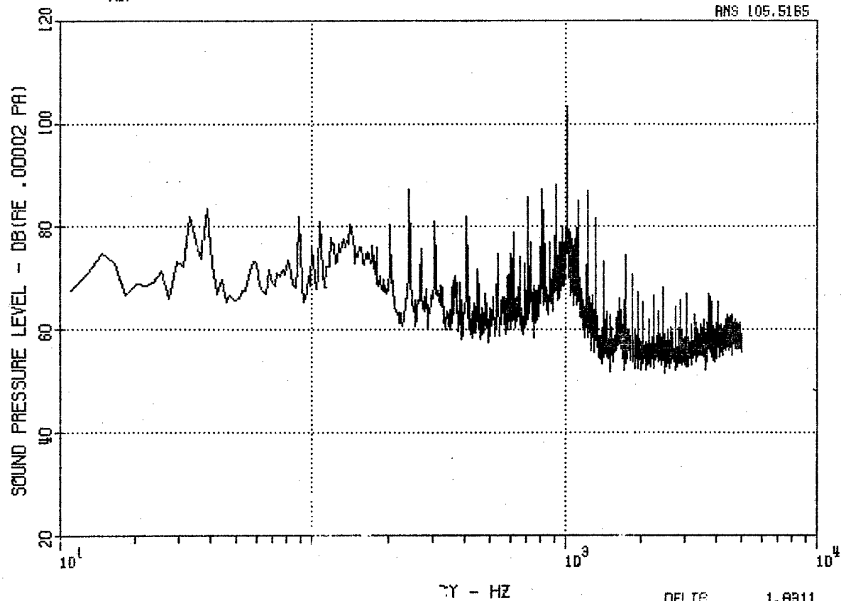
Figure 71. HH-53 Fwd Microphone MF, Autorotation and No-Signal Record.
