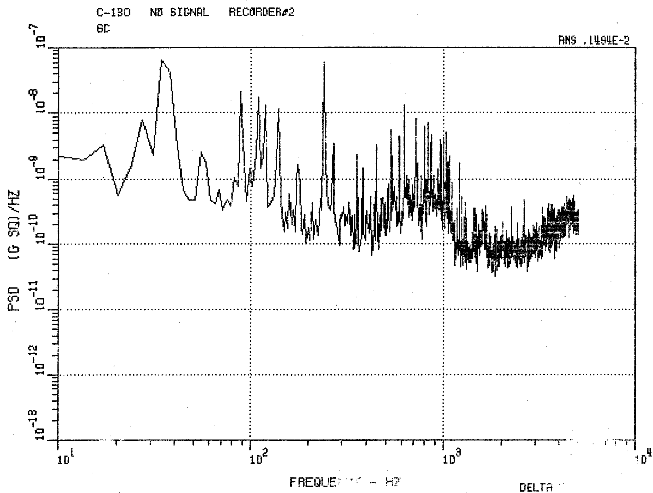
Figure 39. C-130 Center Longitudinal Accelerometer 6C, No-Signal Record.
