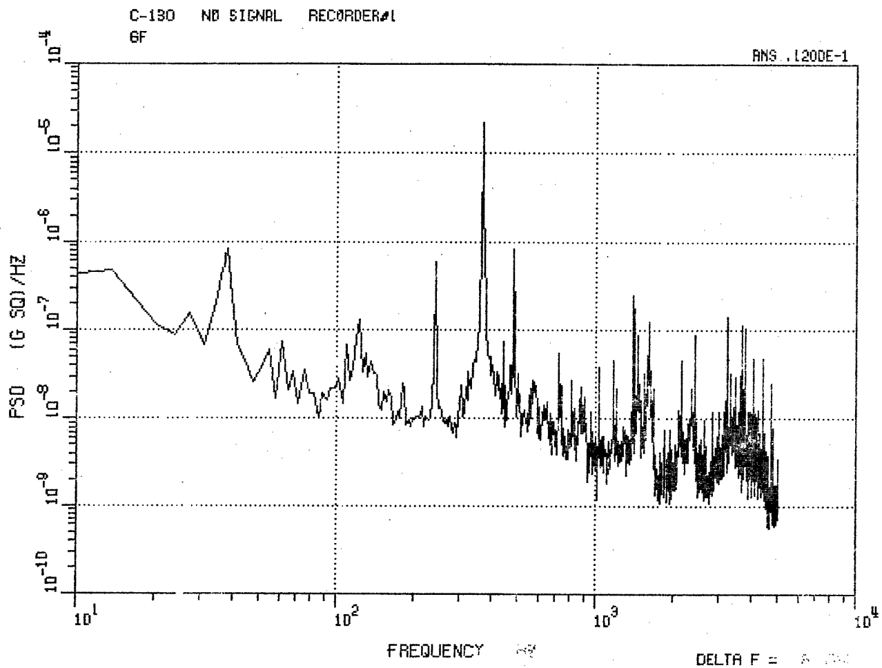
Figure 23. C-130 Fwd Longitudinal Accelerometer 6F, No-Signal Record.
