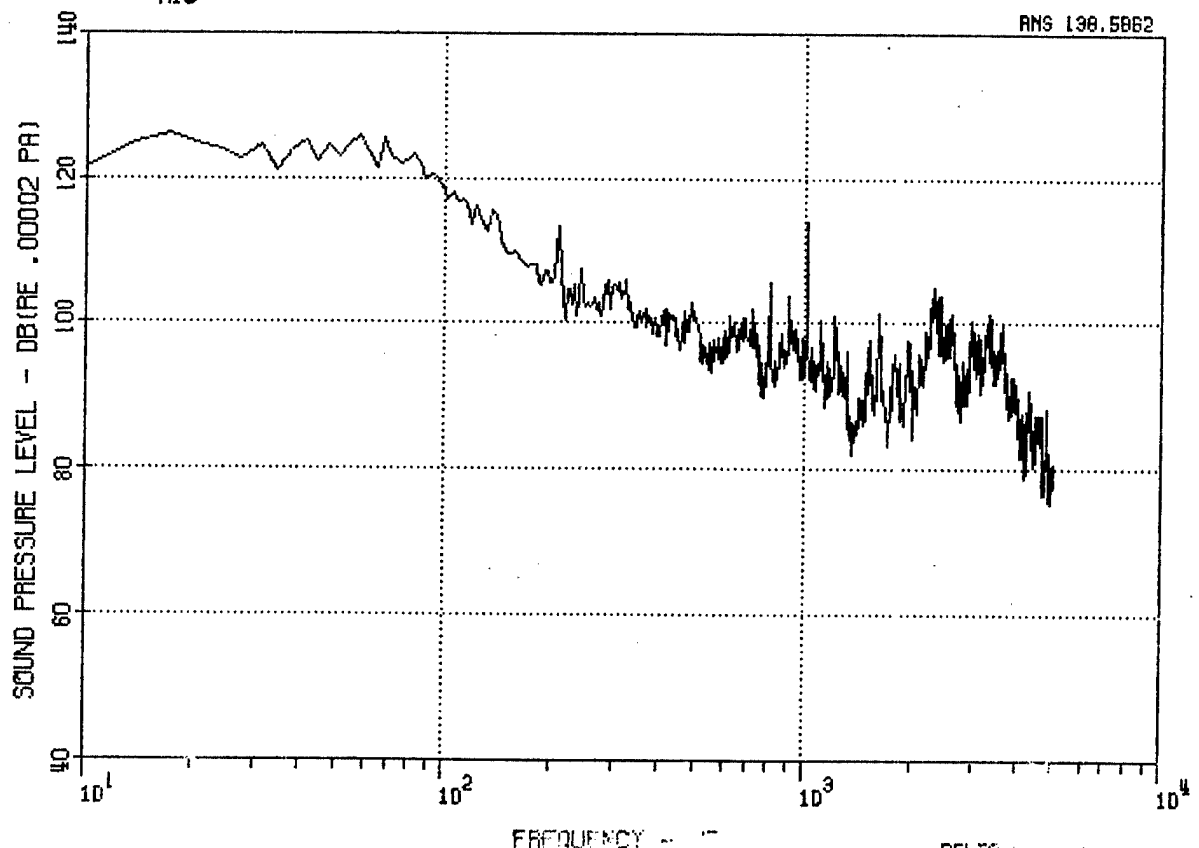
Figure 42. C-130 Center Microphone MC, 1000 Ft, 250 Kt, 30 Deg, and 5000 Ft, 250 Kt, 30 Deg.
