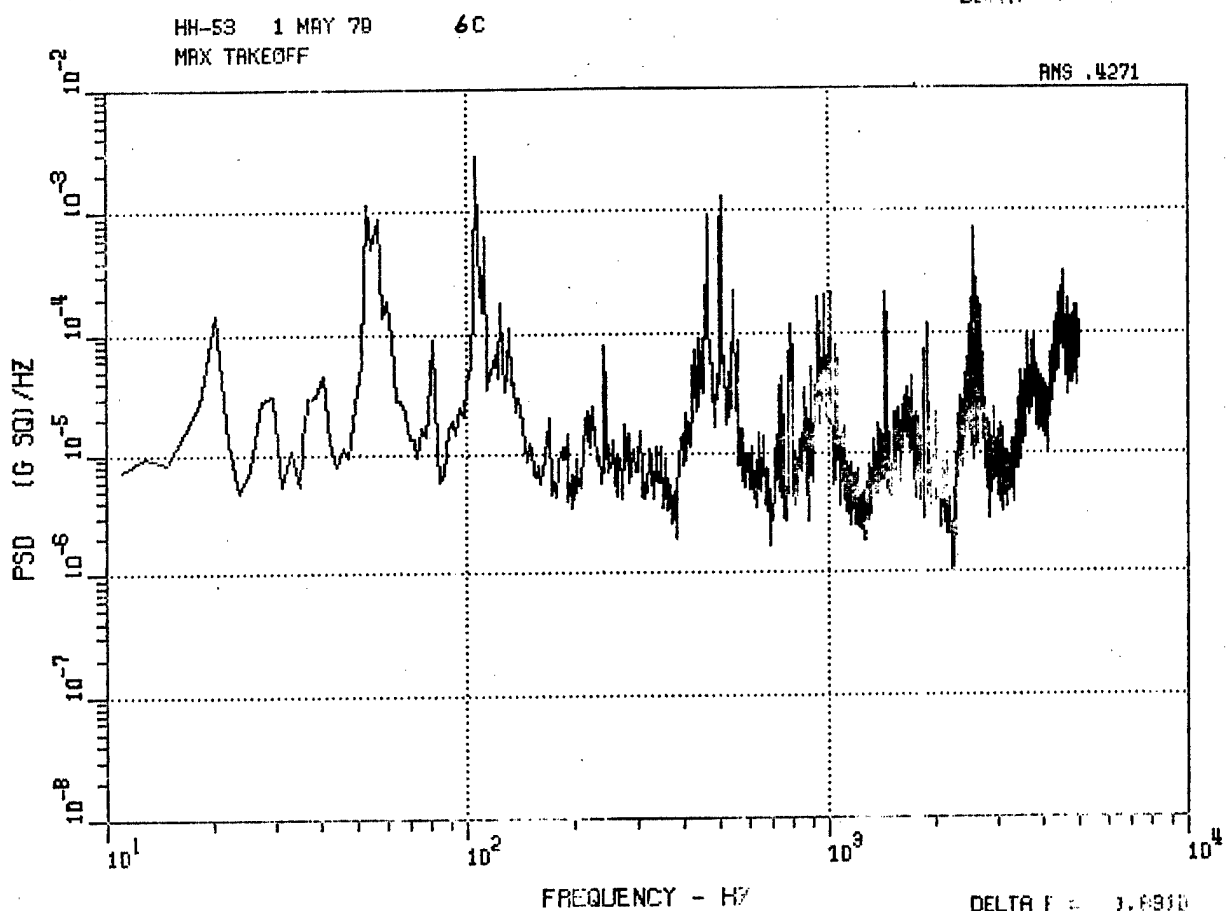
Figure 78. HH-53 Center Longitudinal Accelerometer 6C, Hover IGE and Max Takeoff.
