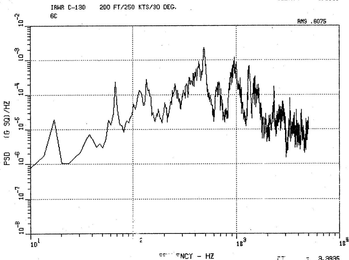
Figure 37. C-130 Center Longitudinal Accelerometer 6C, 5000 Ft, 130 Kt, 0 Deg, and 200 Ft, 250 Kt, 30 Deg.
