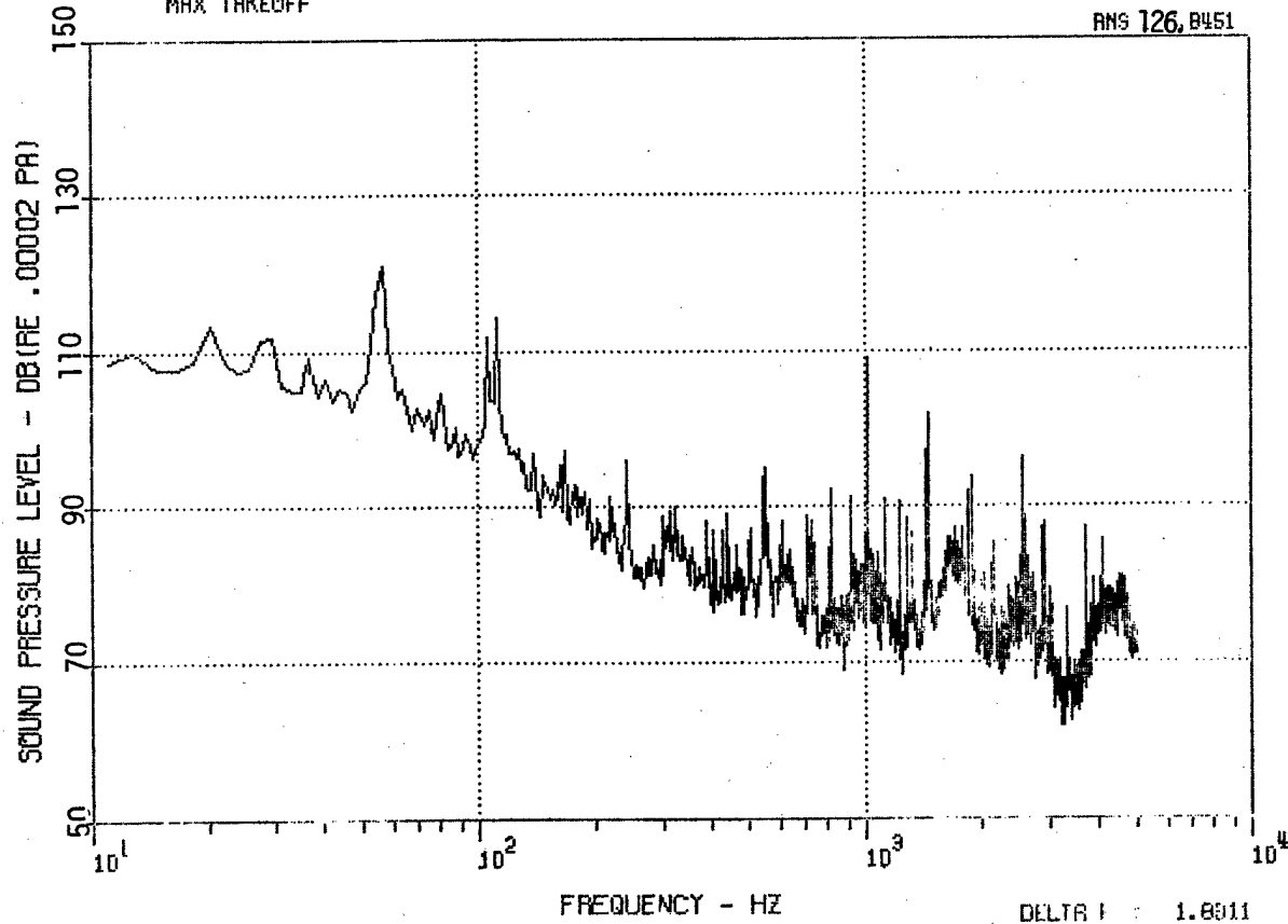
Figure 81. HH-53 Center Microphone MC, Hover IGE and Max Takeoff.
