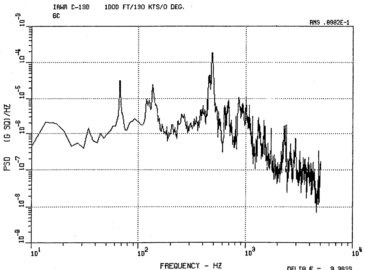
Figure 36. C-130 Center Longitudinal Accelerometer 6C, 200 Ft, 130 Kt, 0 Deg, and 1000 Ft, 130 Kt, 0 Deg.
