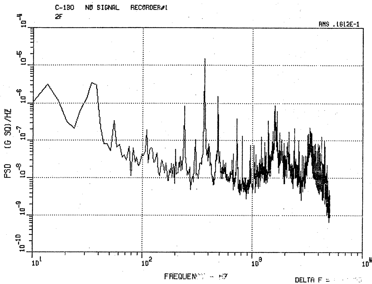
Figure 15. C-130 Fwd Lateral Accelerometer 2F, No-Signal Record.
