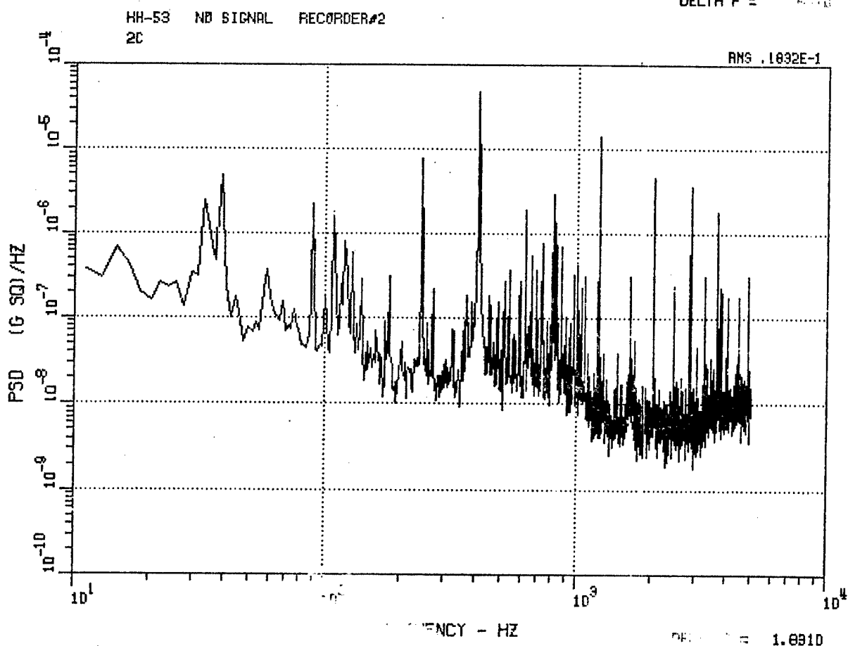
Figure 74. HH-53 Center Vertical Accelerometer 2C, Autorotation and No-Signal Record.
