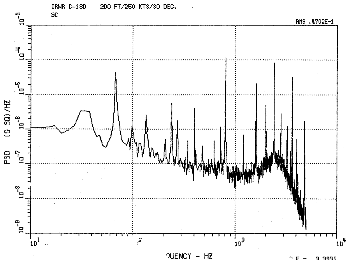
Figure 33. C-130 Center Lateral Accelerometer 3C, 5000 Ft, 130 Kt, 0 Deg, and 200 Ft, 250 Kt, 30 Deg.
