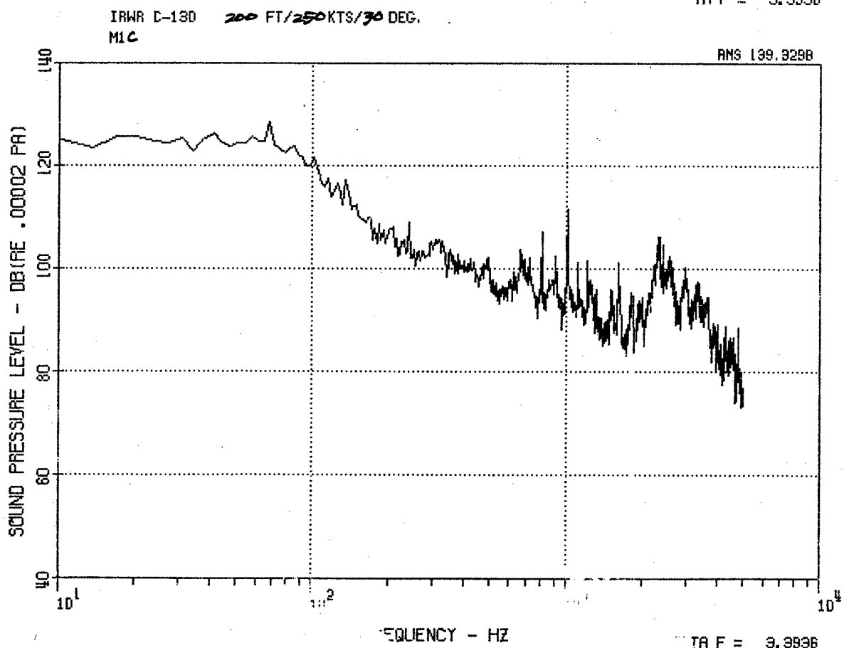
Figure 41. C-130 Center Microphone MC, 5000 Ft, 130 Kt, 0 Deg, and 200 Ft, 250 Kt, 30 Deg.
