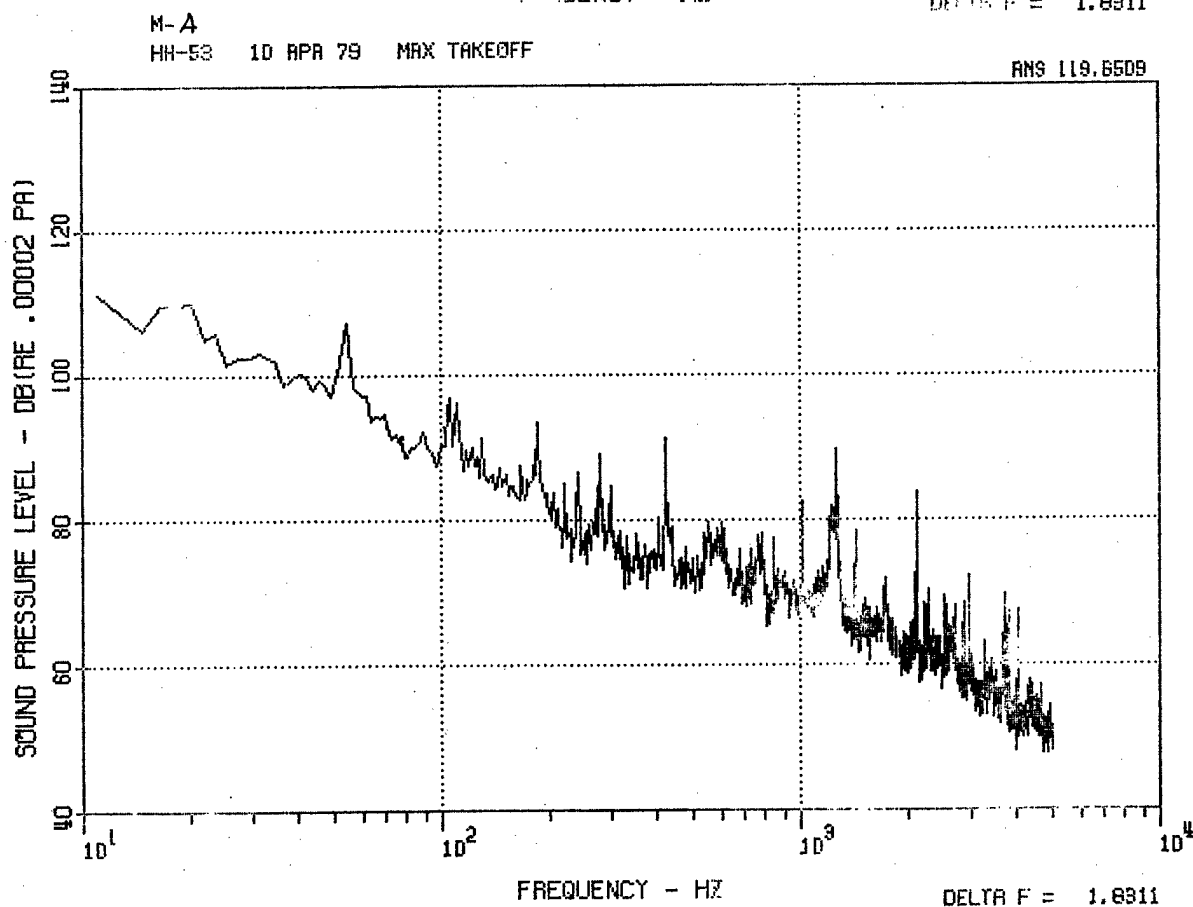
Figure 93. HH-53 Aft Microphone MA, Hover IGE and Max Takeoff.
