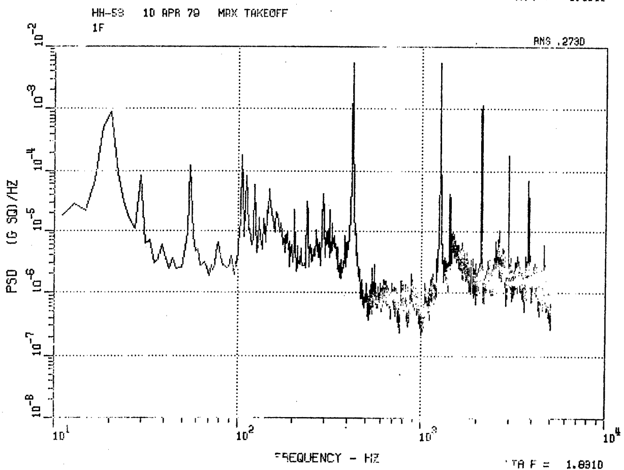
Figure 60. HH-53 Fwd Lateral Accelerometer 1F, Hover IGE and Max Takeoff.
