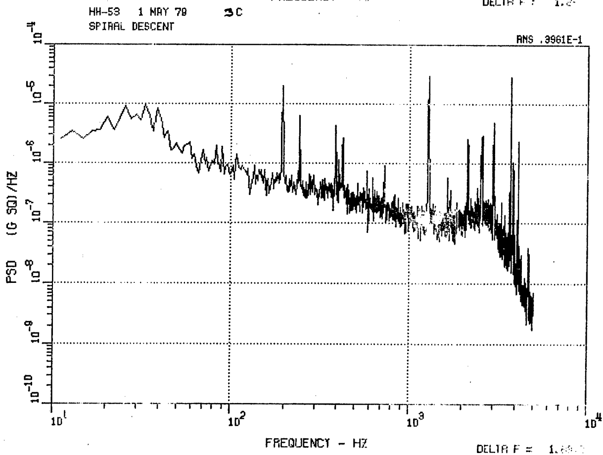
Figure 76. HH-53 Center Lateral Accelerometer 3C, Cruise and Spiral Descent.
