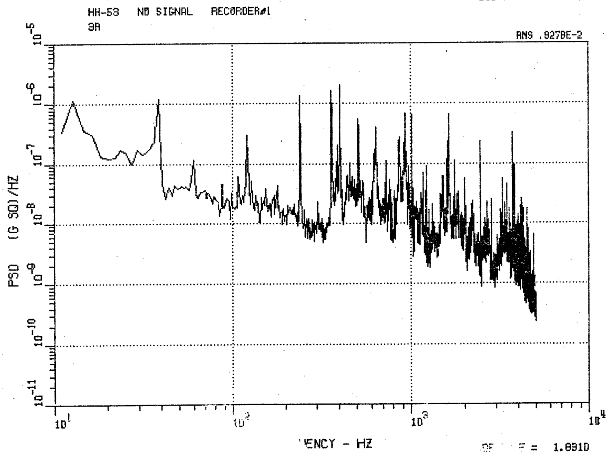
Figure 89. HH-53 Aft Vertical Accelerometer 3A, Autorotation and No-Signal Record.
