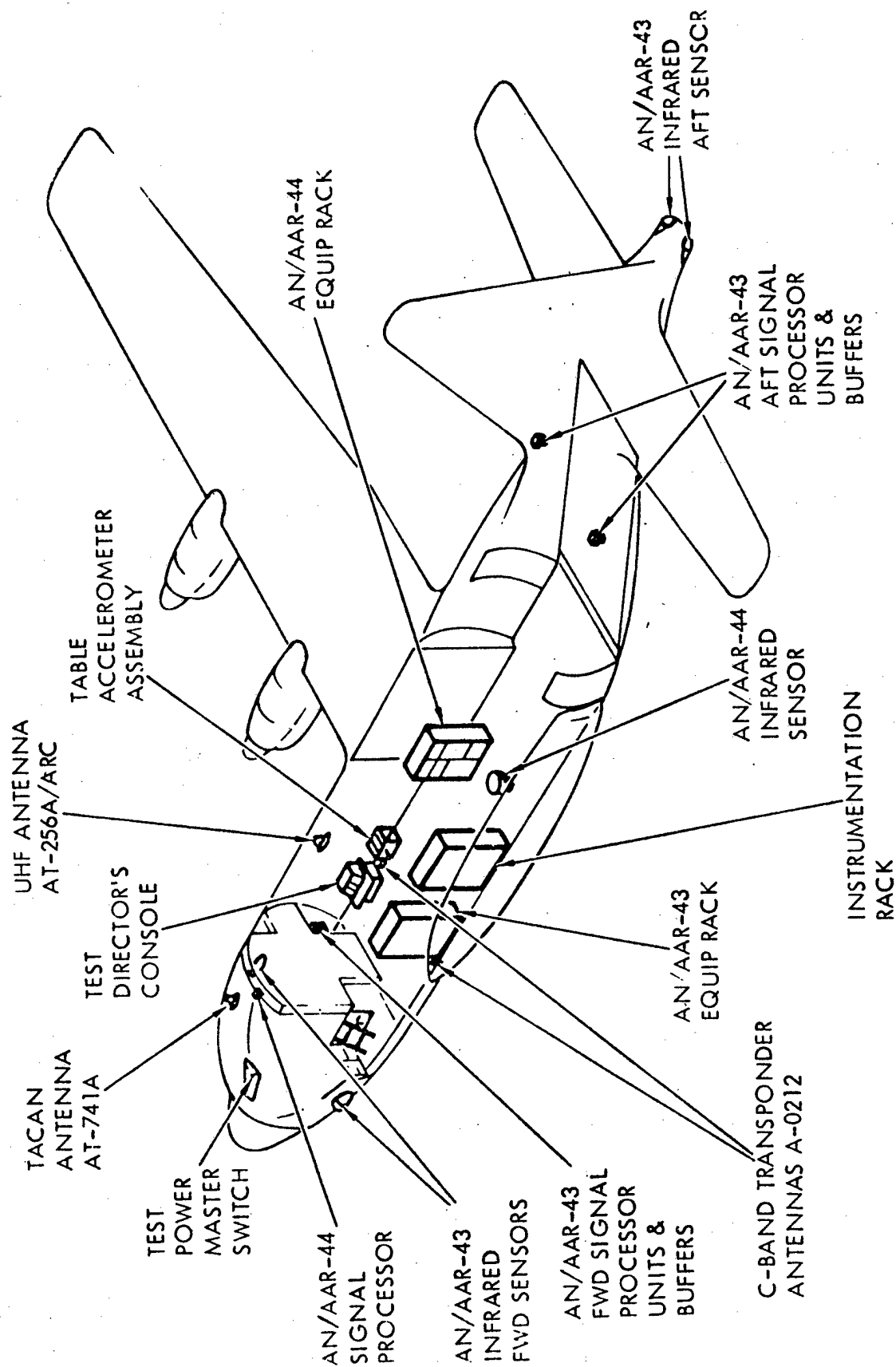
Figure 1. C-130E Installation.
