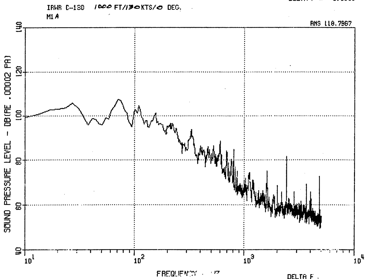
Figure 56. C-130 Aft Microphone MA, 200 Ft, 130 Kt, 0 Deg, and 1000 Ft, 130 Kt, 0 Deg.
