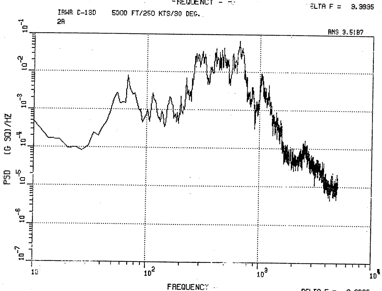
Figure 46. C-130 Aft Lateral Accelerometer 2A, 1000 Ft, 250 Kt, 30 Deg, and 5000 Ft, 250 Kt, 30 Deg.
