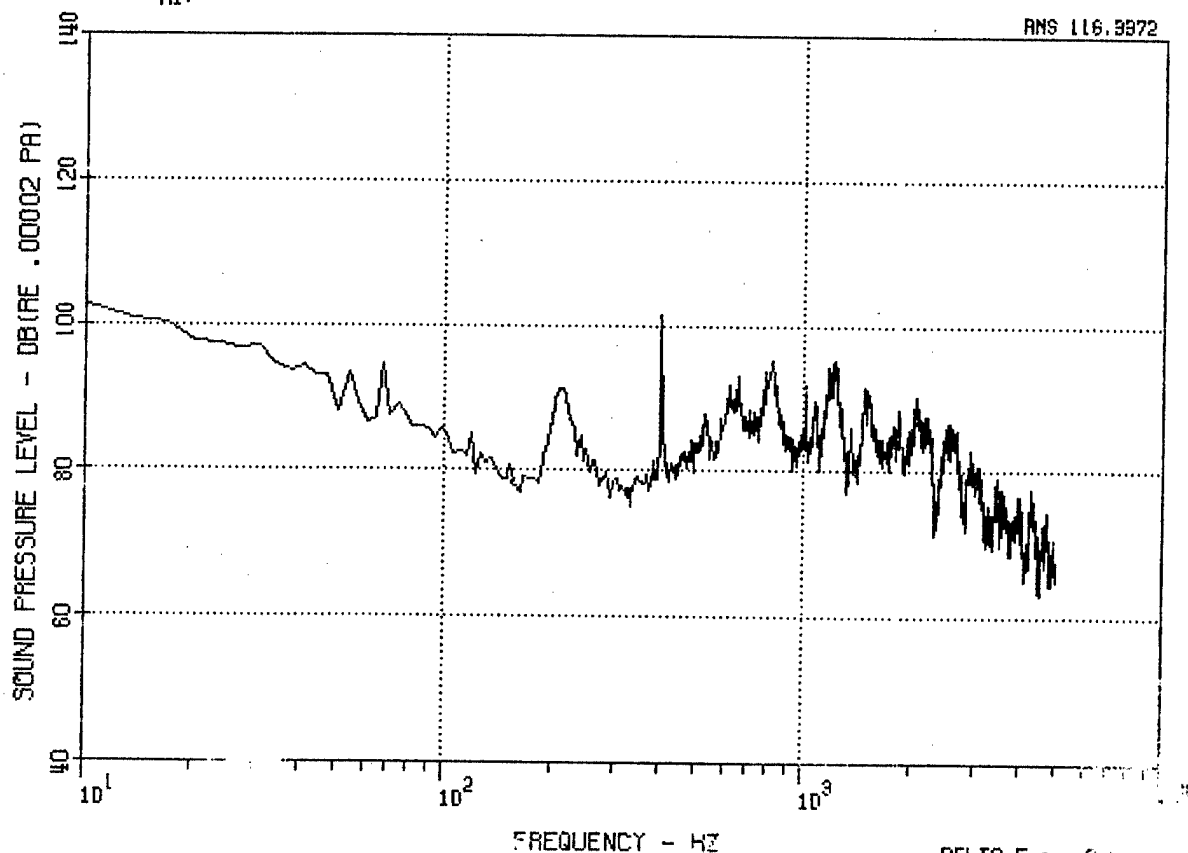
Figure 24. C-130 Fwd Microphone MF, 200 Ft, 130 Kt, 0 Deg, and 1000 Ft, 130 Kt, 0 Deg.
