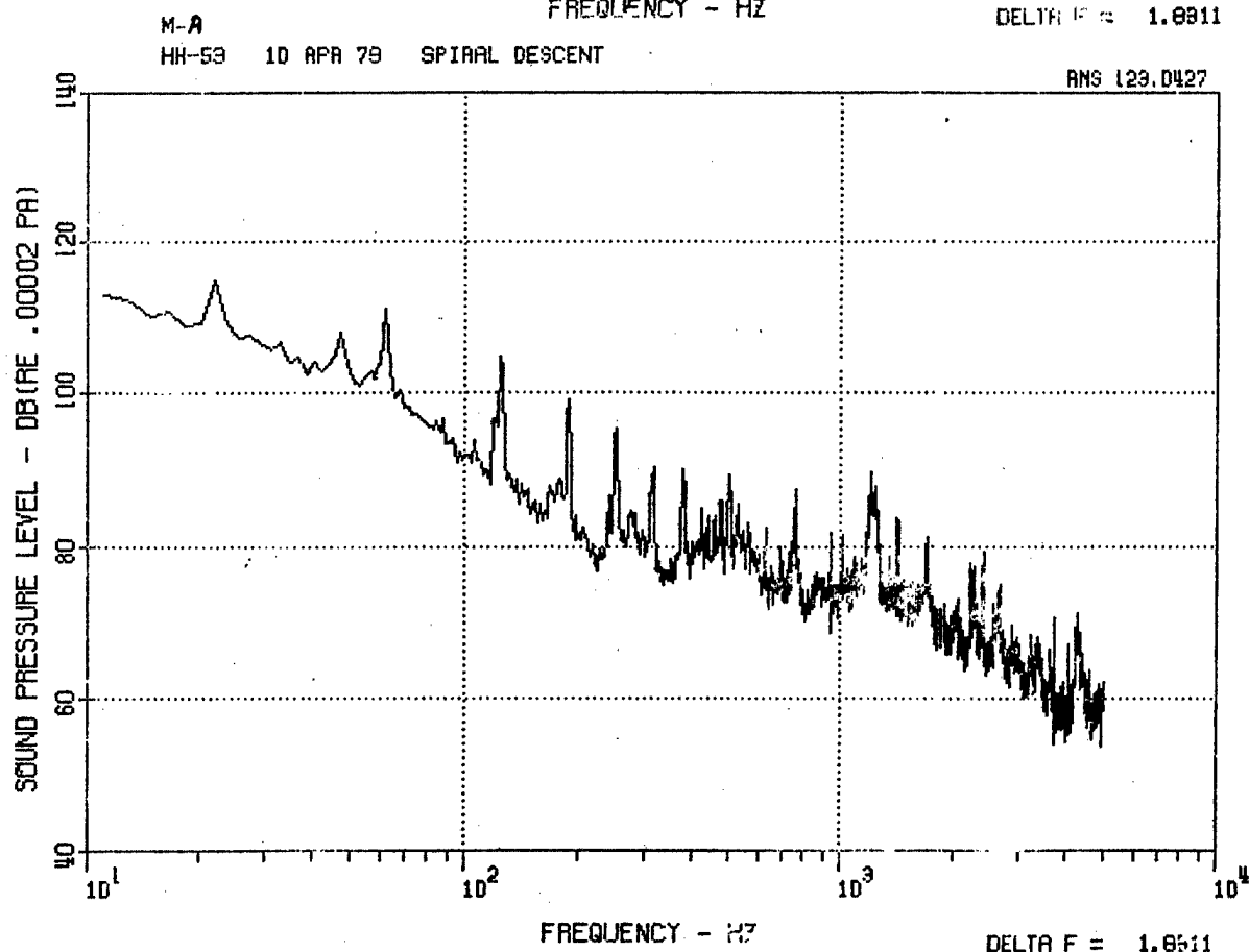
Figure 94. HH-53 Aft Microphone MA, Cruise and Spiral Descent.
