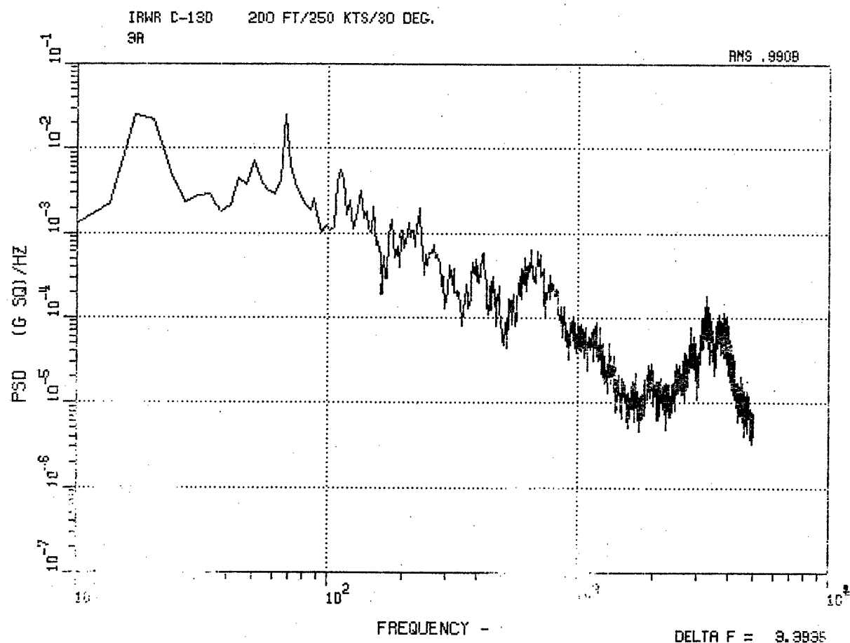
Figure 49. C-130 Aft Vertical Accelerometer 3A, 5000 Ft, 130 Kt, 0 Deg, and 200 Ft, 250 Kt, 30 Deg.
