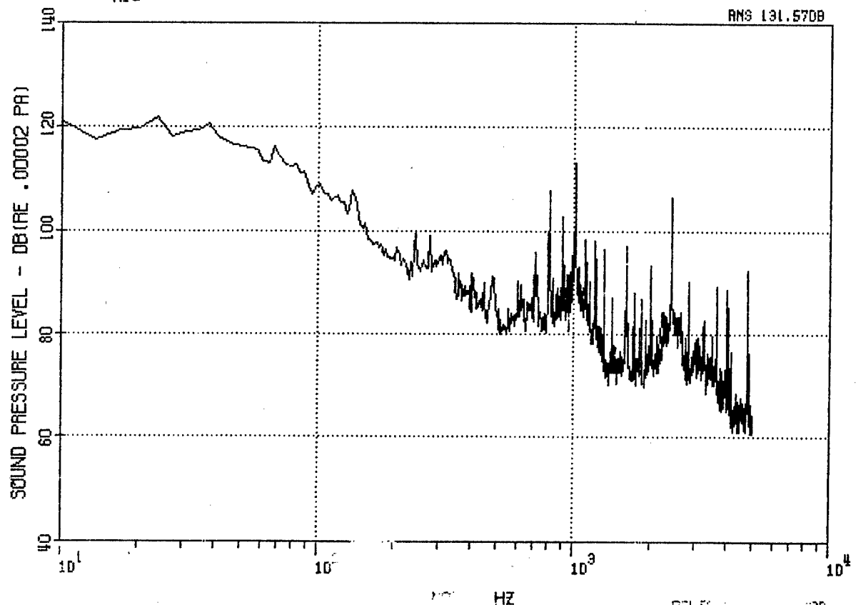
Figure 40. C-130 Center Microphone MC, 200 Ft, 130 Kt, 0 Deg, and 1000 Ft, 130 Kt, 0 Deg.
