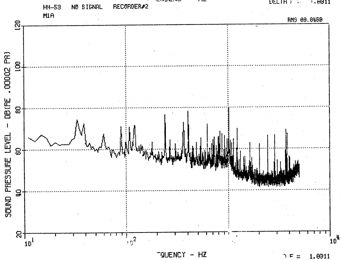
Figure 95. HH-53 Aft Microphone MA, Autorotation and No-Signal Record.
