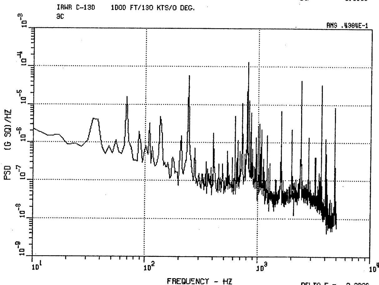
Figure 32. C-130 Center Lateral Accelerometer 3C, 200 Ft, 130 Kt, 0 Deg, and 1000 Ft, 130 Kt, 0 Deg.
