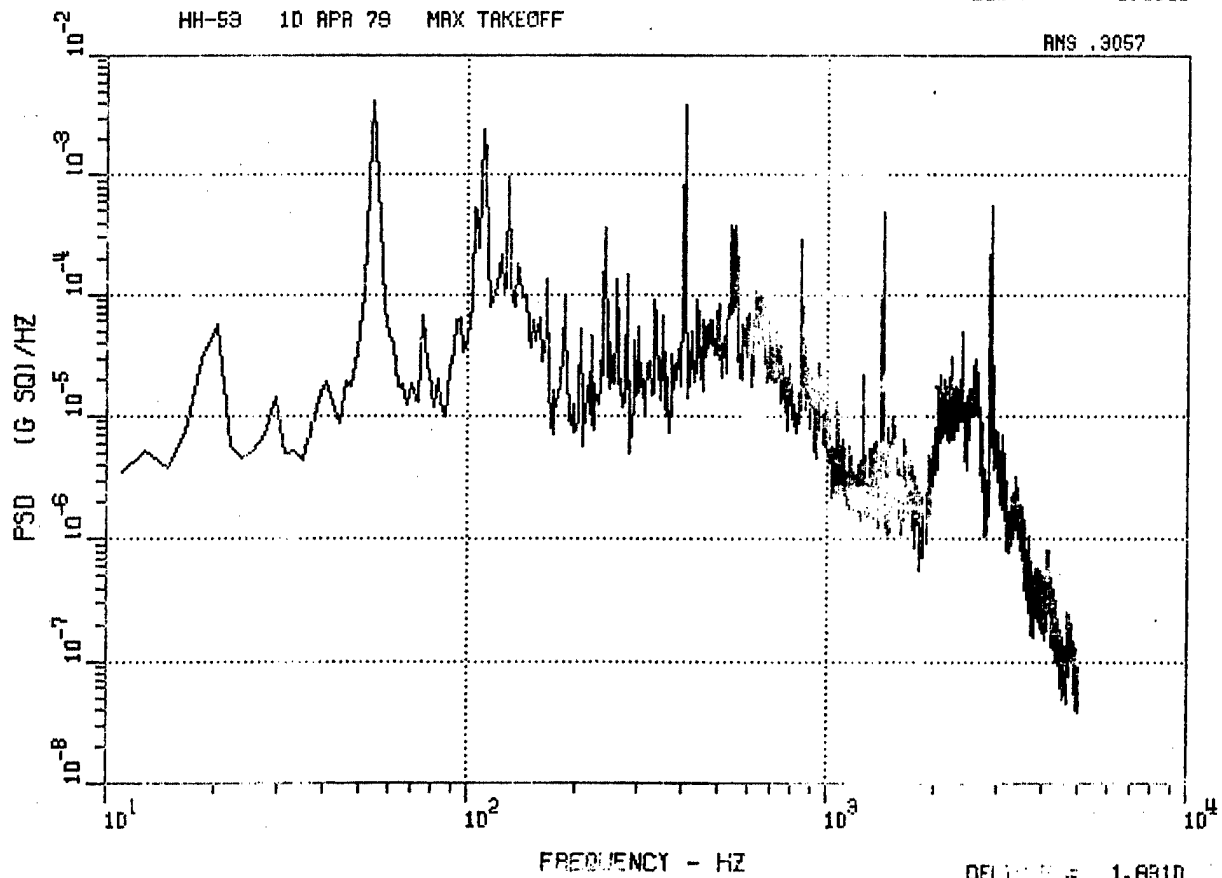
Figure 90. HH-53 Aft Longitudinal Accelerometer 6A, Hover IGE and Max Takeoff.
