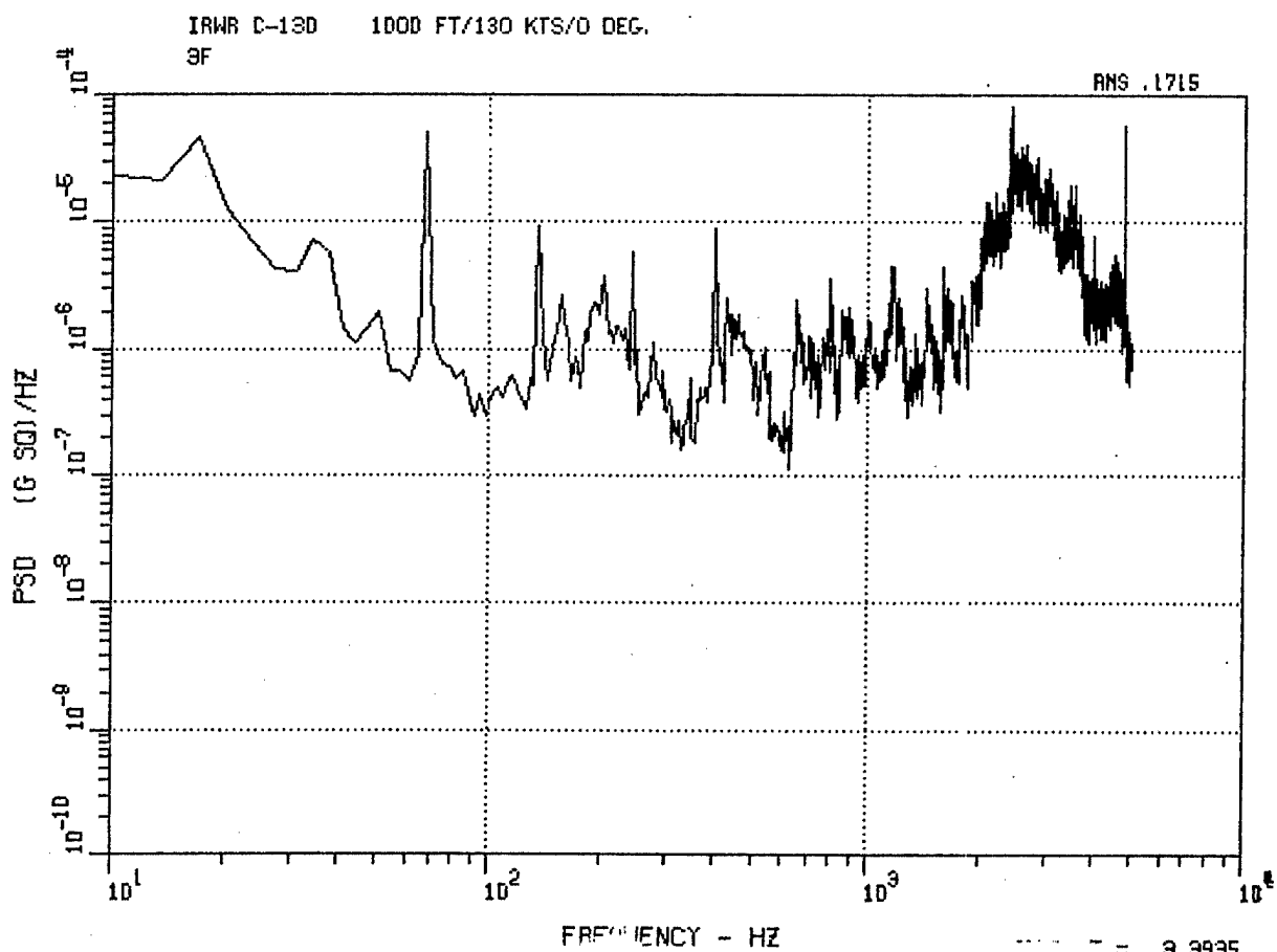
Figure 16. C-130 Fwd Vertical Accelerometer 3F, 200 Ft, 130 Kt, 0 Deg, and 1000 Ft, 130 Kt, 0 Deg.
