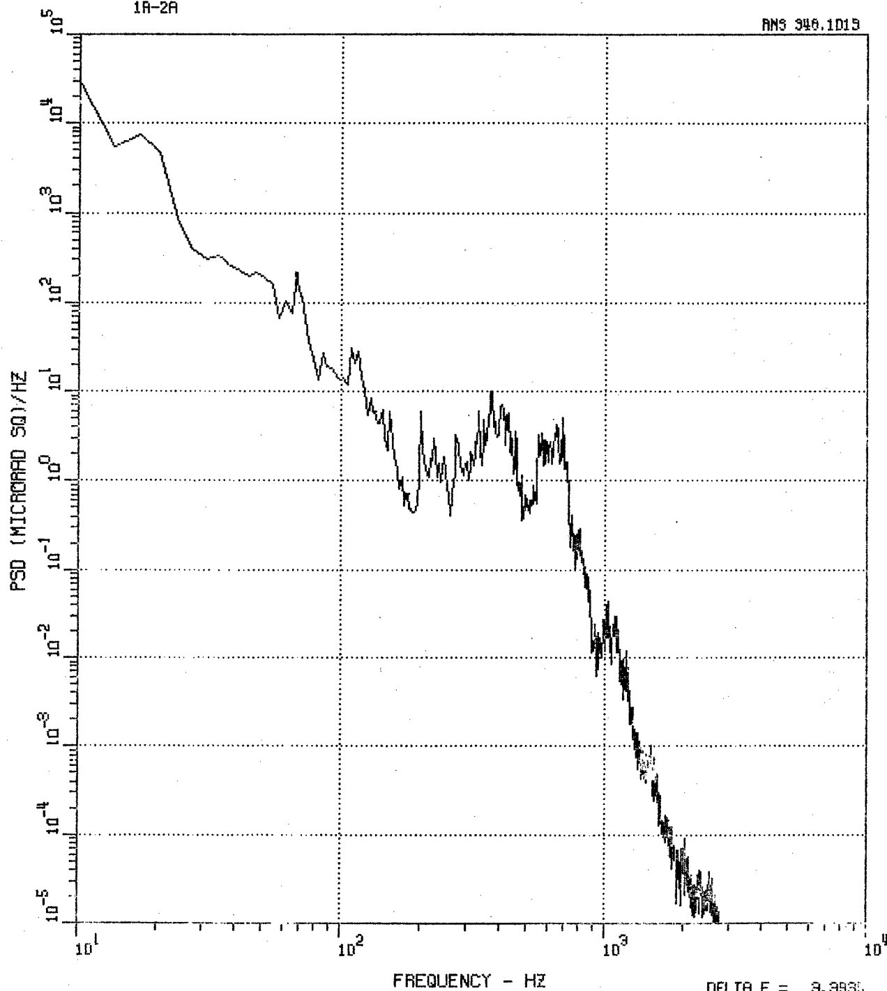
Figure 99. C-130 Aft Roll PSD, 1A-2A, 1000 Ft, 250 Kt, 30 Deg. DELTA F = 3.9835
