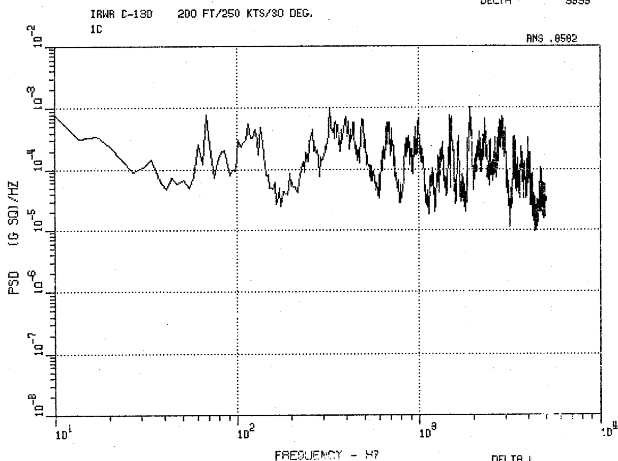
Figure 29. C-130 Center Vertical Accelerometer 1C, 5000 Ft, 130 Kt, 0 Deg, and 200 Ft, 250 Kt, 30 Deg.
