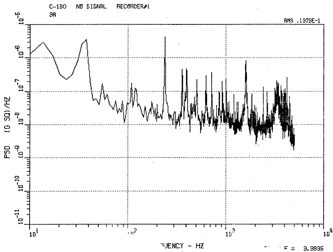
Figure 51. C-130 Aft Vertical Accelerometer 3A, No-Signal Record.
