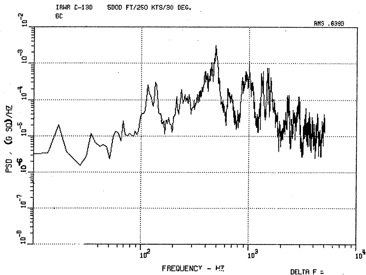
Figure 38. C-130 Center Longitudinal Accelerometer 6C, 1000 Ft, 250 Kt, 30 Deg, and 5000 Ft, 250 Kt, 30 Deg.
