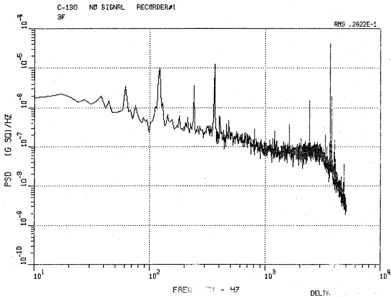
Figure 19. C-130 Fwd Vertical Accelerometer 3F, No-Signal Record.
