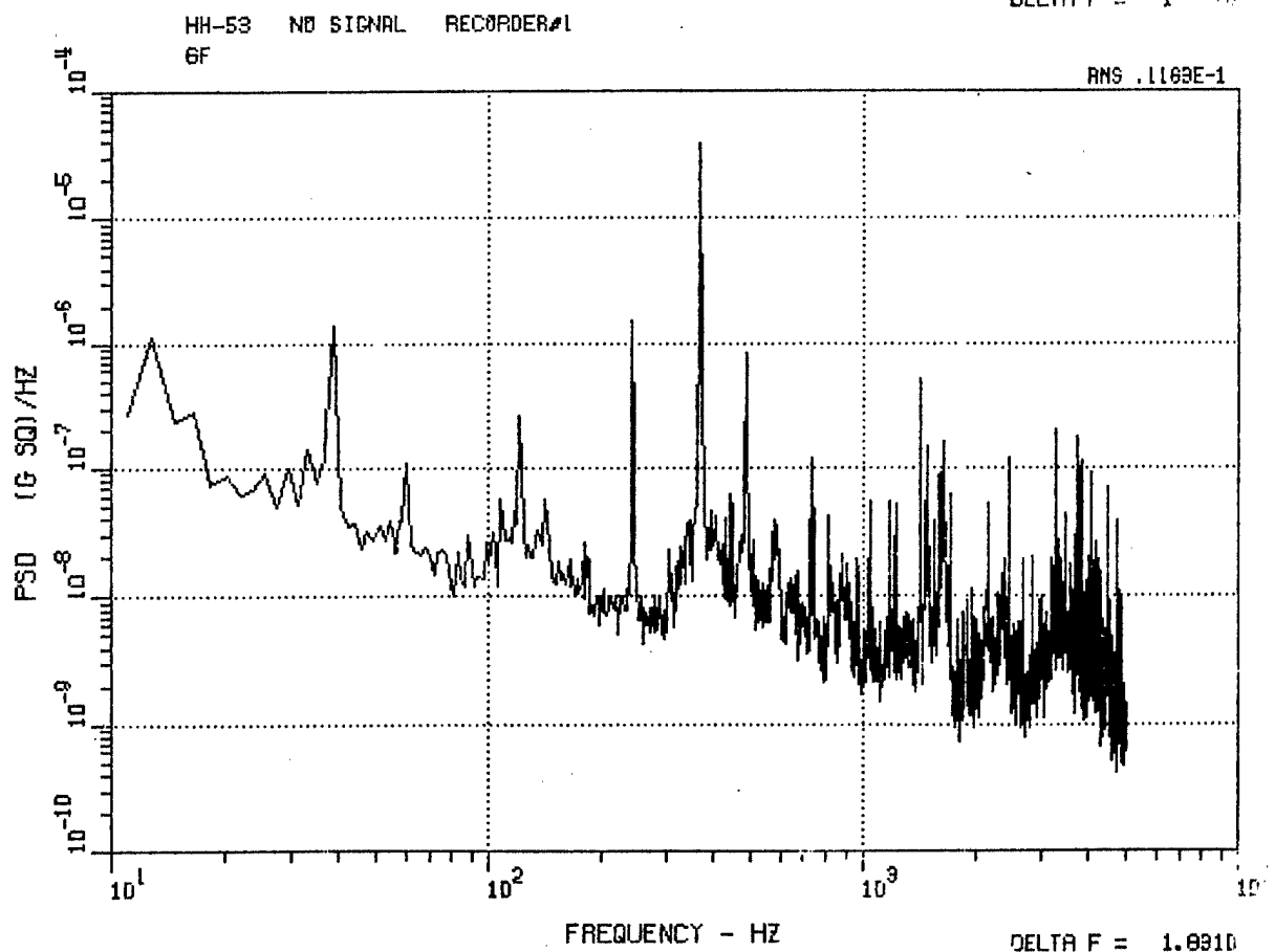
Figure 68. HH-53 Fwd Longitudinal Accelerometer 6F, Autorotation and No-Signal Record.
