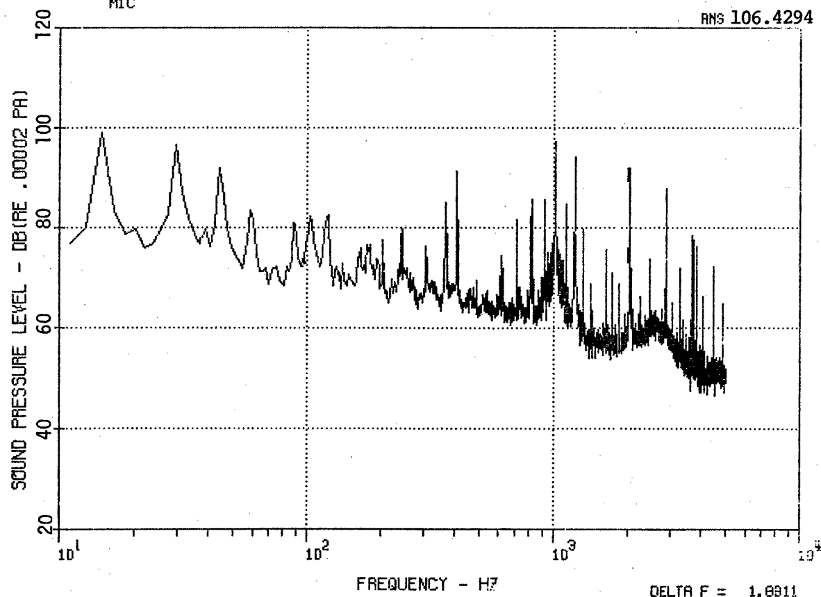
Figure 83. HH-53 Center Microphone MC, Autorotation and No-Signal Record.
