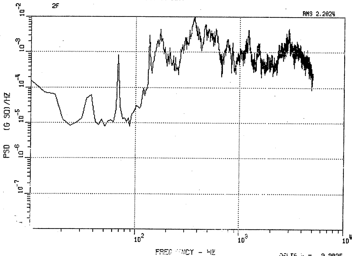
Figure 14. C-130 Fwd Lateral Accelerometer 2F, 1000 Ft, 250 Kt, 30 Deg, and 5000 Ft, 250 Kt, 30 Deg.
