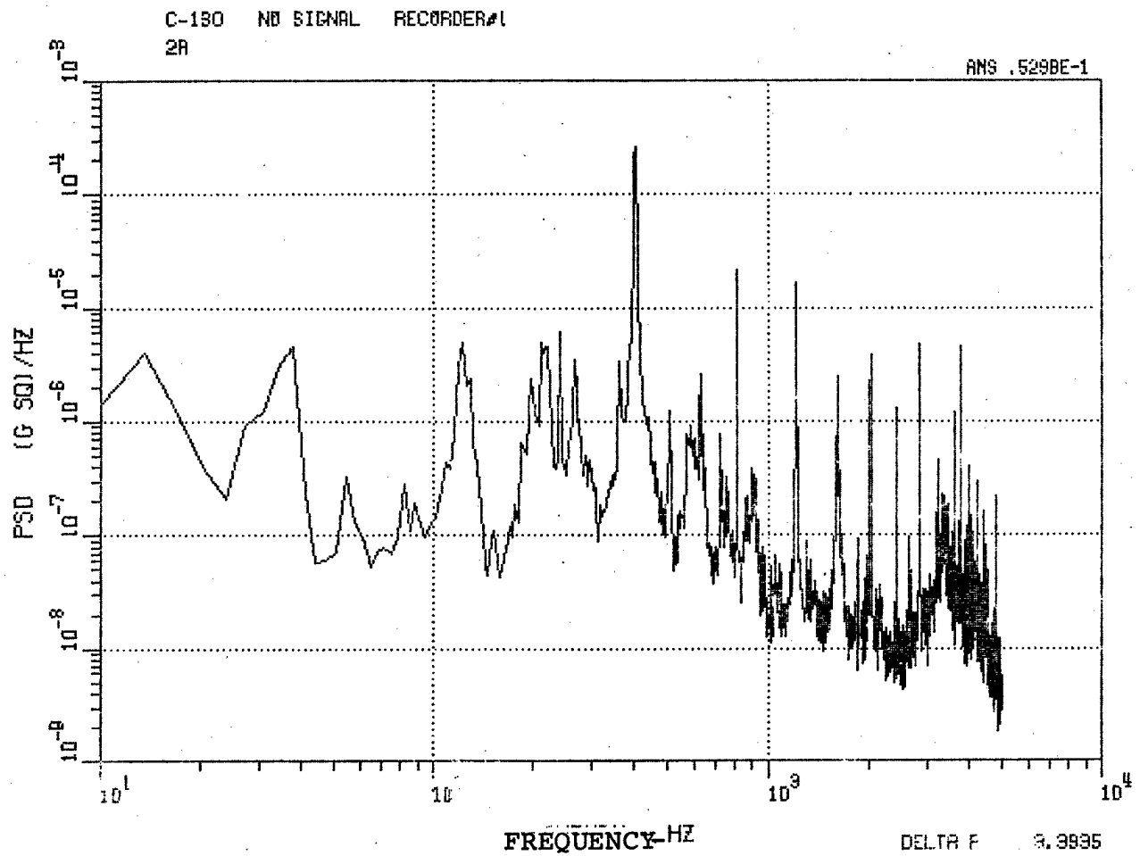
Figure 47. C-130 Aft Lateral Accelerometer 2A, No-Signal Record.
