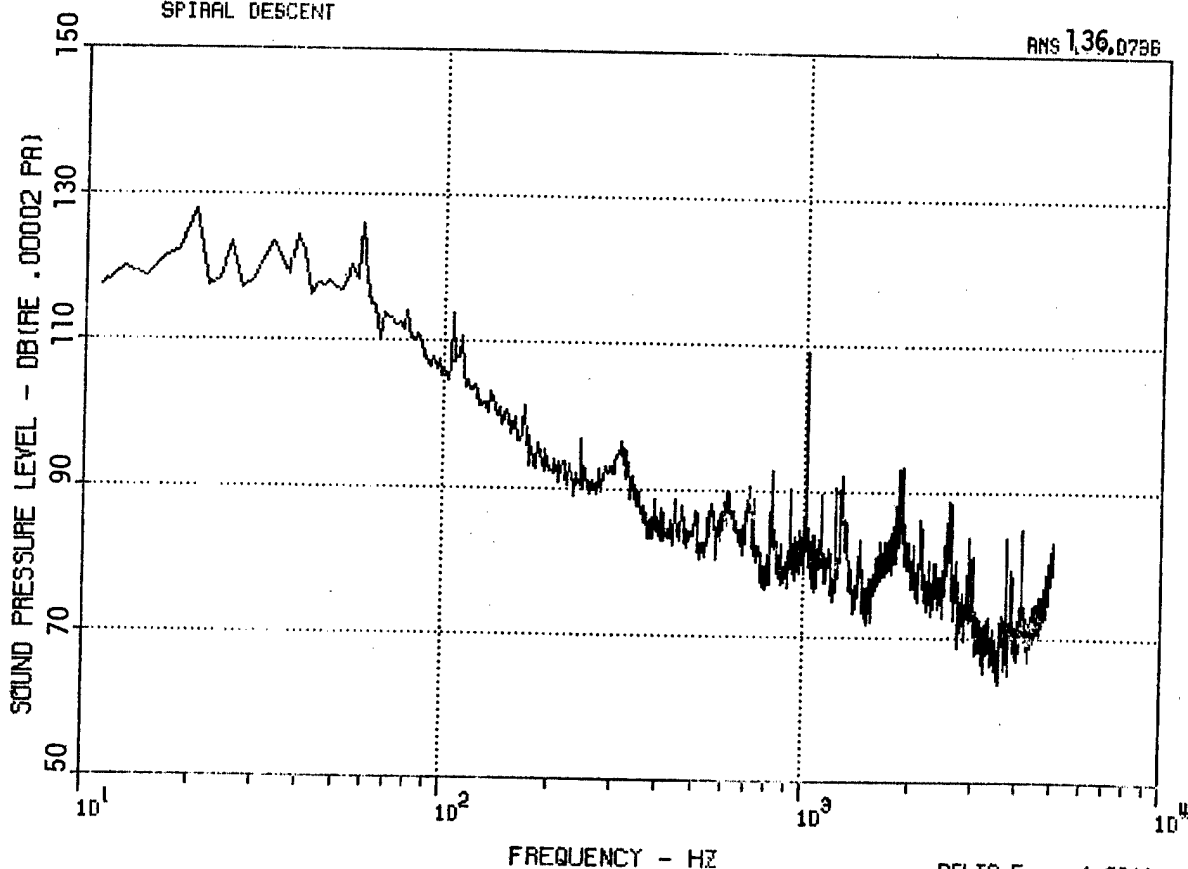
Figure 82. HH-53 Center Microphone MC, Cruise and Spiral Descent.
