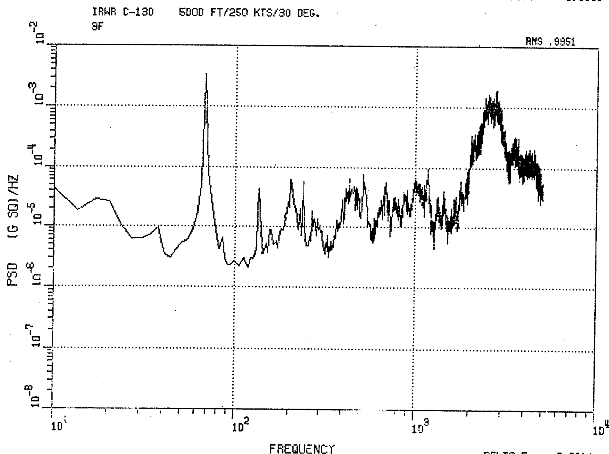
Figure 18. C-130 Fwd Vertical Accelerometer 3F, 1000 Ft, 250 Kt, 30 Deg, and 5000 Ft, 250 Kt, 30 Deg.
