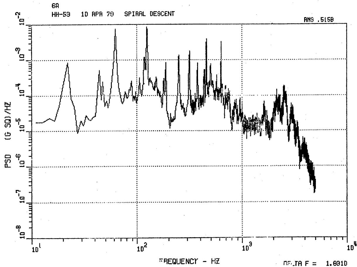
Figure 91. HH-53 Aft Longitudinal Accelerometer 6A, Cruise and Spiral Descent.
