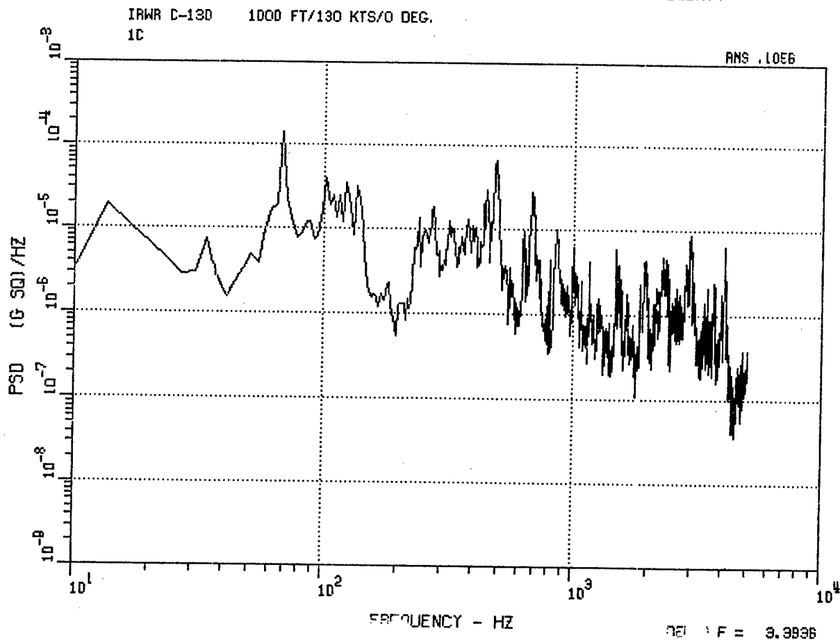
Figure 28. C-130 Center Vertical Accelerometer 1C, 200 Ft, 130 Kt, 0 Deg, and 1000 Ft, 130 Kt, 0 Deg.
