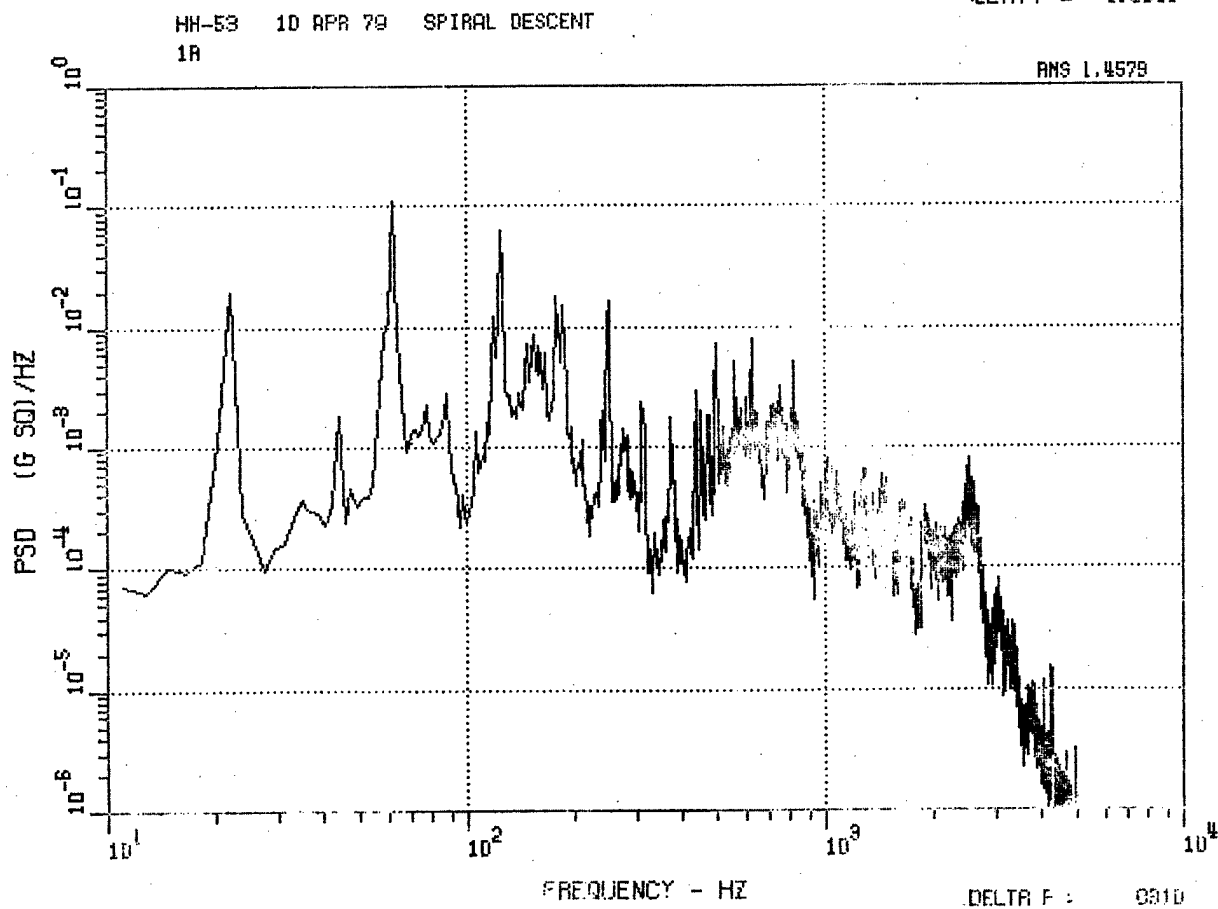
Figure 85. HH-53 Aft Lateral Accelerometer 1A, Cruise and Spiral Descent.
