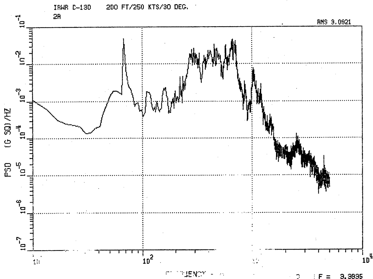
Figure 45. C-130 Aft Lateral Accelerometer 2A, 5000 Ft, 130 Kt, 0 Deg, and 200 Ft, 250 Kt, 30 Deg.
