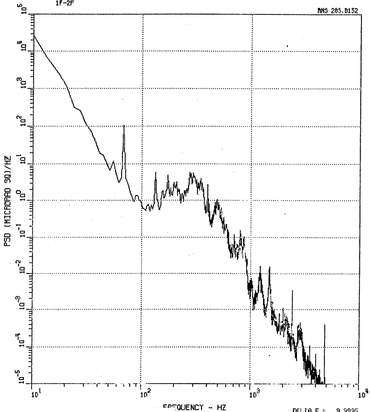
Figure 96. C-130 Fwd Roll PSD, 1F-2F, 1000 Ft, 250 Kt, 30 Deg.
