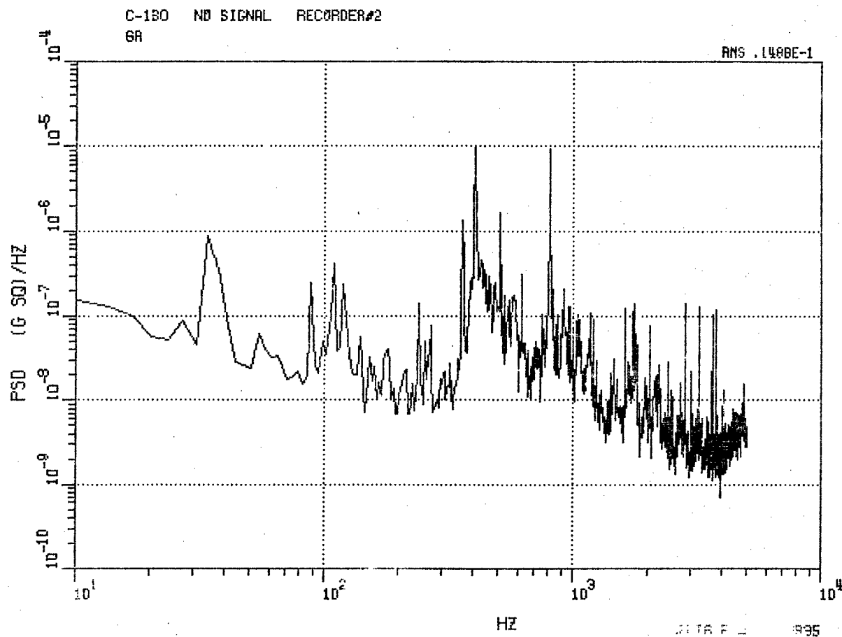
Figure 55. C-130 Aft Longitudinal Accelerometer 6A, No-Signal Record.
