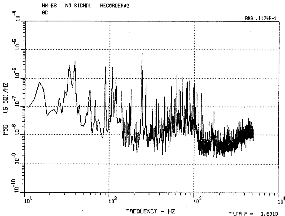
Figure 80. HH-53 Center Longitudinal Accelerometer 6C, Autorotation and No-Signal Record.
