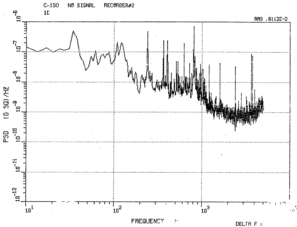
Figure 31. C-130 Center Vertical Accelerometer 1C, No-Signal Record.
