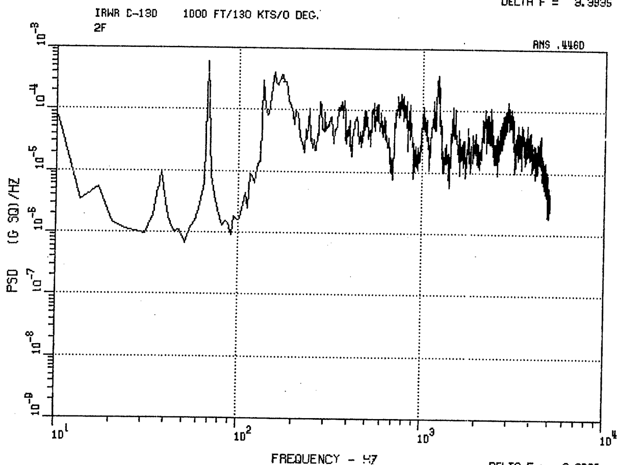
Figure 12. C-130 Fwd Lateral Accelerometer 2F, 200 Ft, 130 Kt, 0 Deg, and 1000 Ft, 130 Kt, 0 Deg.
