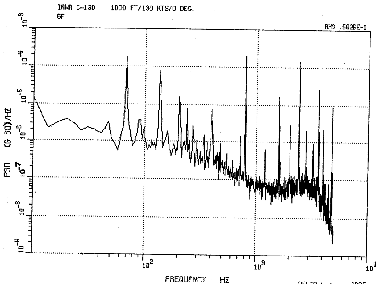
Figure 20. C-130 Fwd Longitudinal Accelerometer 6F, 200 Ft, 130 Kt, 0 Deg, and 1000 Ft, 130 Kt, 0 Deg.
