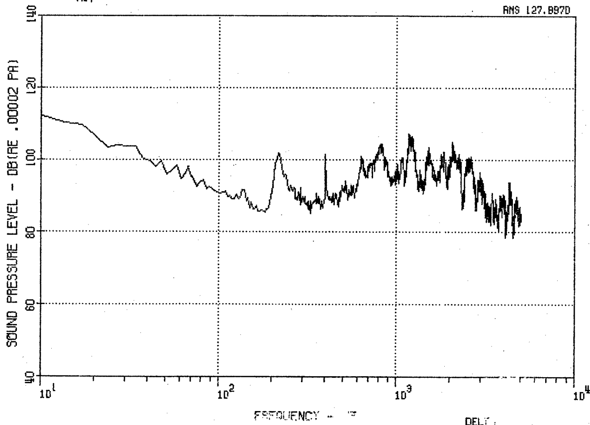
Figure 25. C-130 Fwd Microphone MF, 5000 Ft, 130 Kt, 0 Deg, and 200 Ft, 250 Kt, 30 Deg.
