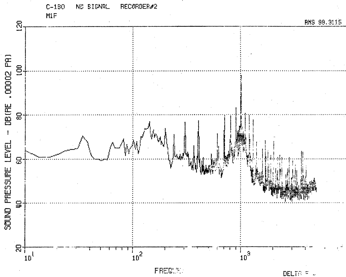
Figure 27. C-130 Fwd Microphone MF, No-Signal Record.
