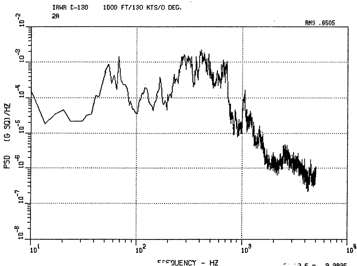
Figure 44. C-130 Aft Lateral Accelerometer 2A, 200 Ft, 130 Kt, 0 Deg, and 1000 Ft, 130 Kt, 0 Deg.
