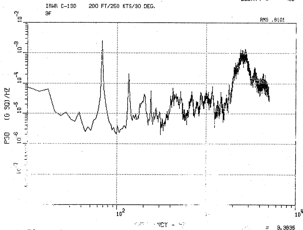
Figure 17. C-130 Fwd Vertical Accelerometer 3F, 5000 Ft, 130 Kt, 0 Deg, and 200 Ft, 250 Kt, 30 Deg.
