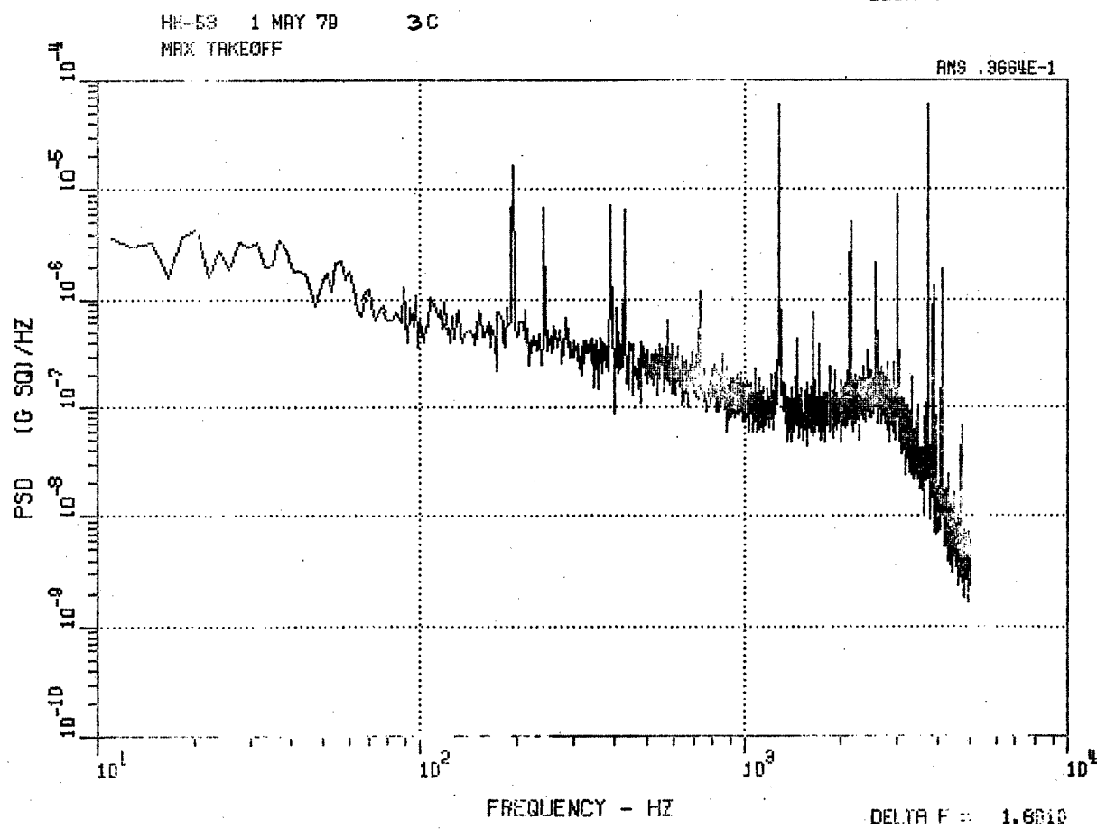
Figure 75. HH-53 Center Lateral Accelerometer 3C, Hover IGE and Max Takeoff.
