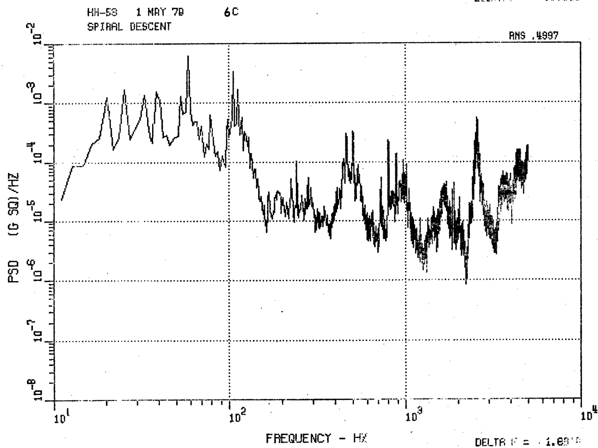
Figure 79. HH-53 Center Longitudinal Accelerometer 6C, Cruise and Spiral Descent.
