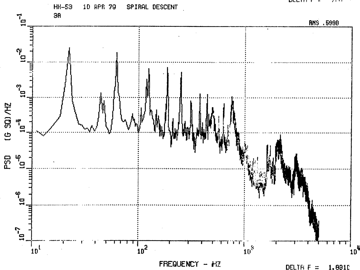
Figure 88. HH-53 Aft Vertical Accelerometer 3A, Cruise and Spiral Descent.
