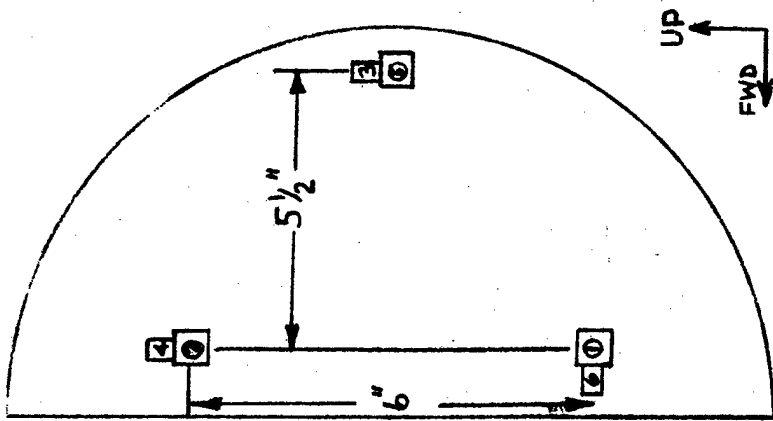
Aft Left AAR-43 Side View
