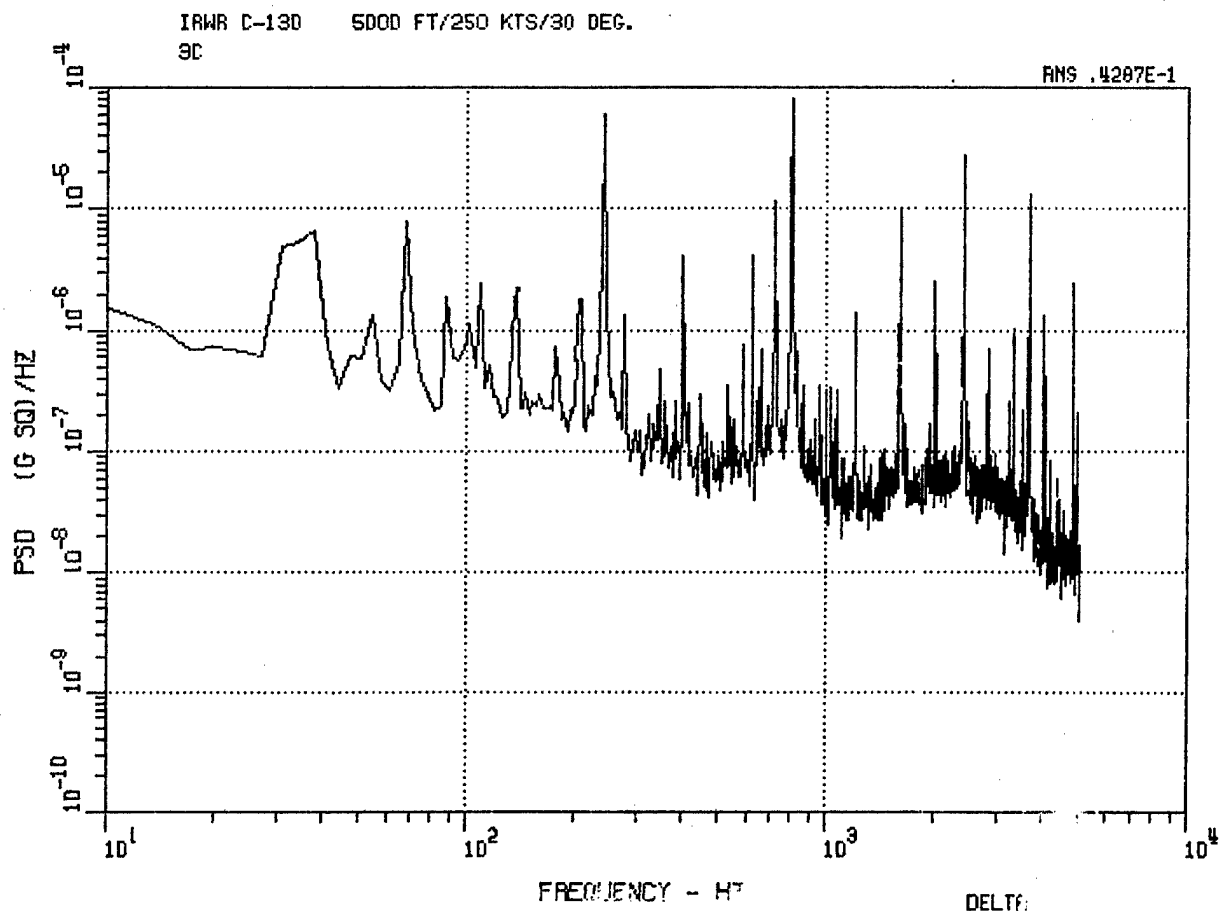
Figure 34. C-130 Center Lateral Accelerometer 3C, 1000 Ft, 250 Kt, 30 Deg, and 5000 Ft, 250 Kt, 30 Deg.
