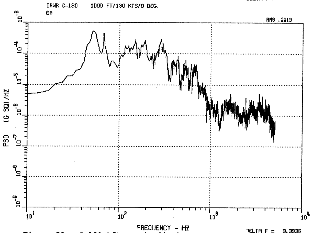
Figure 52. C-130 Aft Longitudinal Accelerometer 6A, 200 Ft, 130 Kt, 0 Deg, and 1000 Ft, 130 Kt, 0 Deg.
