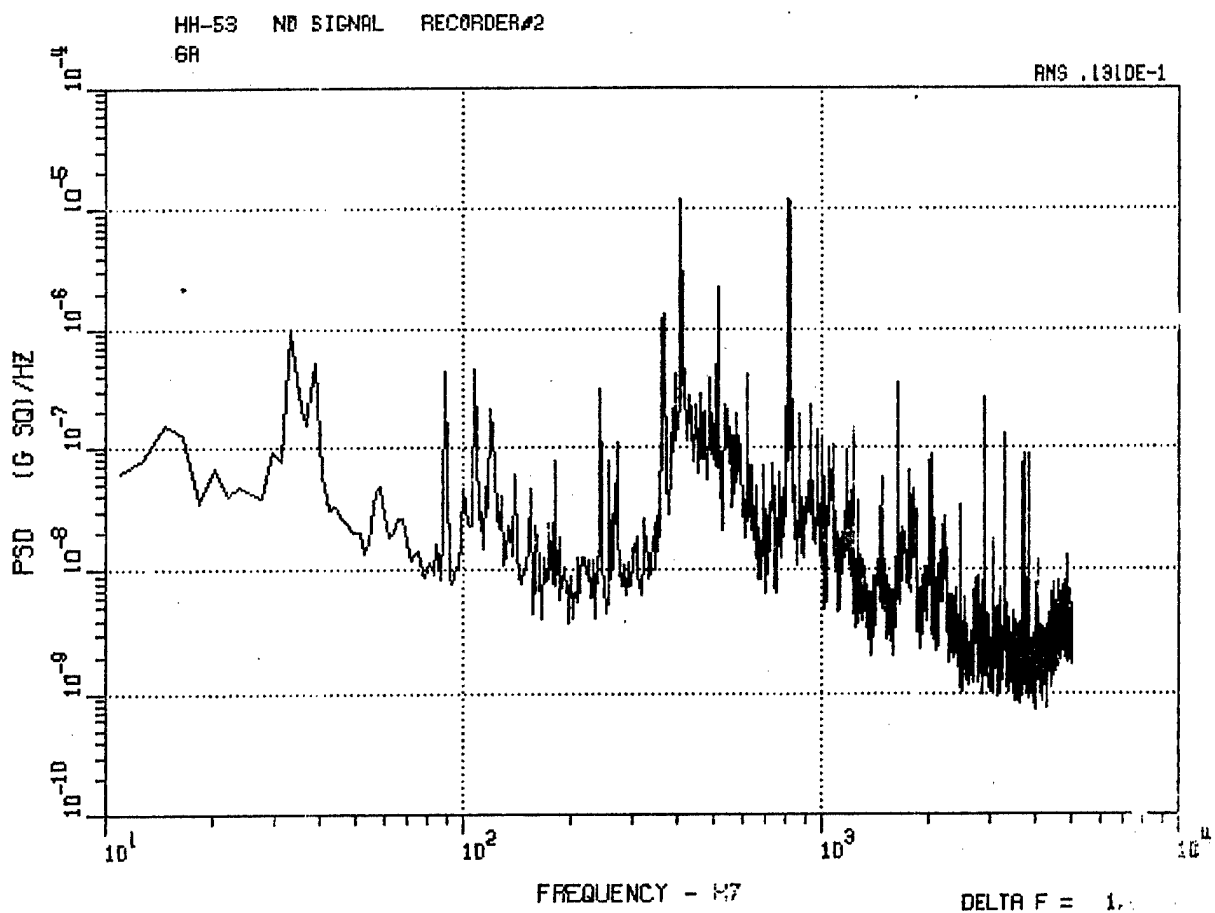
Figure 92. HH-53 Aft Longitudinal Accelerometer 6A, Autorotation and No-Signal Record.
