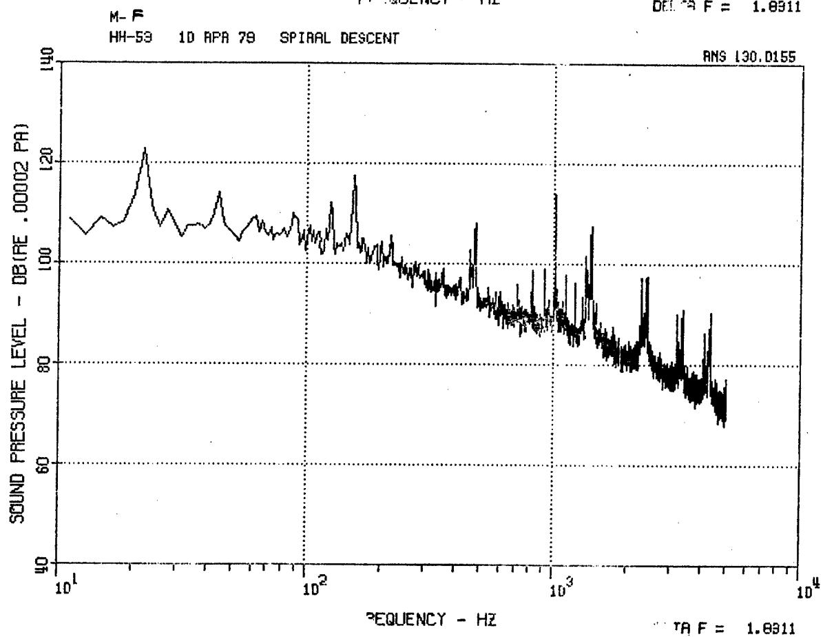
Figure 70. HH-53 Fwd Microphone MF, Cruise and Spiral Descent.
