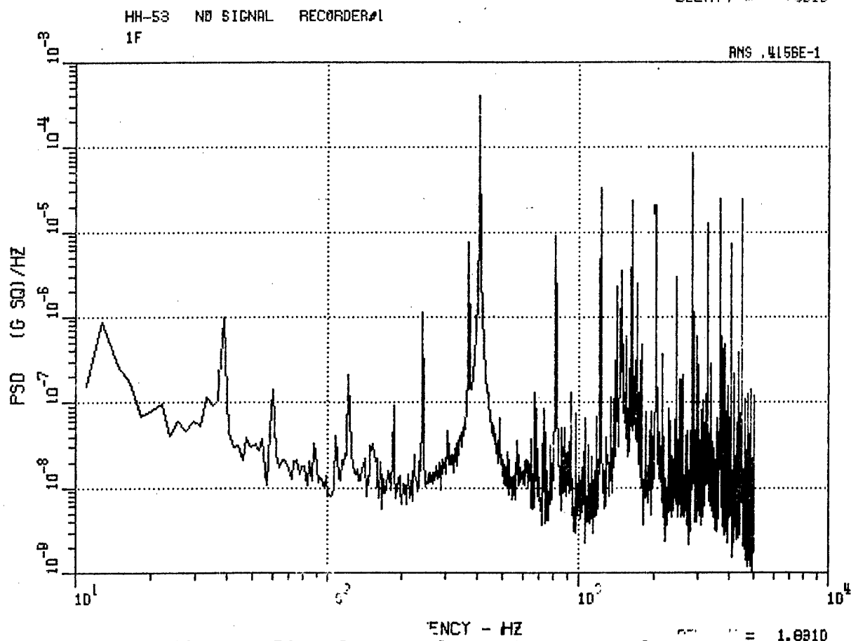
Figure 62. HH-53 Fwd Lateral Accelerometer 1F, Autorotation and No-Signal Record.
