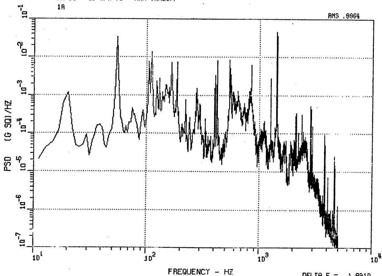
Figure 84. HH-53 Aft Lateral Accelerometer 1A, Hover IGE and Max Takeoff.
