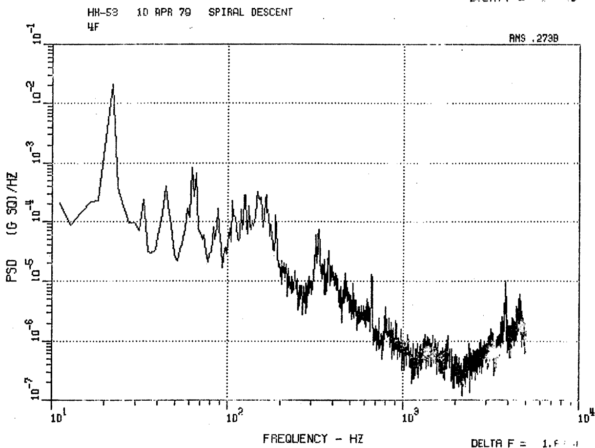
Figure 64. HH-53 Fwd Vertical Accelerometer 4F, Cruise and Spiral Descent.
