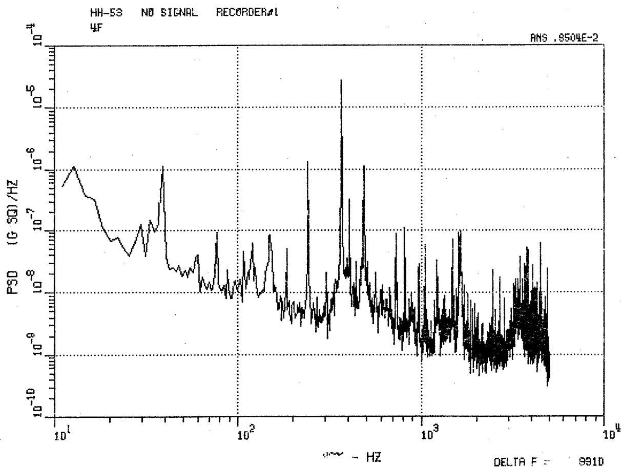
Figure 65. HH-53 Fwd Vertical Accelerometer 4F, Autorotation and No-Signal Record.
