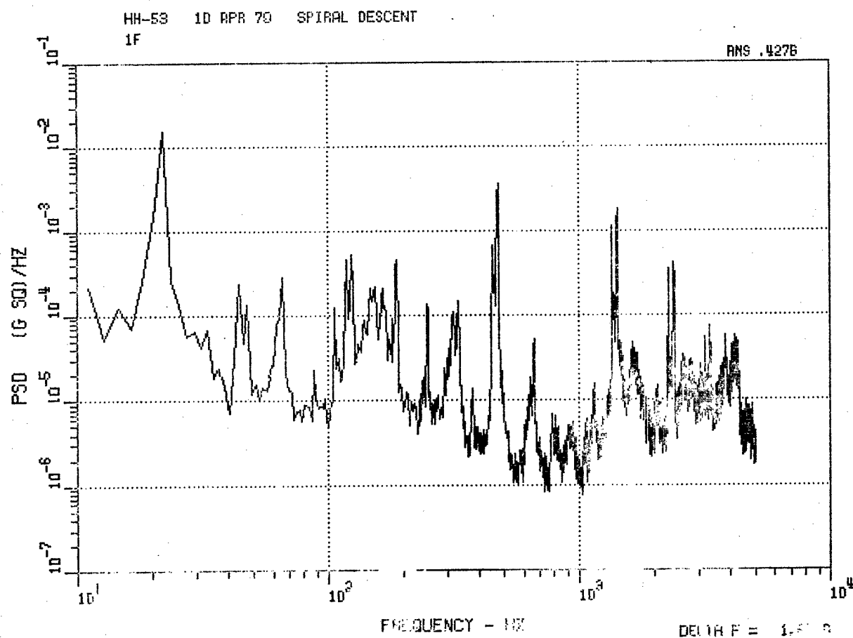
Figure 61. HH-53 Fwd Lateral Accelerometer 1F, Cruise and Spiral Descent.
