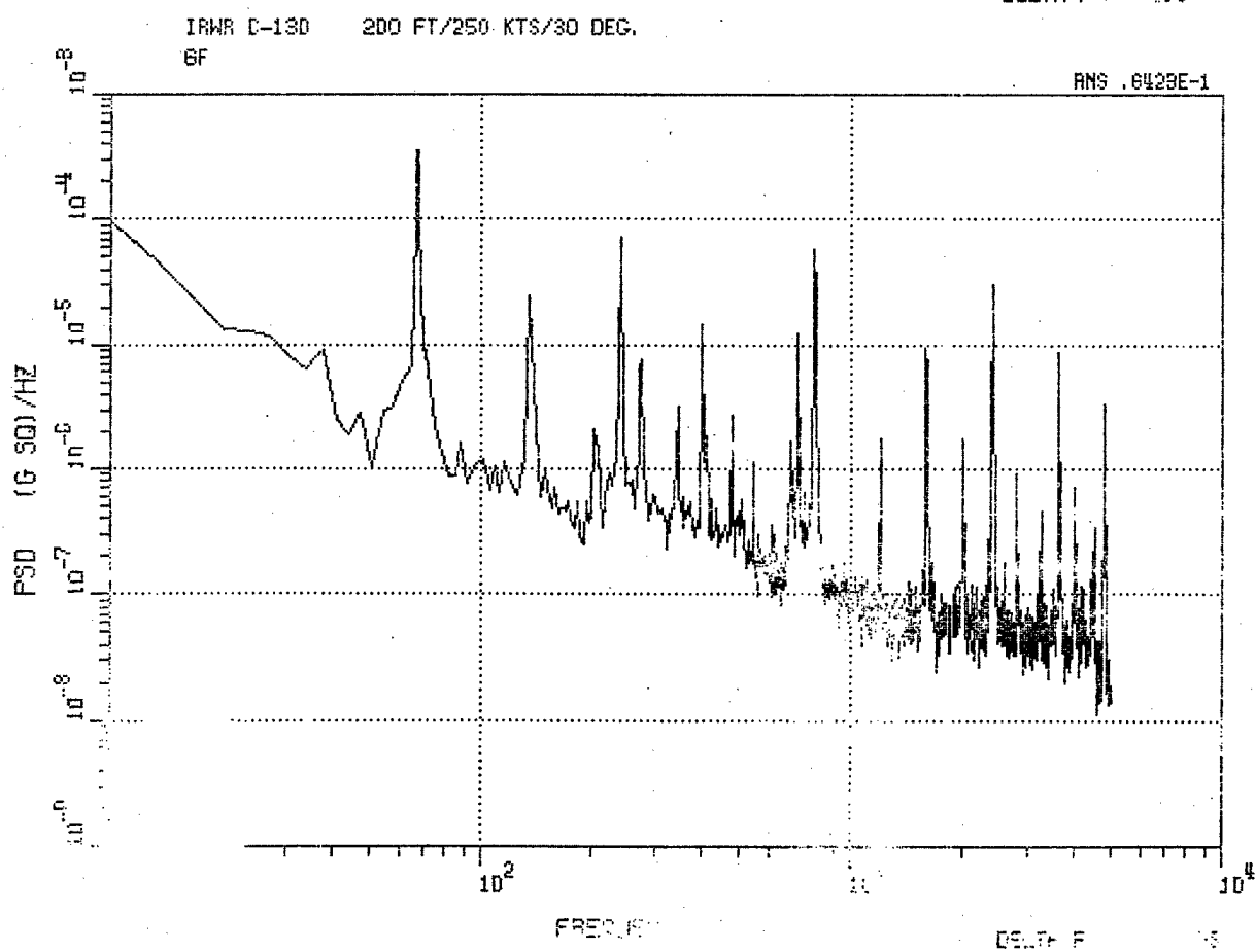
Figure 21. C-130 Fwd Longitudinal Accelerometer 6F, 5000 Ft, 130 Kt, 0 Deg, and 200 Ft, 250 Kt, 30 Deg.
