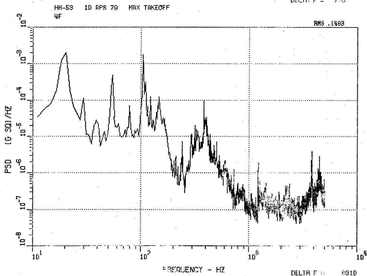
Figure 63. HH-53 Fwd Vertical Accelerometer 4F, Hover IGE and Max Takeoff.
