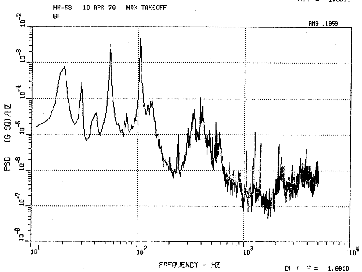
Figure 66. HH-53 Fwd Longitudinal Accelerometer 6F, Hover IGE and Max Takeoff.
