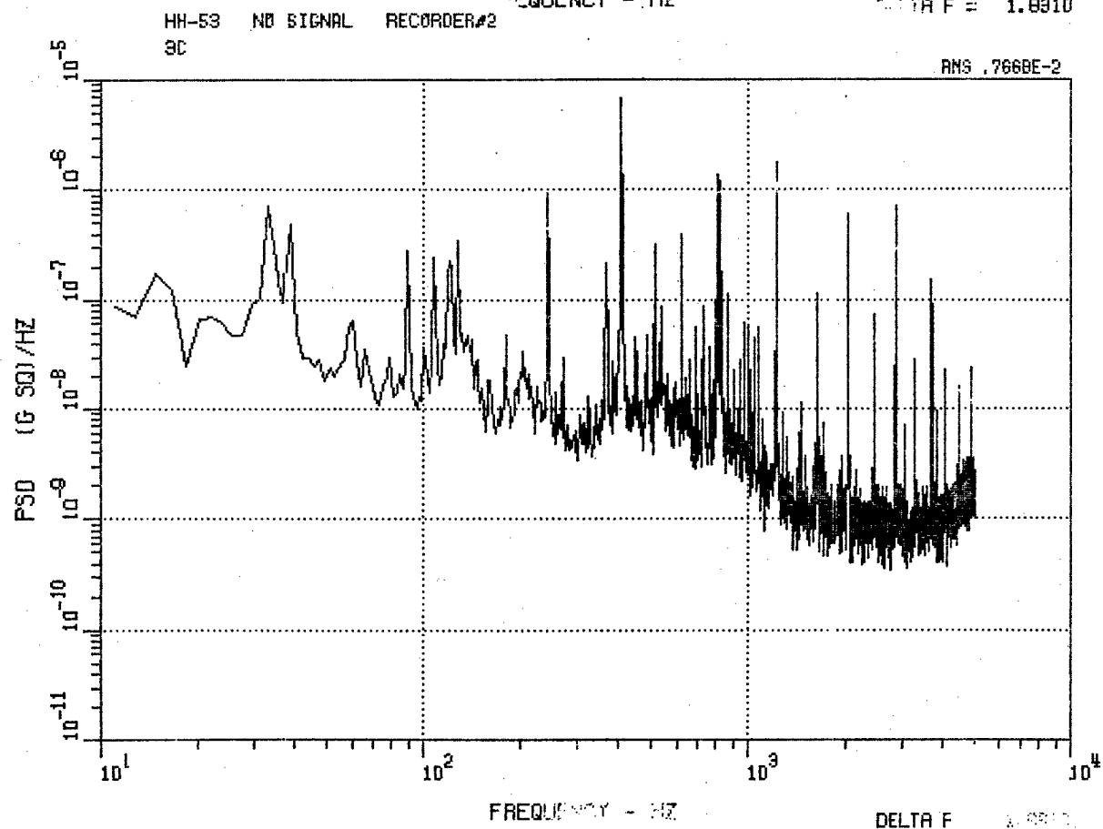
Figure 77. HH-53 Center Lateral Accelerometer 3C, Autorotation and No-Signal Record.
