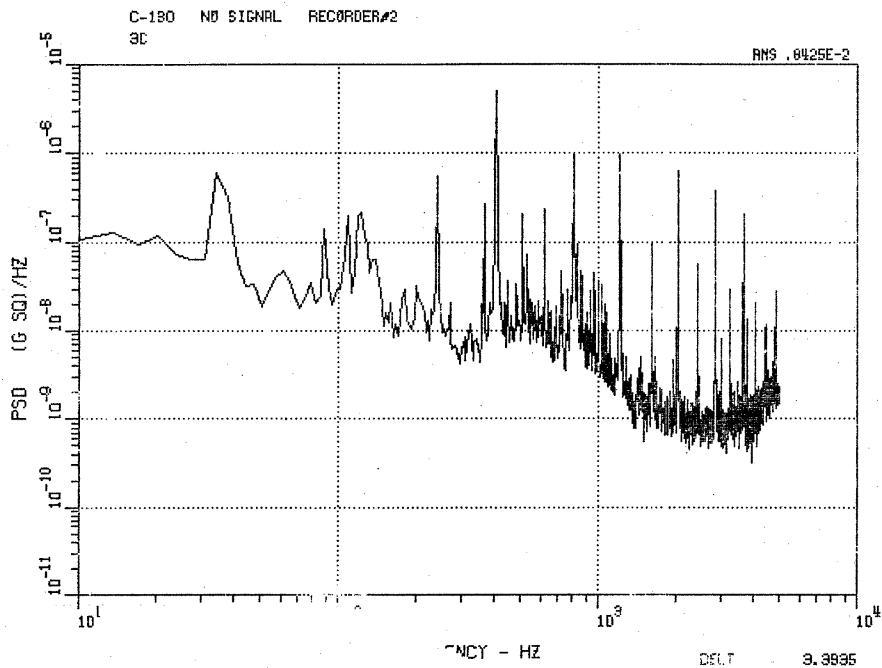
Figure 35. C-130 Center Lateral Accelerometer 3C, No-Signal Record.
