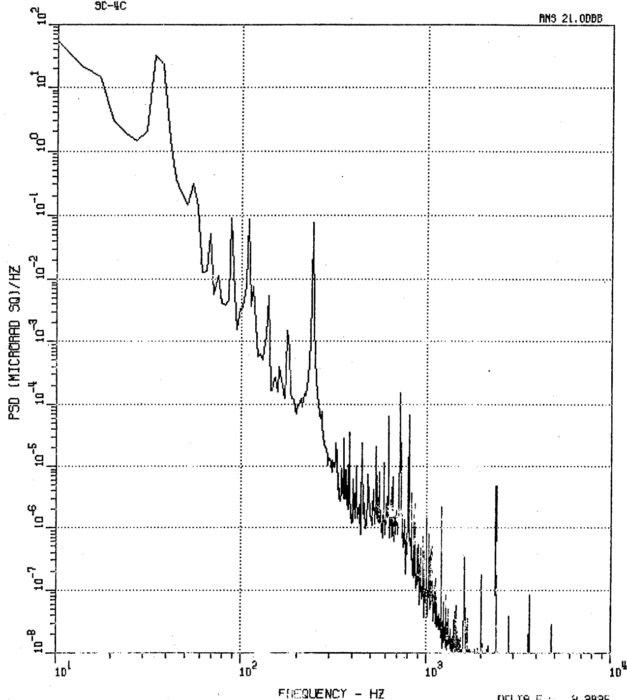
Figure 98. C-130 Center Yaw PSD; 3C-4C, 1000 Ft, 250 Kt, 30 Deg.
