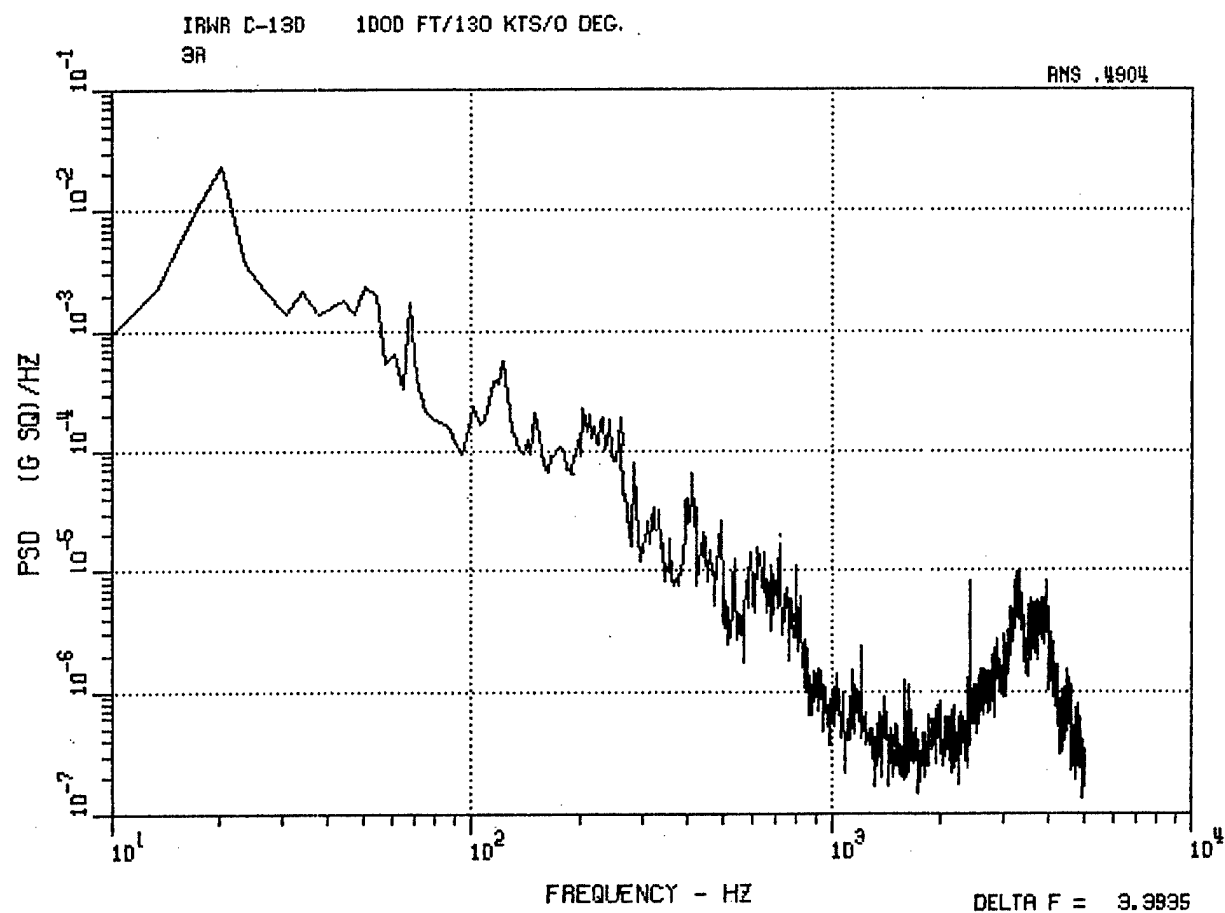
Figure 48. C-130 Aft Vertical Accelerometer 3A, 200 Ft, 130 Kt, 0 Deg, and 1000 Ft, 130 Kt, 0 Deg.
