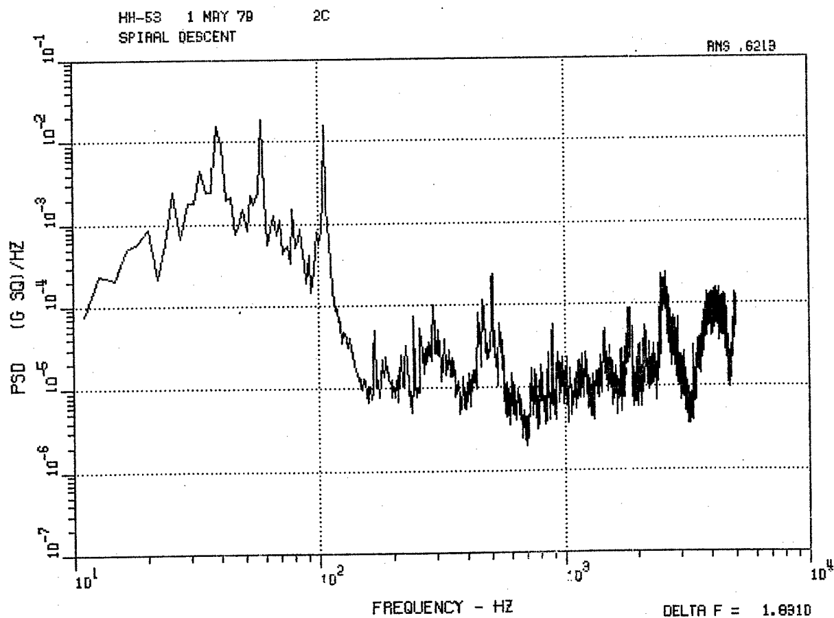
Figure 73. HH-53 Center Vertical Accelerometer 2C, Cruise and Spiral Descent.
