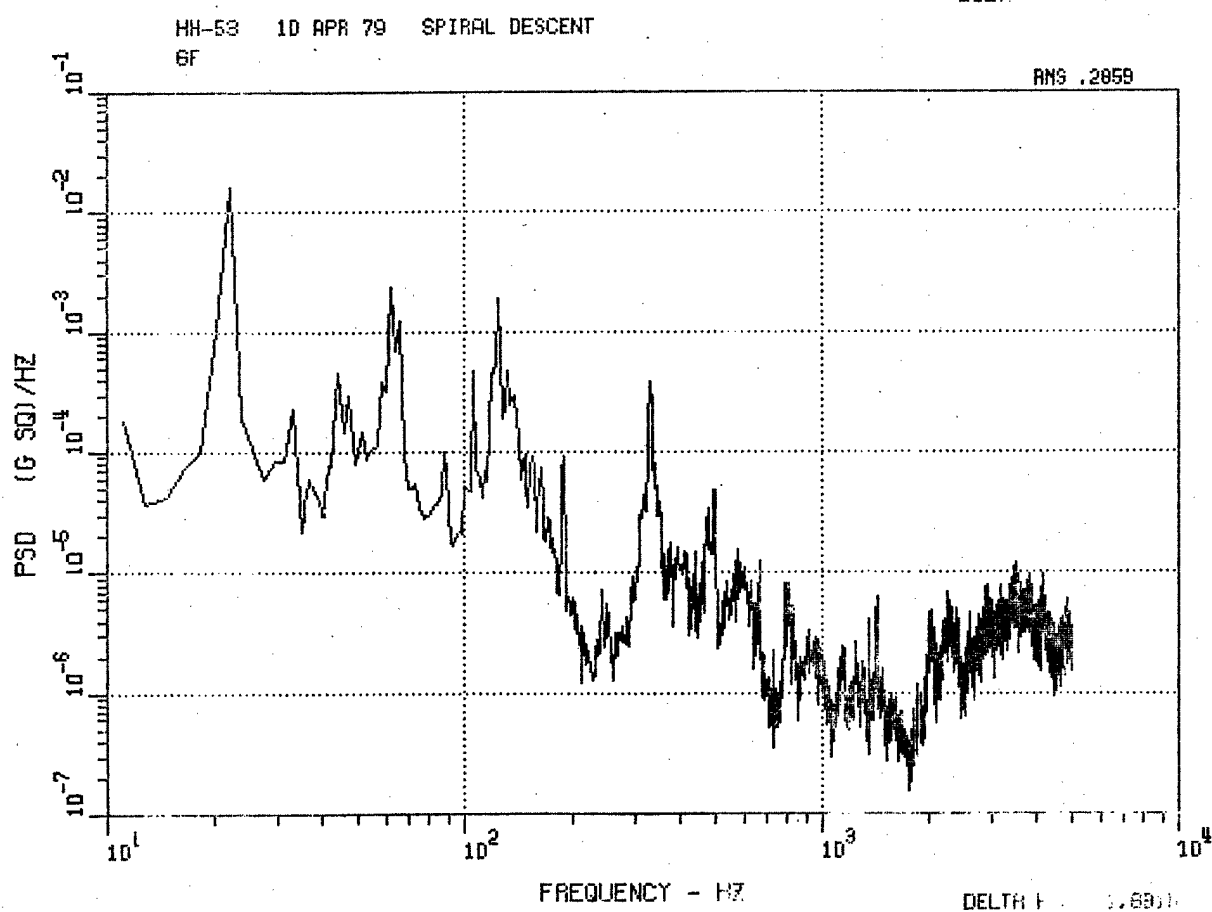
Figure 67. HH-53 Fwd Longitudinal Accelerometer 6F, Cruise and Spiral Descent.
