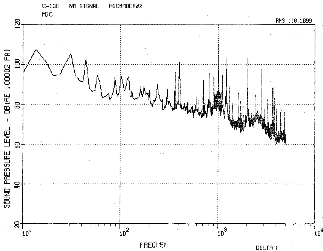
Figure 43. C-130 Center Microphone MC, No-Signal Record.
