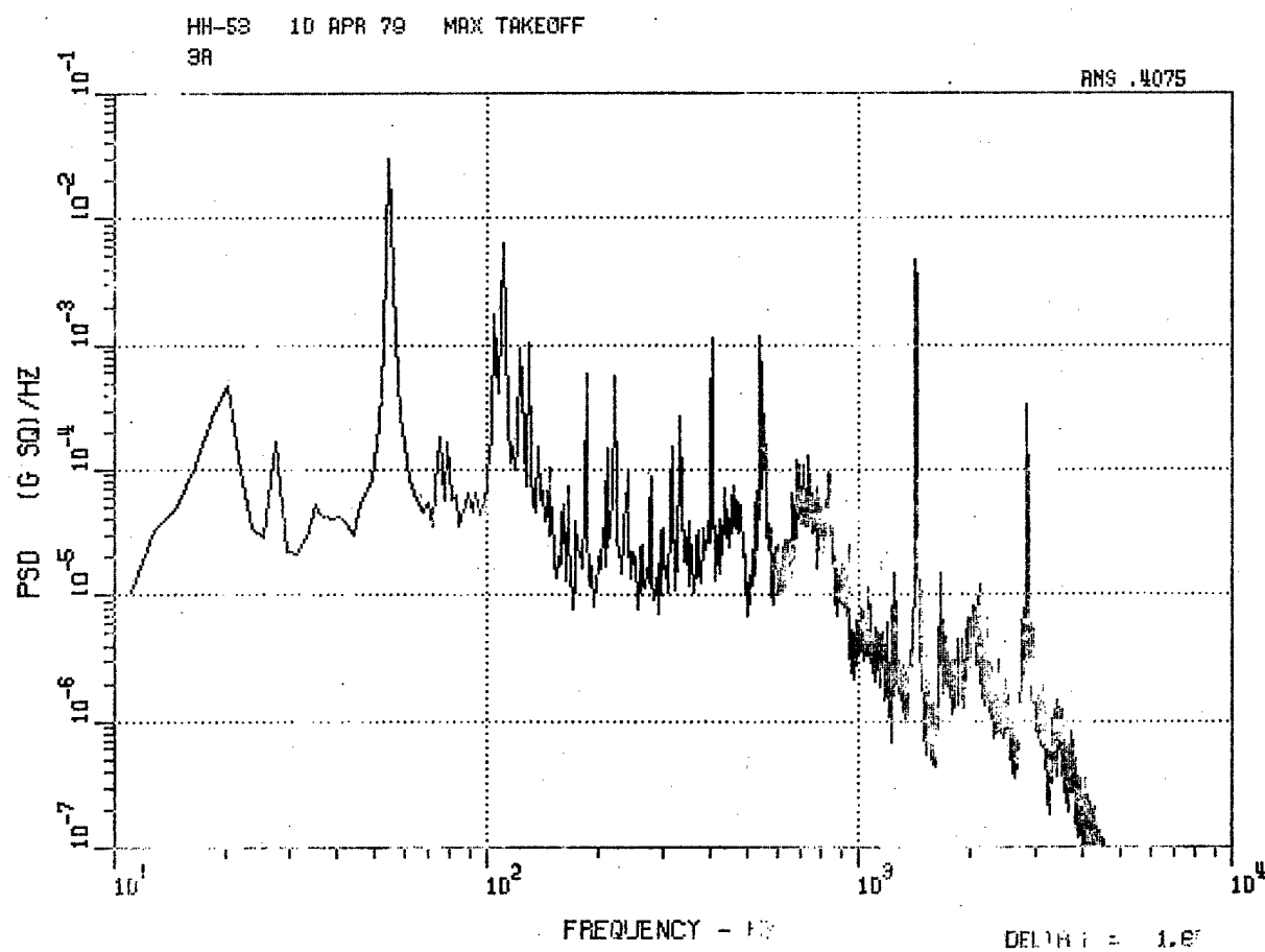
Figure 87. HH-53 Aft Vertical Accelerometer 3A, Hover IGE and Max Takeoff.
