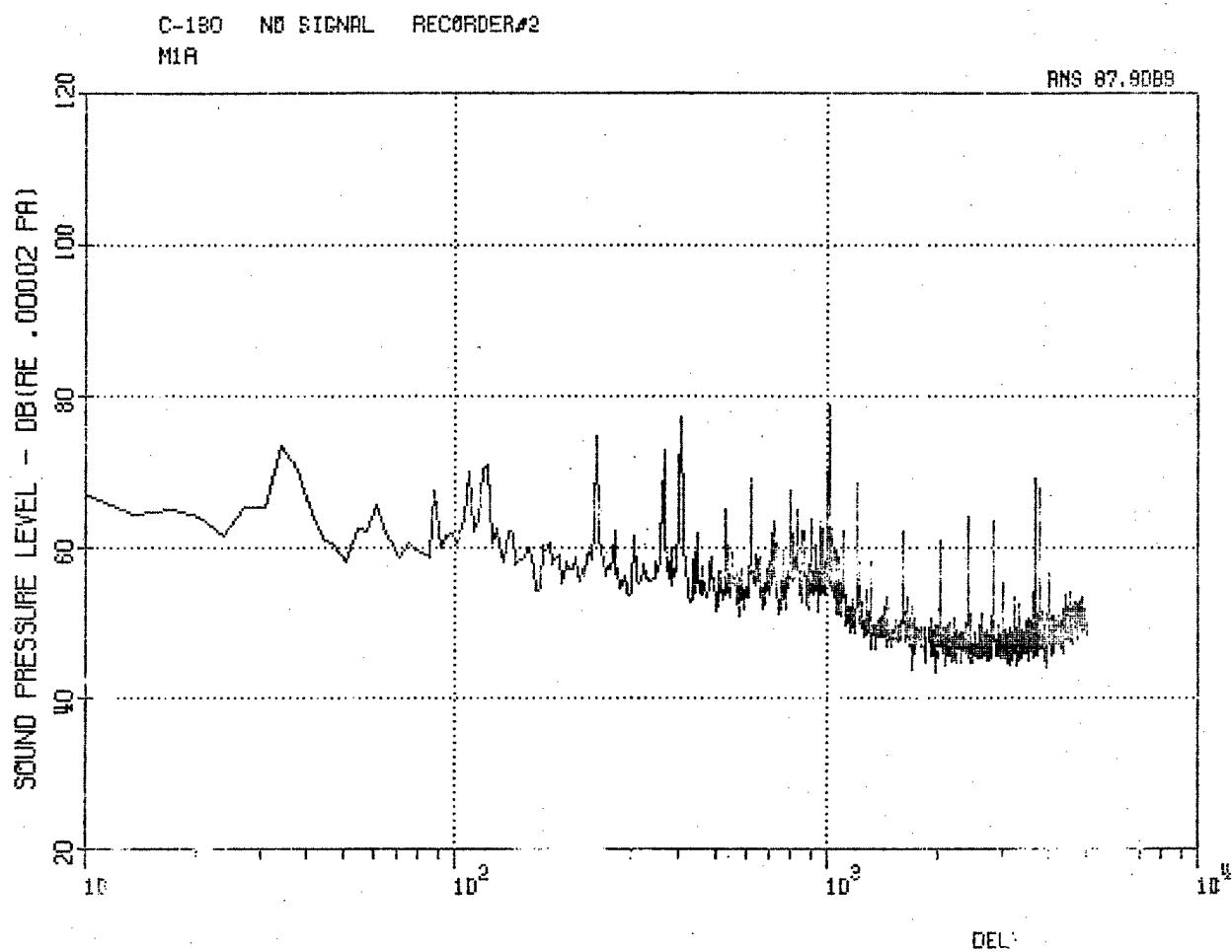
Figure 59. C-130 Aft Microphone MA, No-Signal Record.
