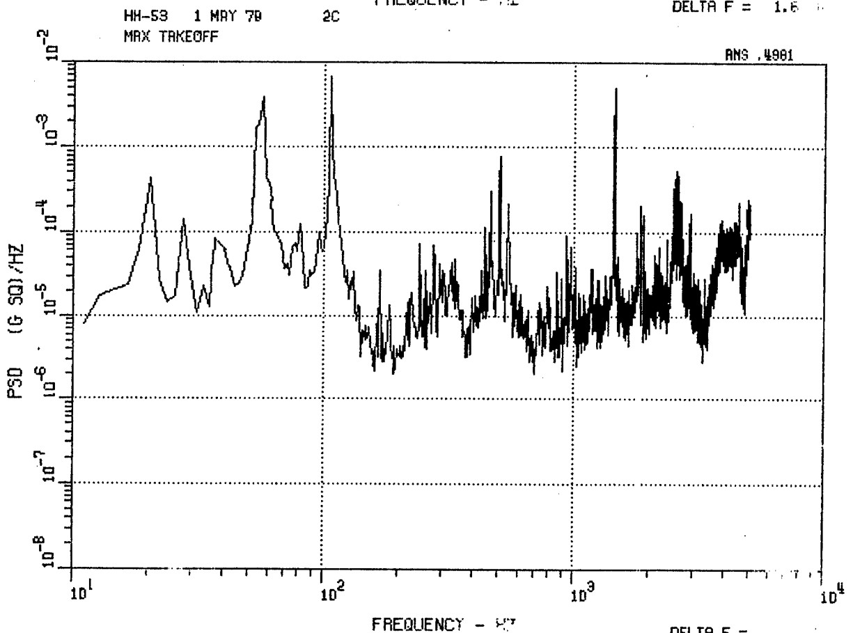
Figure 72. HH-53 Center Vertical Accelerometer 2C, Hover IGE and Max Takeoff.
