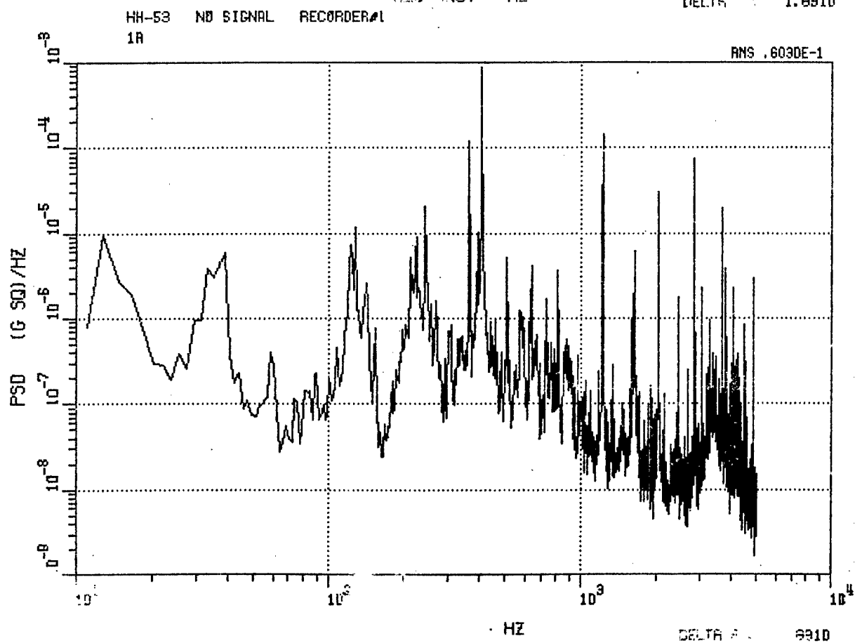
Figure 86. HH-53 Aft Lateral Accelerometer 1A, Autorotation and No-Signal Record.
