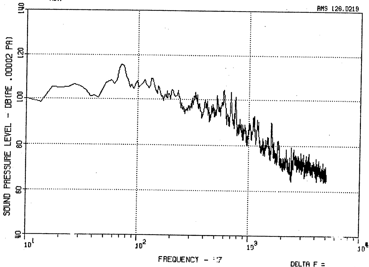
Figure 58. C-130 Aft Microphone MA, 1000 Ft, 250 Kt, 30 Deg, and 5000 Ft, 250 Kt, 30 Deg.
