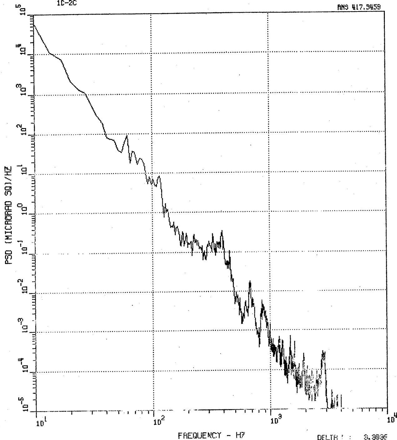
Figure 97. C-130 Center Roll PSD, 1C-2C, 1000 Ft, 250 Kt, 30 Deg.
