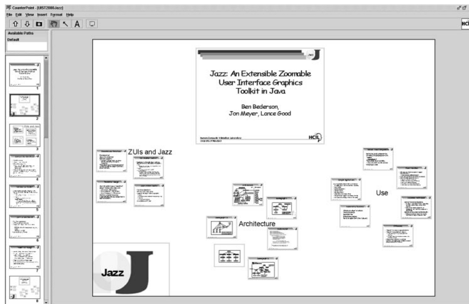
Figure 4 A screen shot of CounterPoint in spatial arrangement mode. The panel on the right, the 'Editing Canvas', is used to modify the positions and magnifications of pre-authored slides. The panel on the left is used to edit paths through the presentation.
