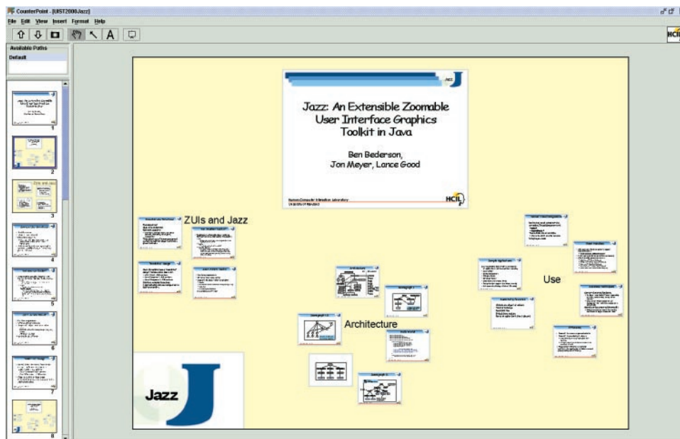
Figure 3 A screen shot of CounterPoint in spatial arrangement mode. The panel on the right, the 'Editing Canvas', is used to modify the positions and magnifications of pre-authored slides. The panel on the left is used to edit paths through the presentation.
