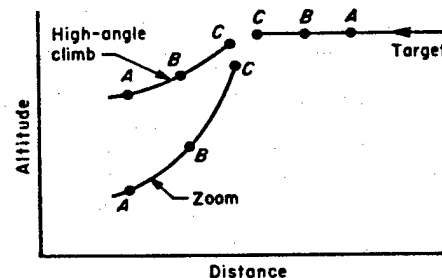
Fig. 45—"Zoom" and "high-angle" climbs
