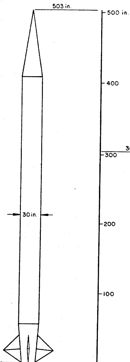
Fig. 62—Advanced generalized local-defense missile (semi-active homing-all-the-way)
