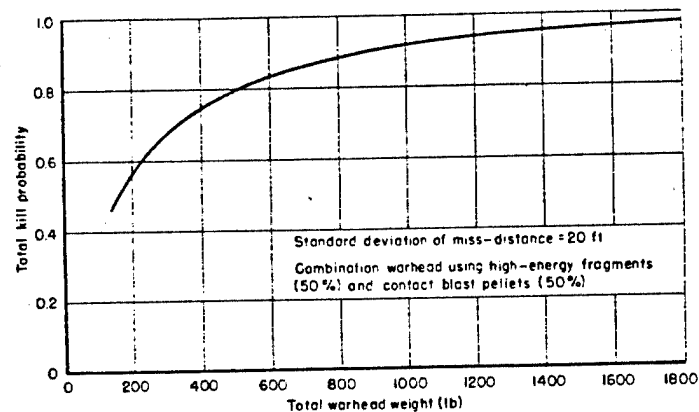
Fig. 59—K-kill probability on aircraft and missiles for dual-purpose warhead
