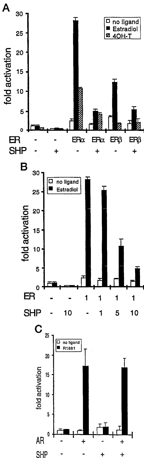
Fig. 4. Specific Inhibition of ER \alpha by SHP A, Inhibition of transactivation by ER with SHP. Plasmids containing human ER \alpha and rat ER \beta 1 in pCDNA3 vector (25 ng/well) and SHP in CDM8 vector (250 ng/well) were cotransfected with TK \beta -gal (125 ng/well) and ERETkluciferase (250 ng/well), a luciferase reporter plasmid containing three copies
